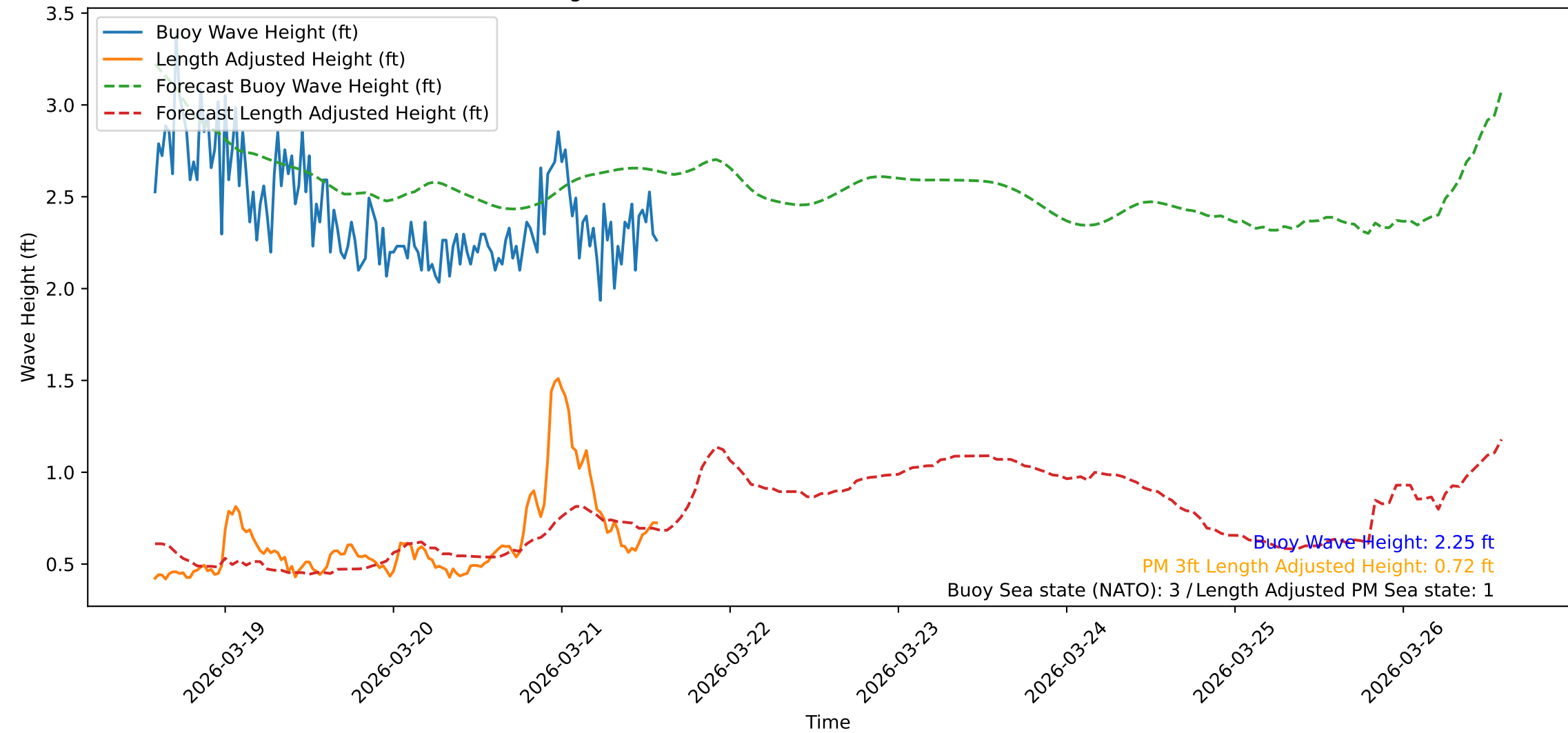
Wave Heights over Time for Green Beach at 2026-03-21 14:11:11
