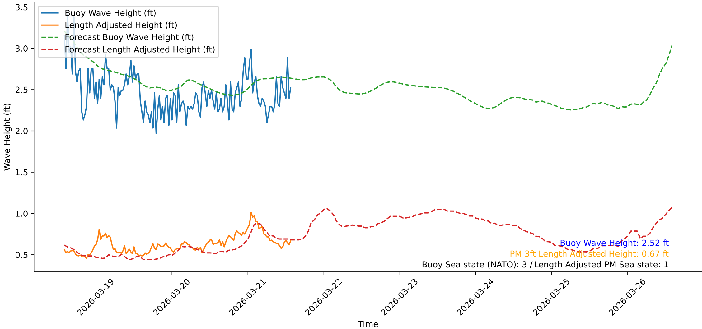
Wave Heights over Time for Oceanside Harbor at 2026-03-21 14:10:32
