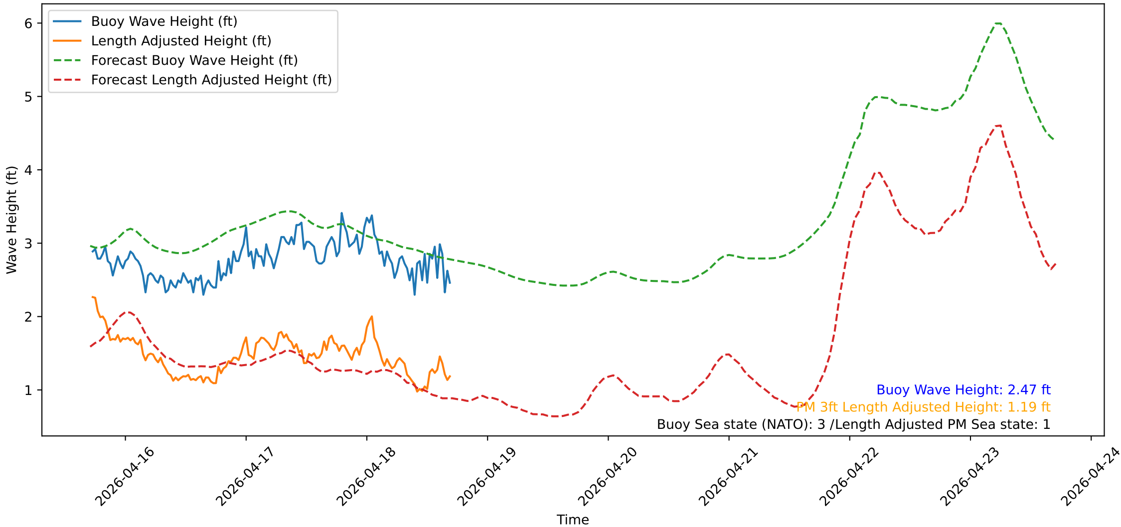
Wave Heights over Time for Oceanside Harbor at 2026-04-18 17:20:31
