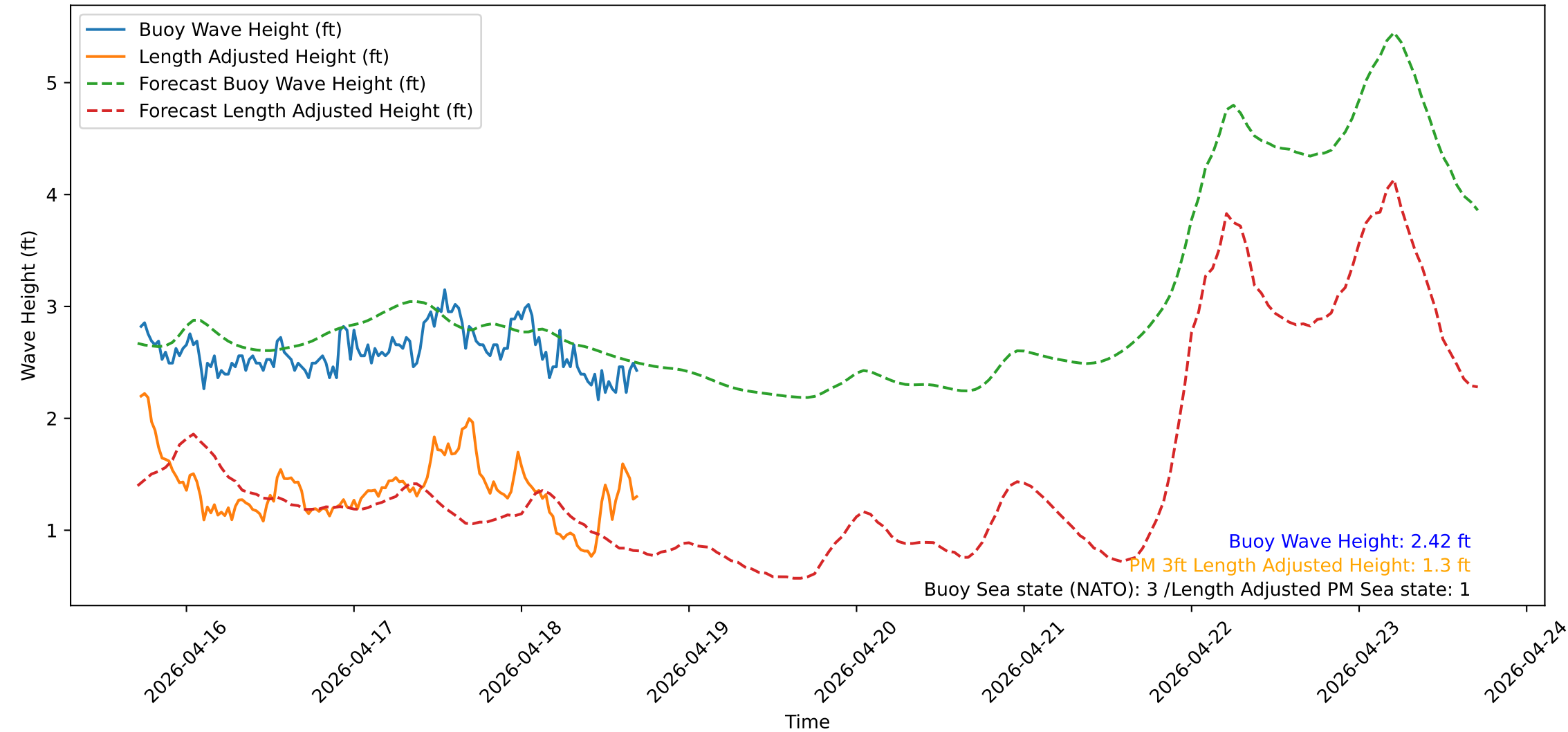
Wave Heights over Time for Red Beach at 2026-04-18 17:20:52
