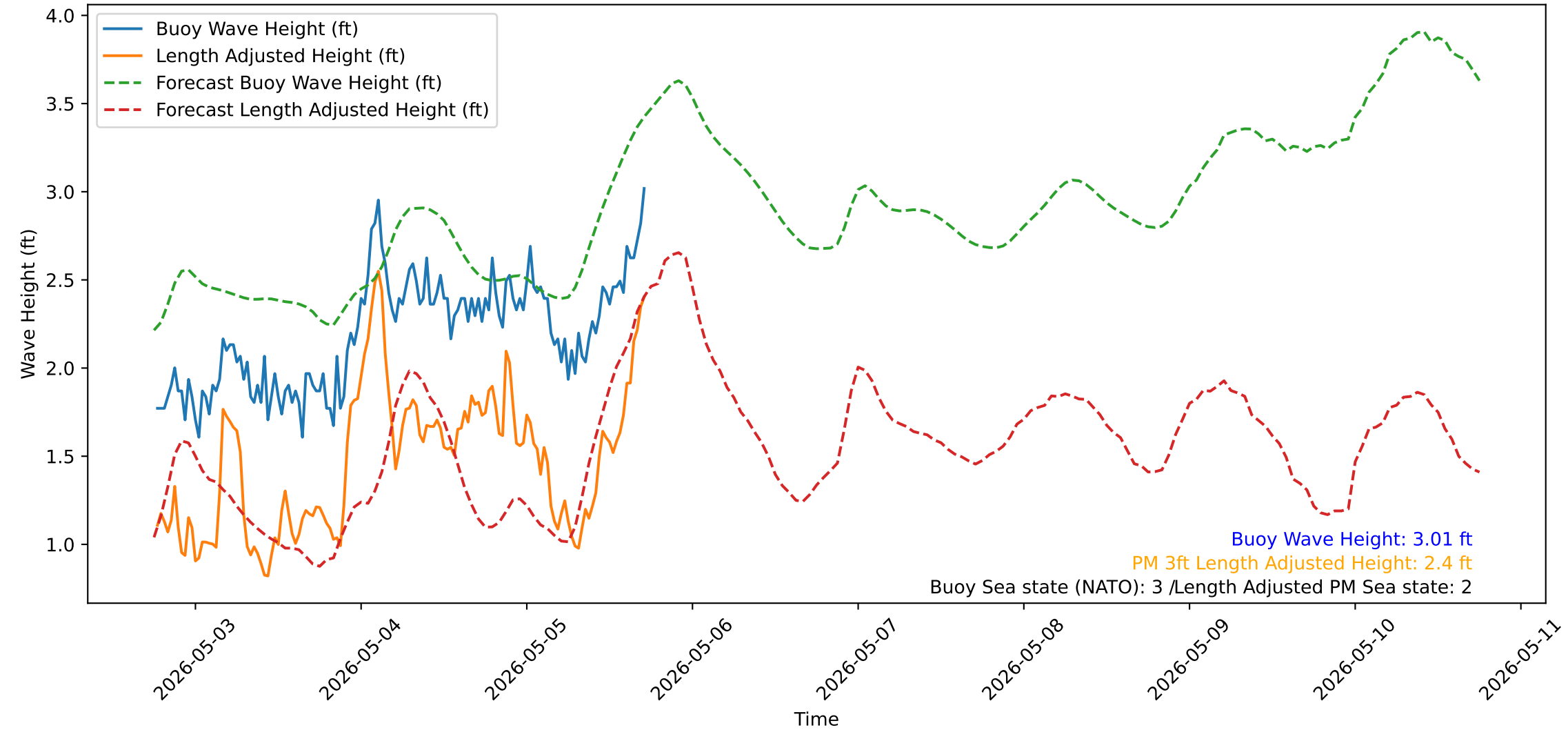
Wave Heights over Time for Red Beach at 2026-05-05 18:00:51
