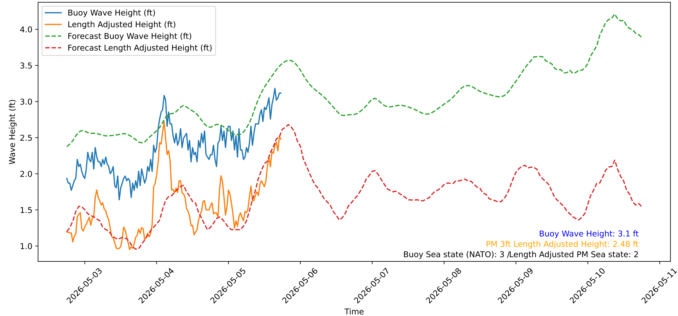
Wave Heights over Time for Oceanside Harbor at 2026-05-05 18:00:32
