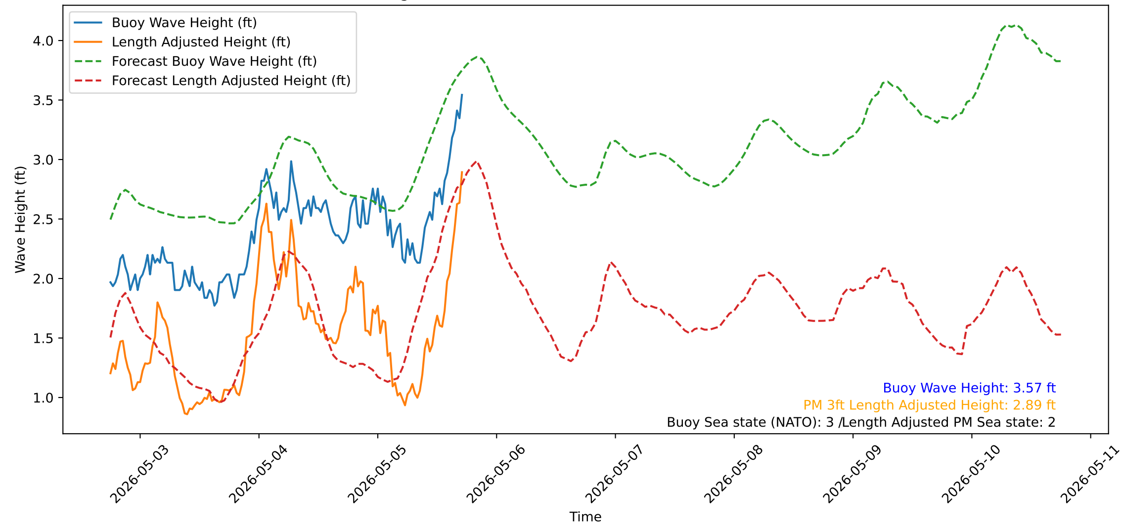
Wave Heights over Time for Green Beach at 2026-05-05 18:01:14
