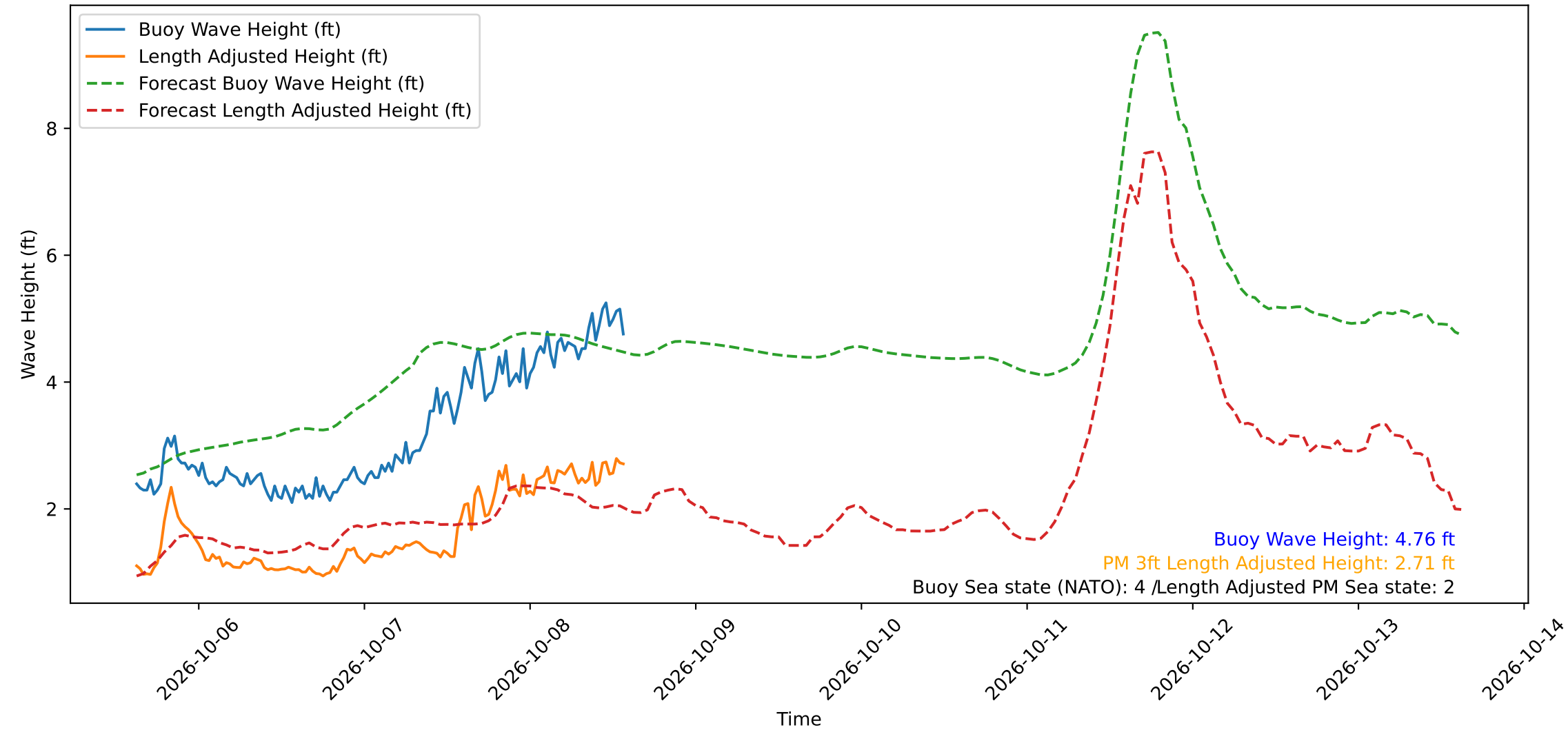
Wave Heights over Time for Green Beach at 2026-10-08 14:31:12
