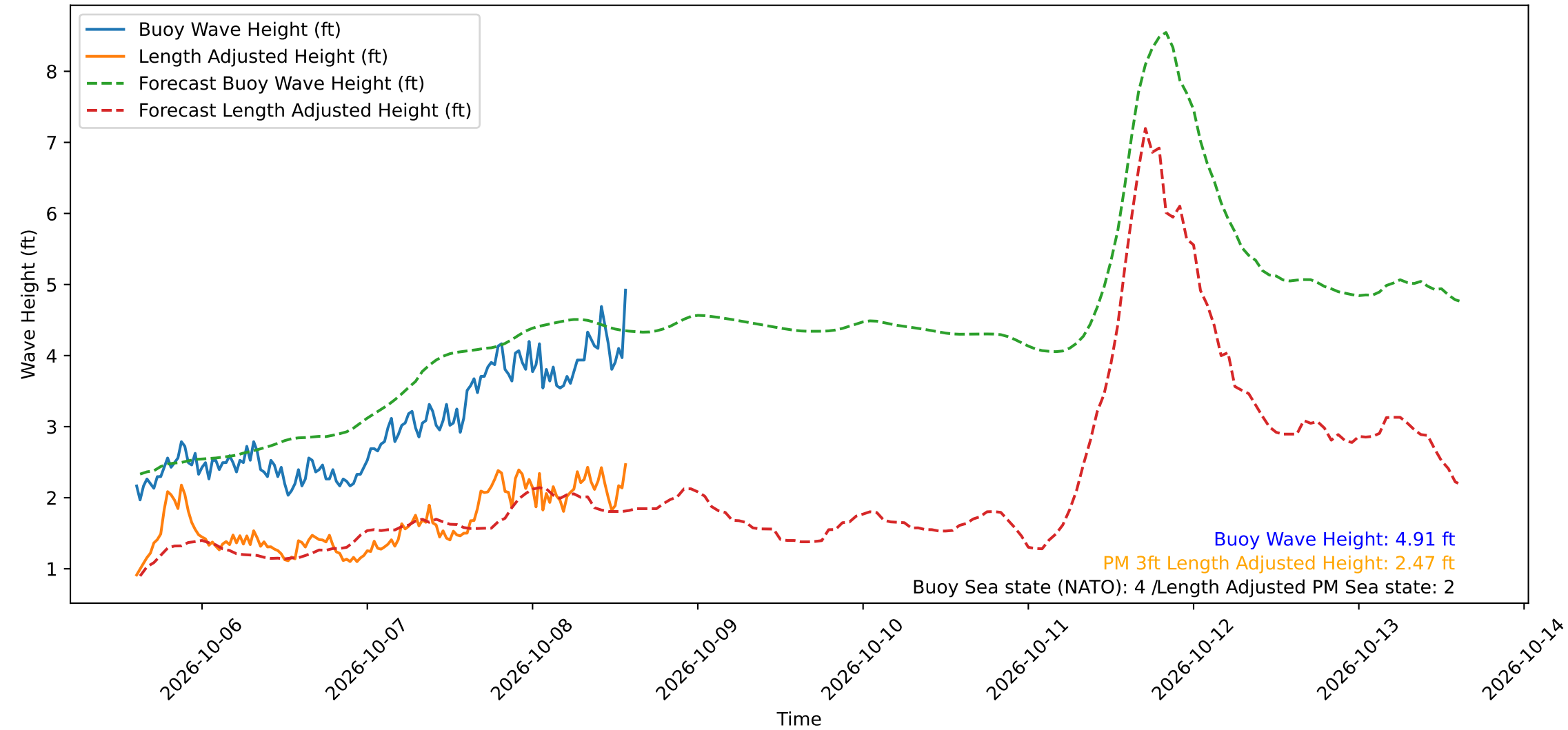
Wave Heights over Time for Oceanside Harbor at 2026-10-08 14:30:30
