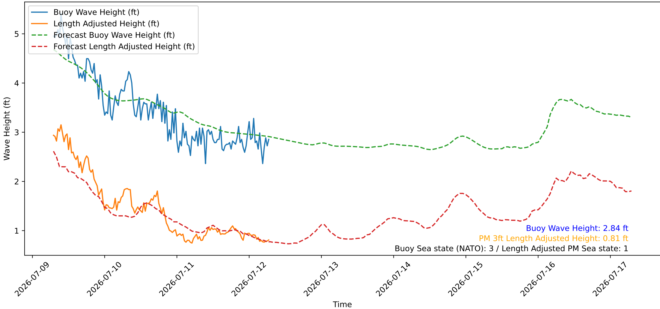
Wave Heights over Time for Oceanside Harbor at 2026-07-12 07:10:27
