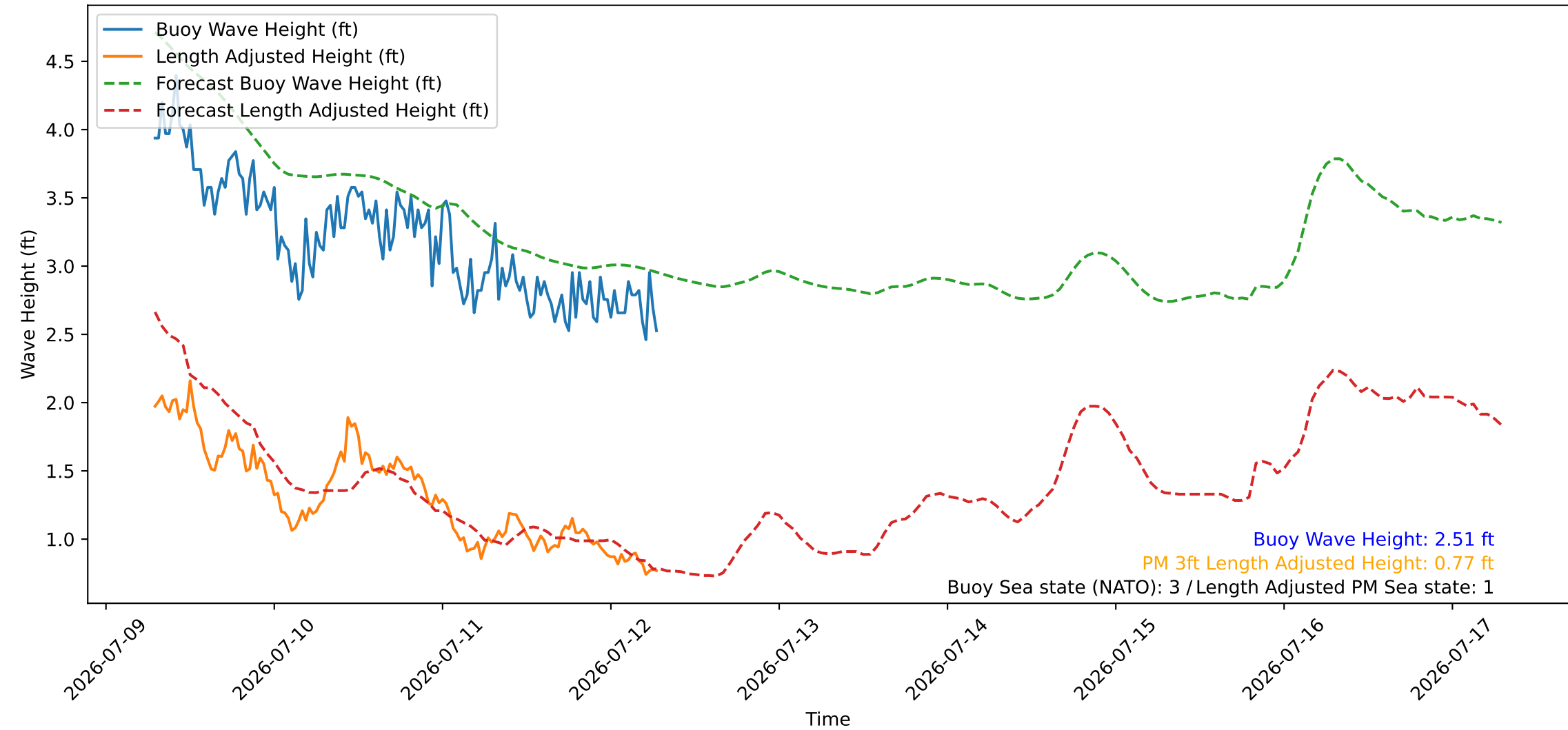
Wave Heights over Time for Green Beach at 2026-07-12 07:11:09
