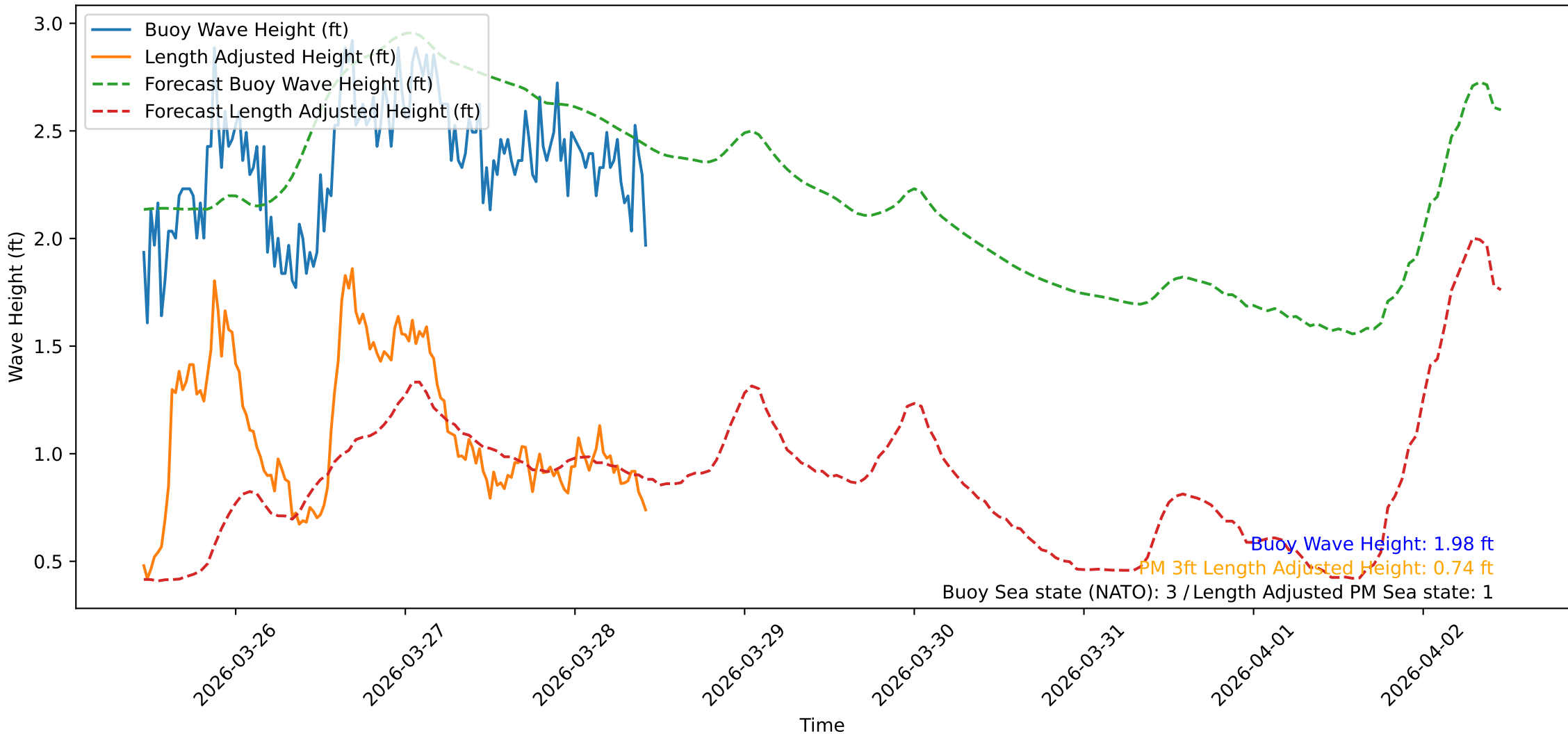
Wave Heights over Time for Oceanside Harbor at 2026-03-28 11:10:31
