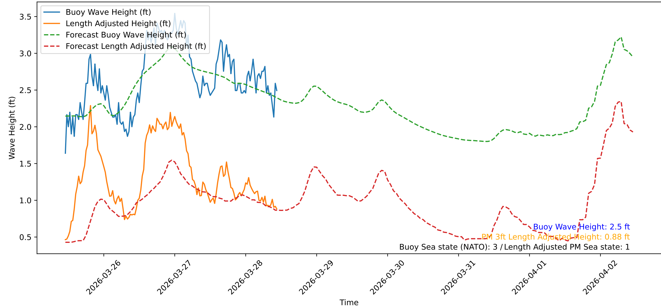
Wave Heights over Time for Green Beach at 2026-03-28 11:11:09
