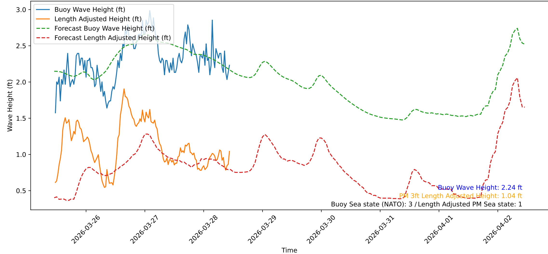
Wave Heights over Time for Red Beach at 2026-03-28 11:10:46
