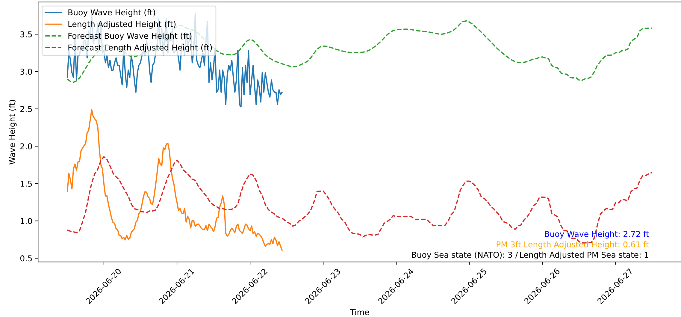
Wave Heights over Time for Red Beach at 2026-06-22 11:30:45
