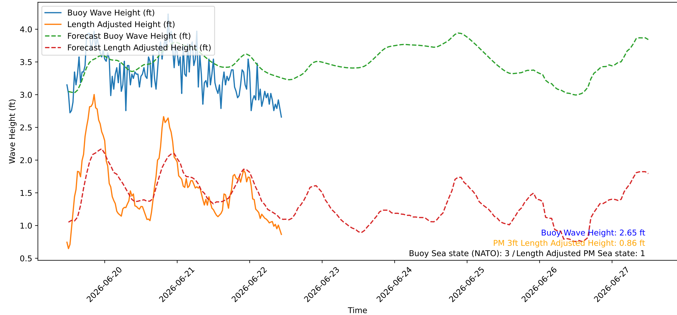
Wave Heights over Time for Green Beach at 2026-06-22 11:31:08
