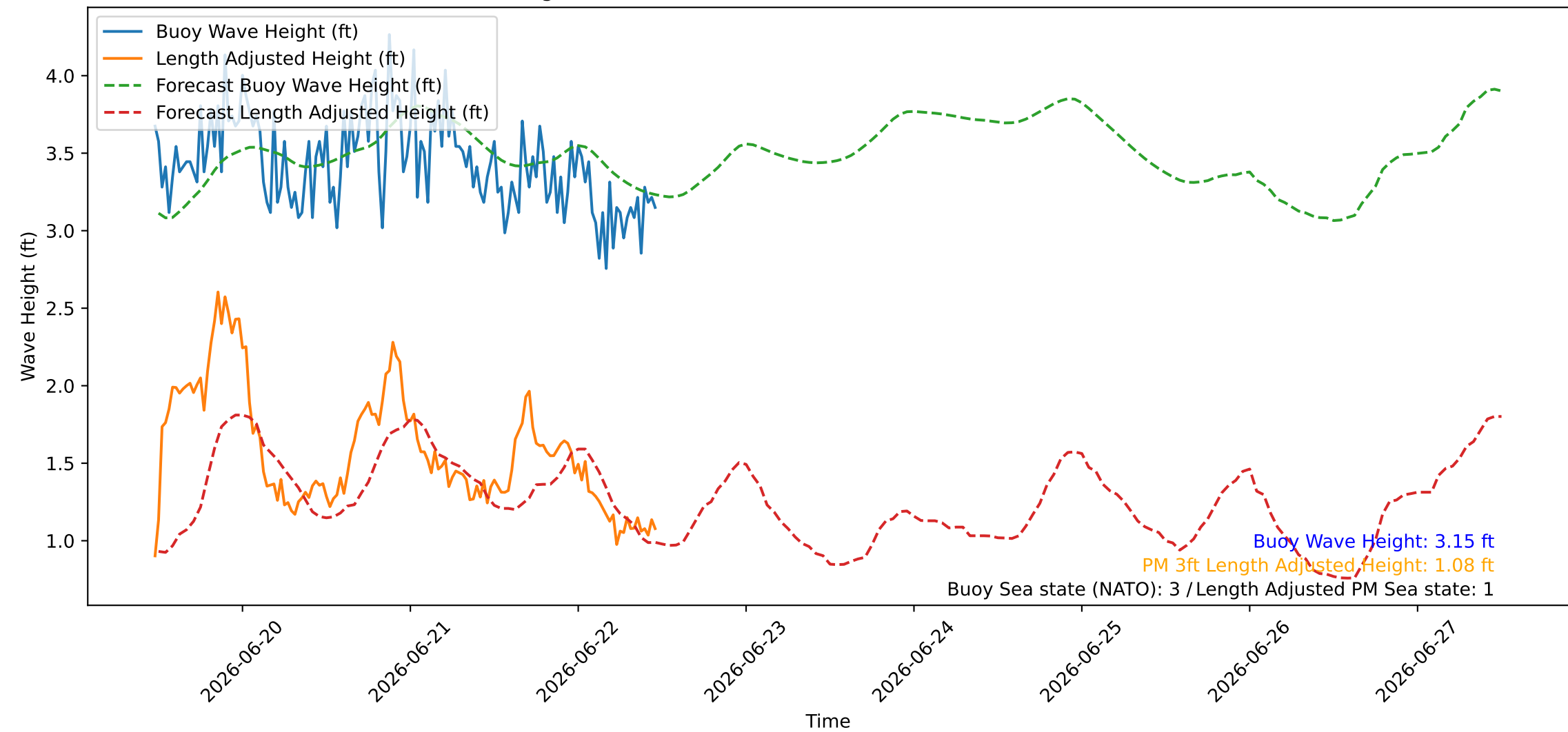
Wave Heights over Time for Oceanside Harbor at 2026-06-22 11:30:26
