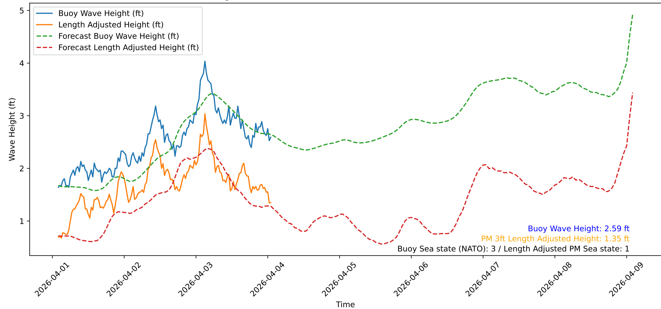
Wave Heights over Time for Oceanside Harbor at 2026-04-04 01:50:31
