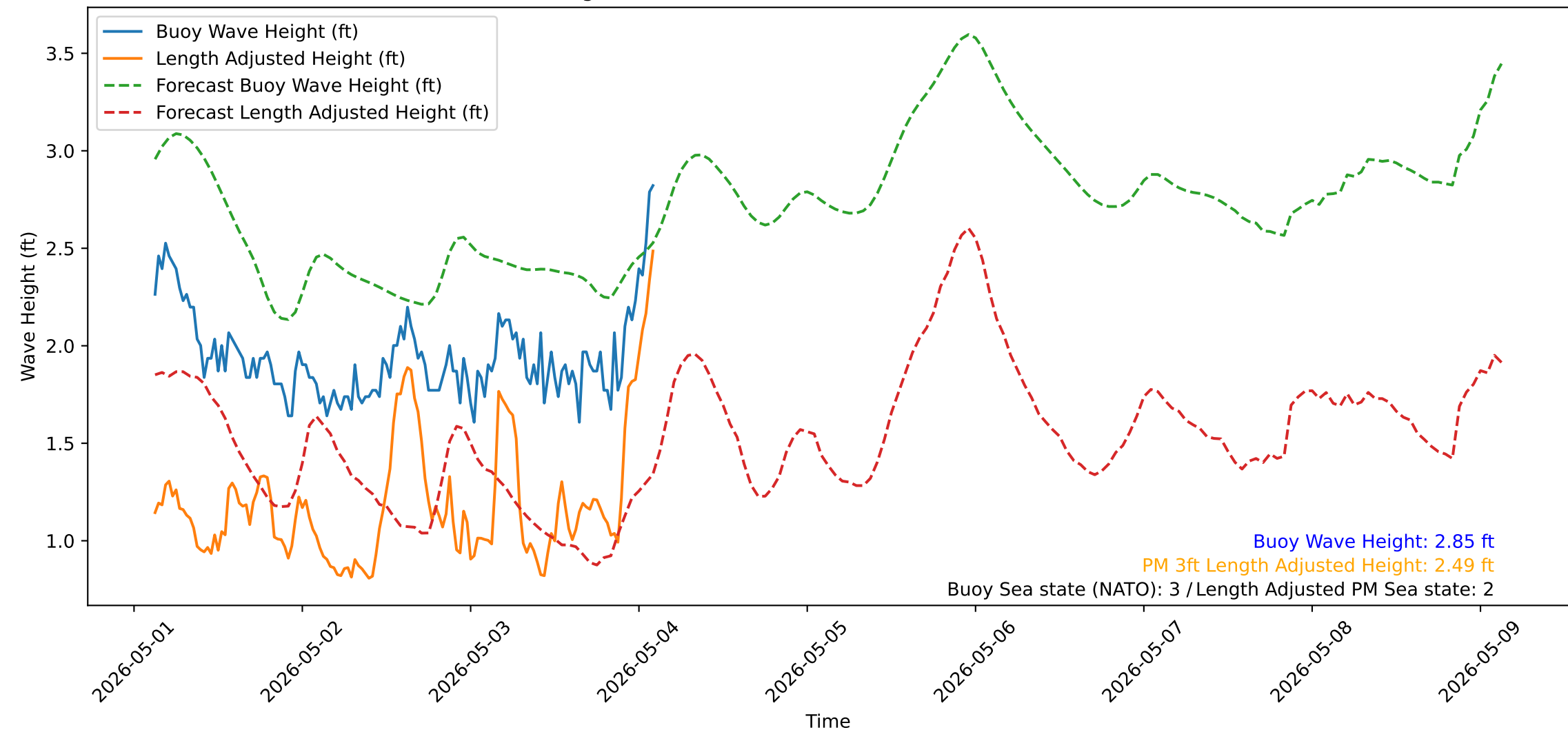
Wave Heights over Time for Red Beach at 2026-05-04 02:40:50
