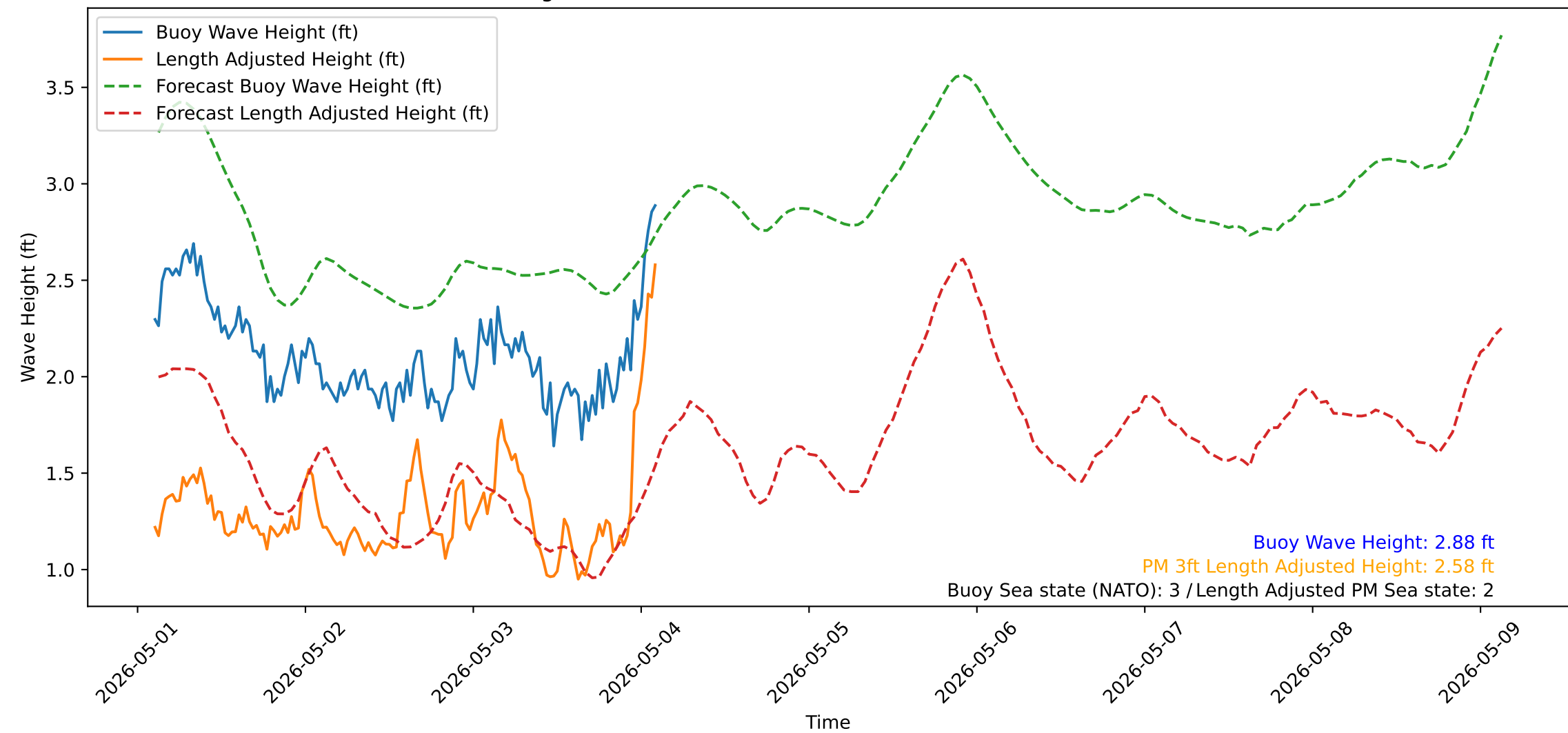
Wave Heights over Time for Oceanside Harbor at 2026-05-04 02:40:31
