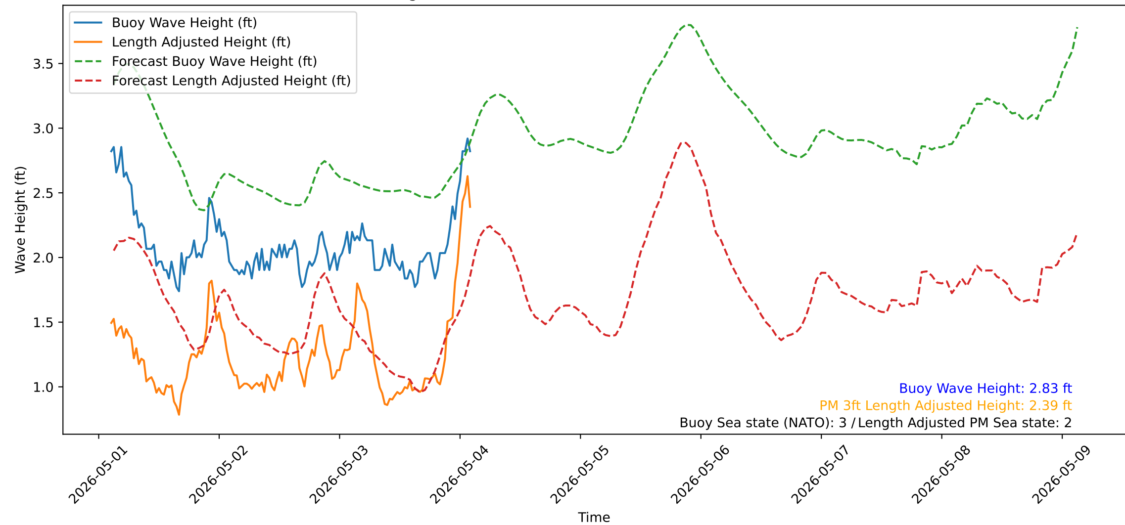
Wave Heights over Time for Green Beach at 2026-05-04 02:41:12
