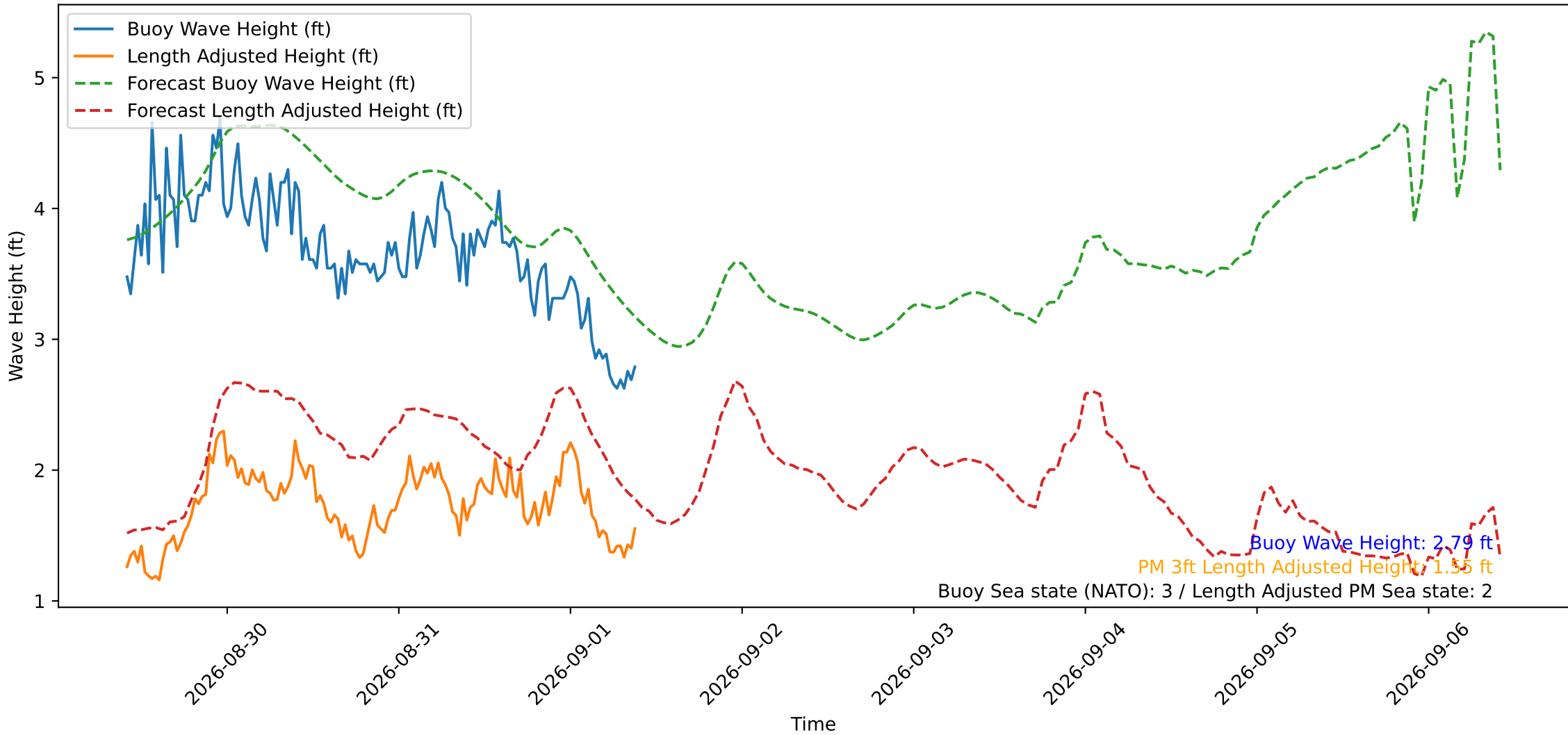
Wave Heights over Time for Red Beach at 2026-09-01 09:50:51
