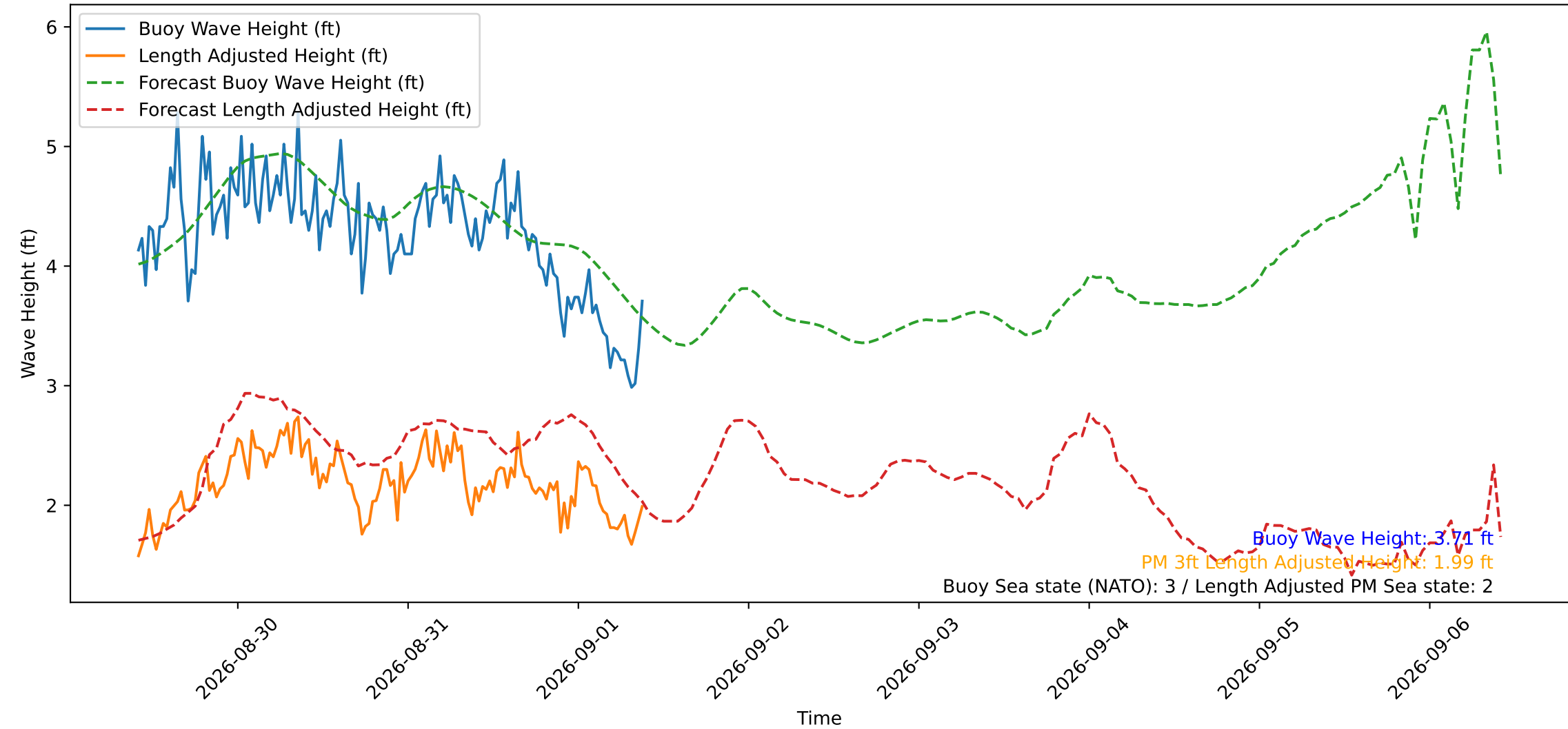
Wave Heights over Time for Oceanside Harbor at 2026-09-01 09:50:30
