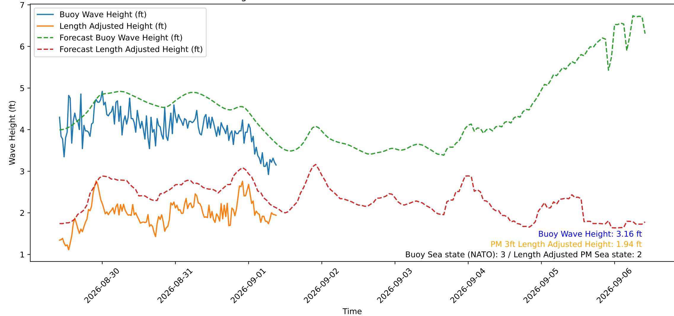
Wave Heights over Time for Green Beach at 2026-09-01 09:51:15
