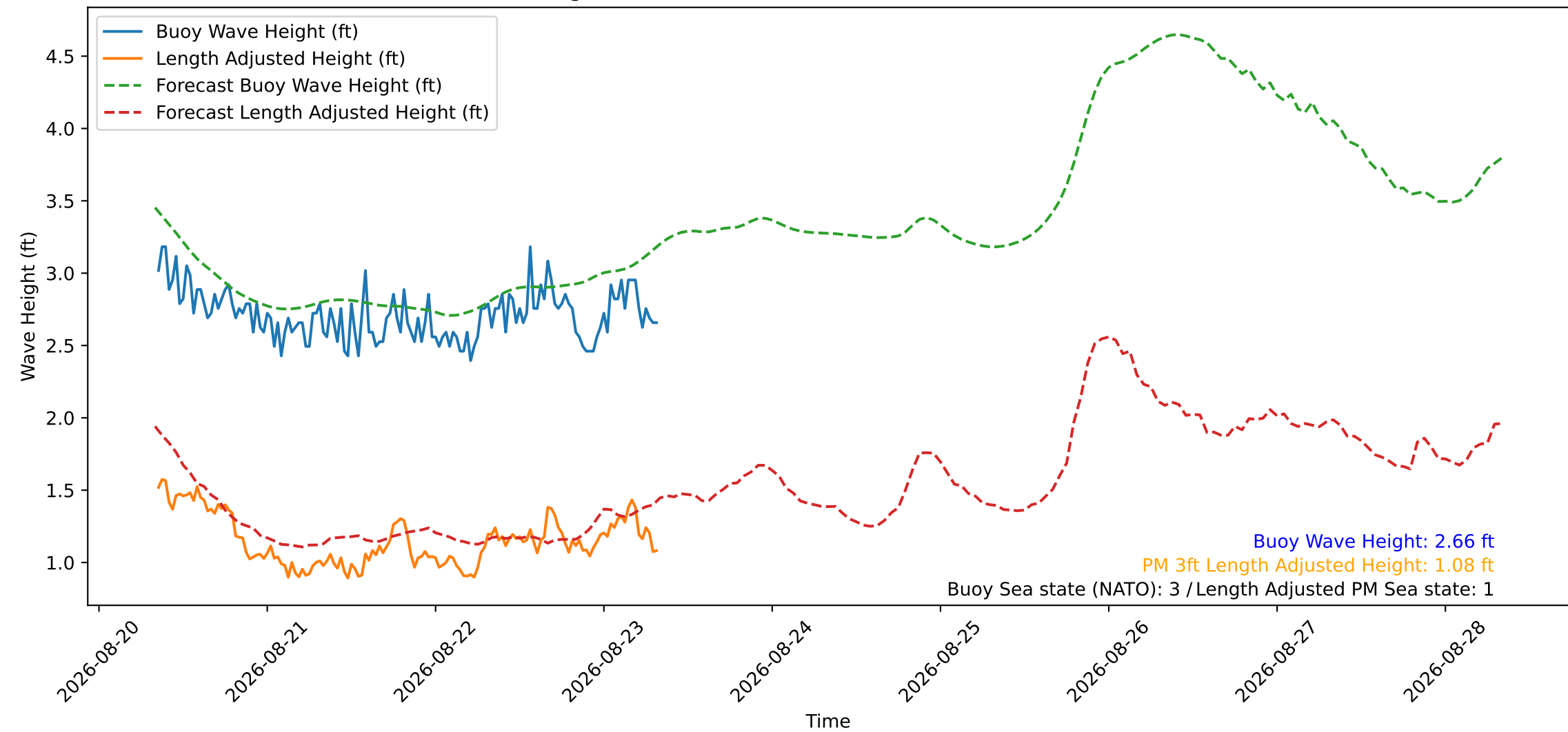
Wave Heights over Time for Green Beach at 2026-08-23 08:21:15
