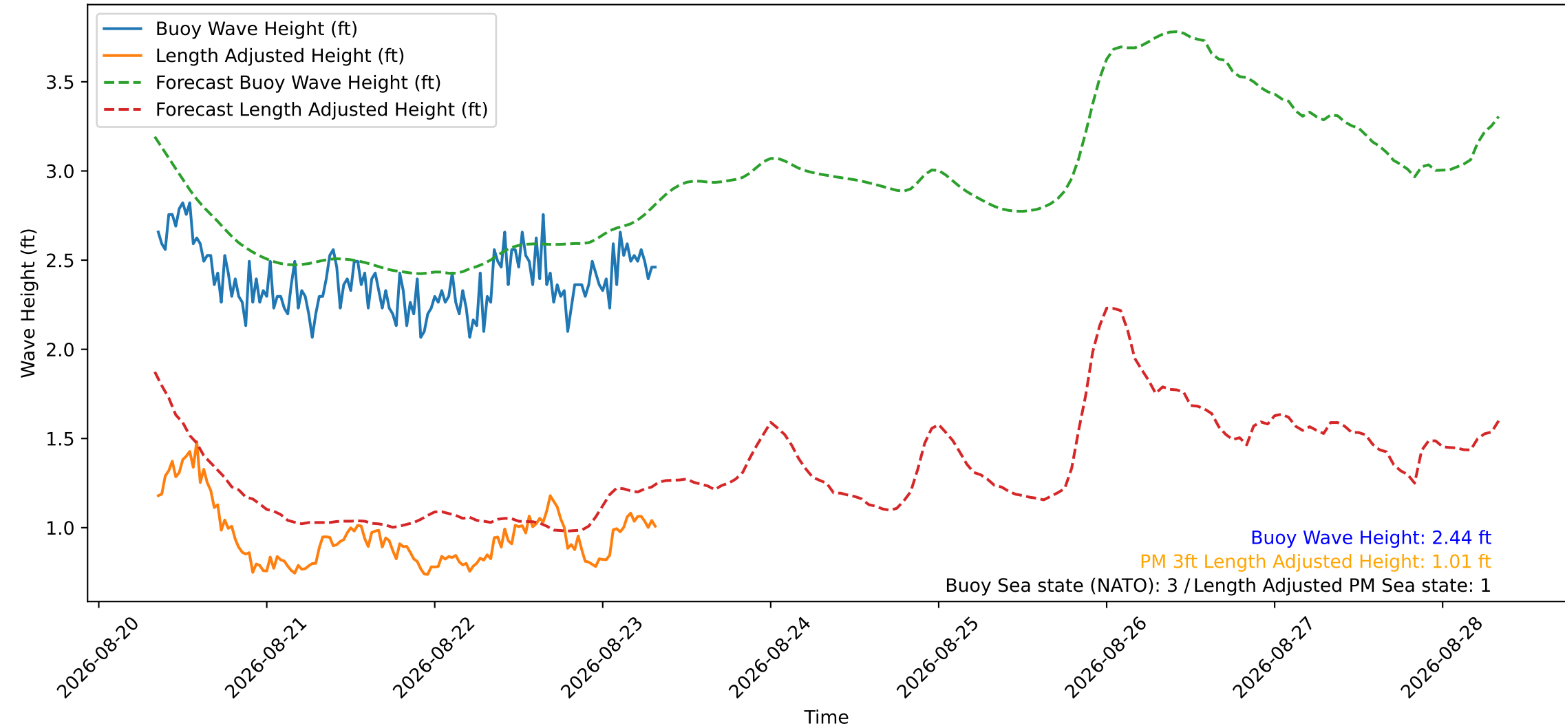
Wave Heights over Time for Red Beach at 2026-08-23 08:20:51
