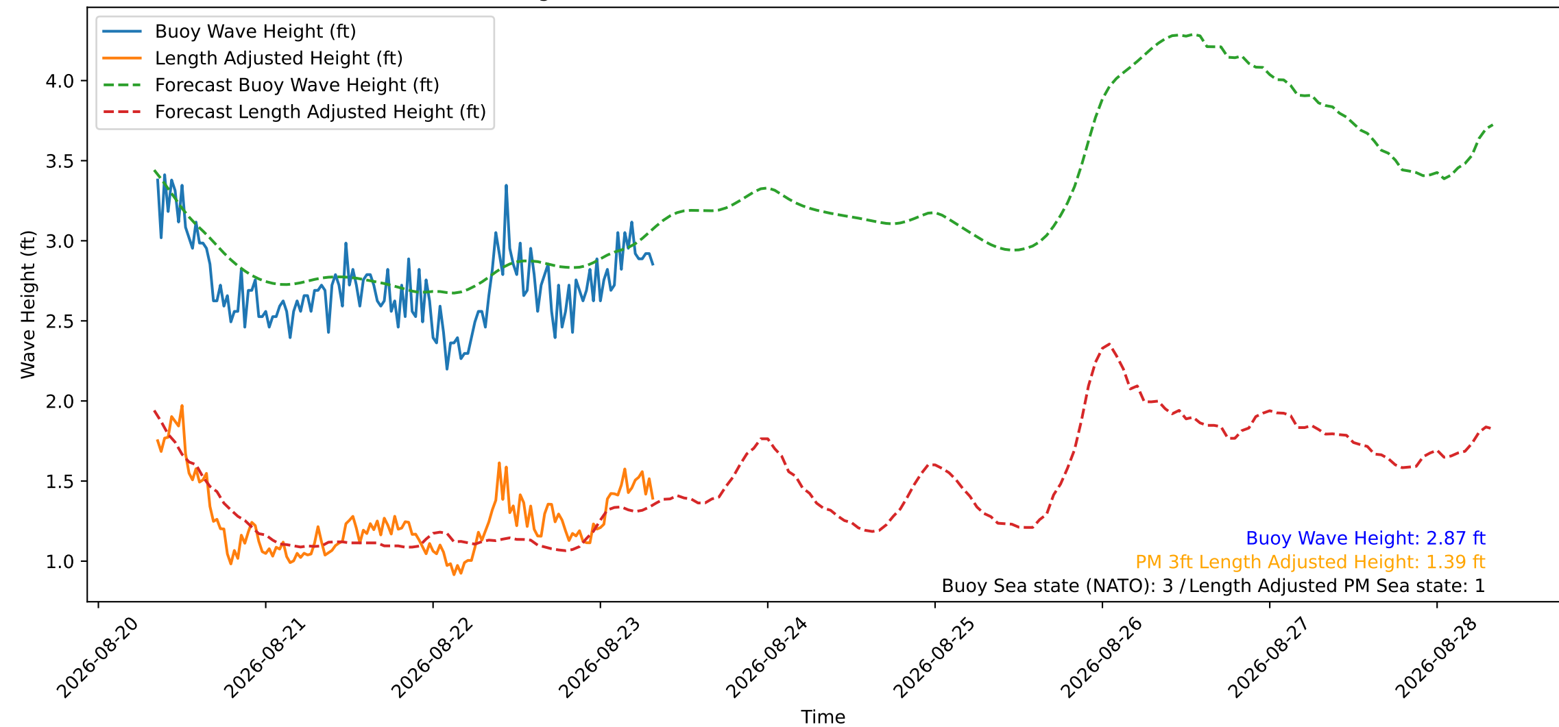
Wave Heights over Time for Oceanside Harbor at 2026-08-23 08:20:30
