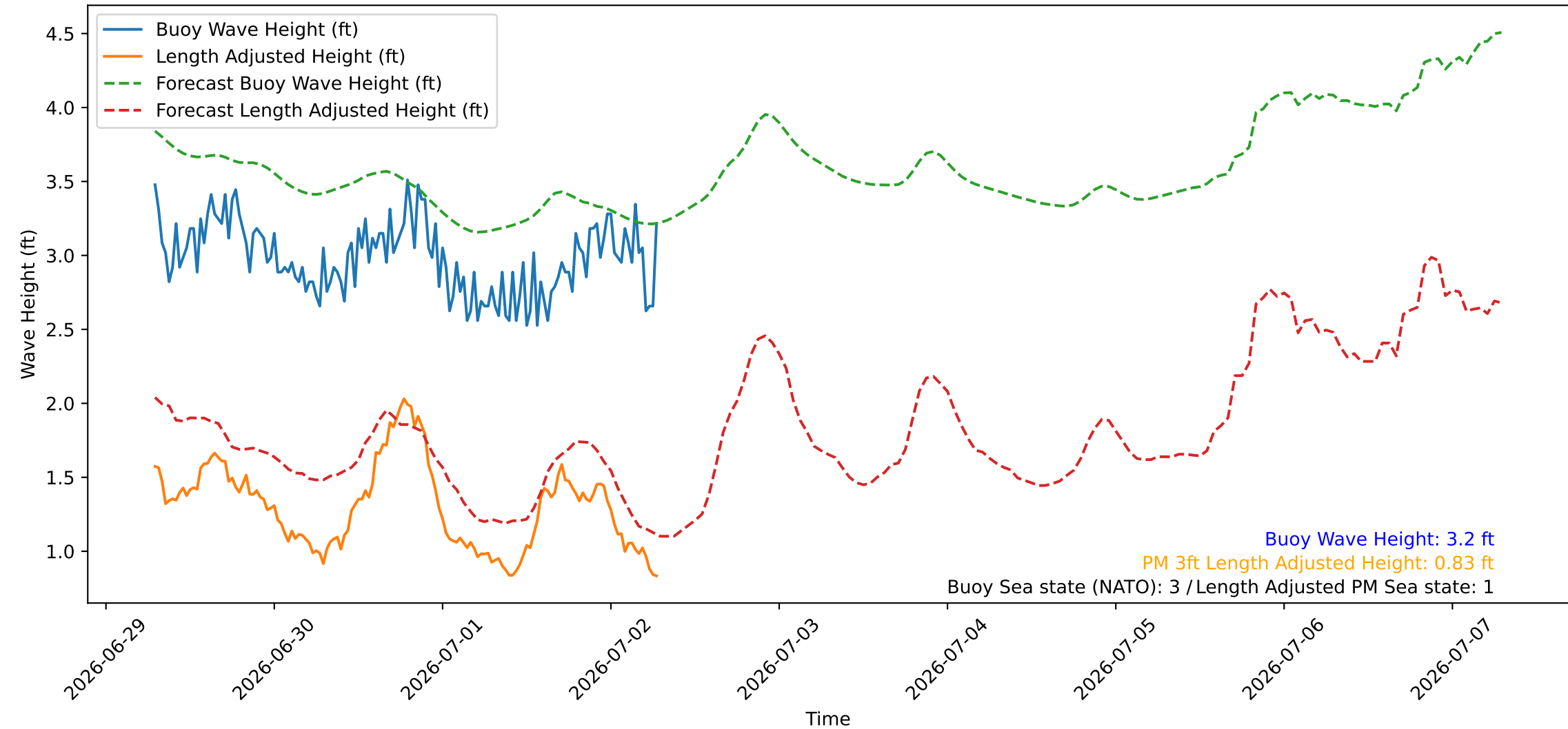
Wave Heights over Time for Green Beach at 2026-07-02 07:11:08
