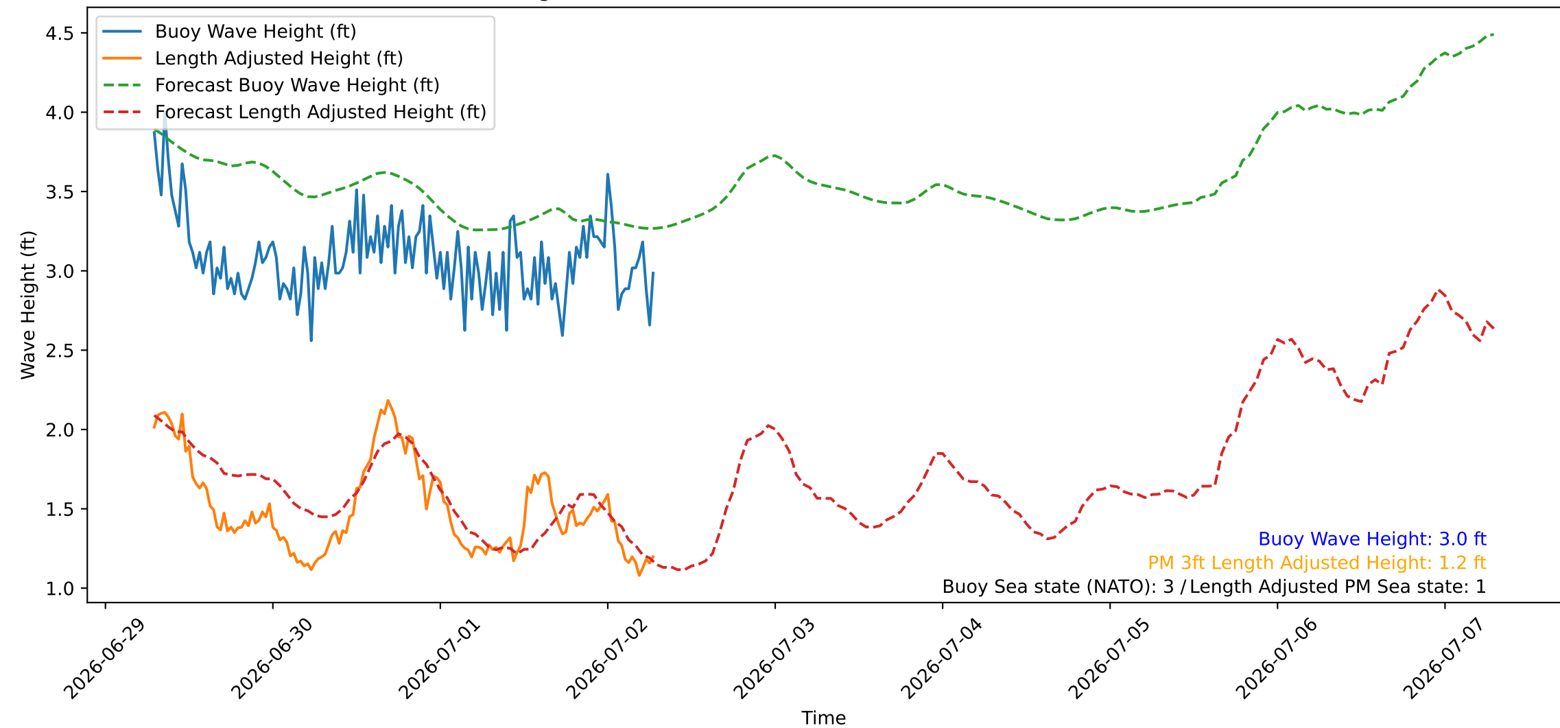
Wave Heights over Time for Oceanside Harbor at 2026-07-02 07:10:26
