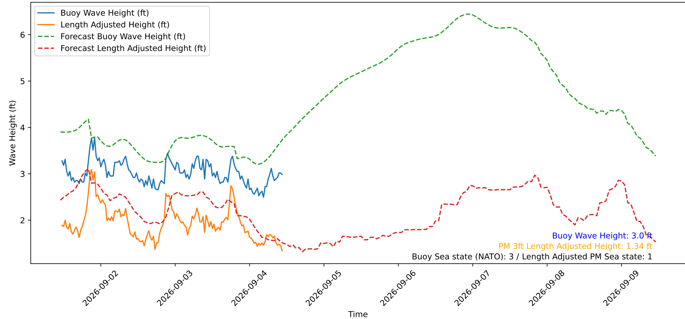
Wave Heights over Time for Green Beach at 2026-09-04 11:21:16
