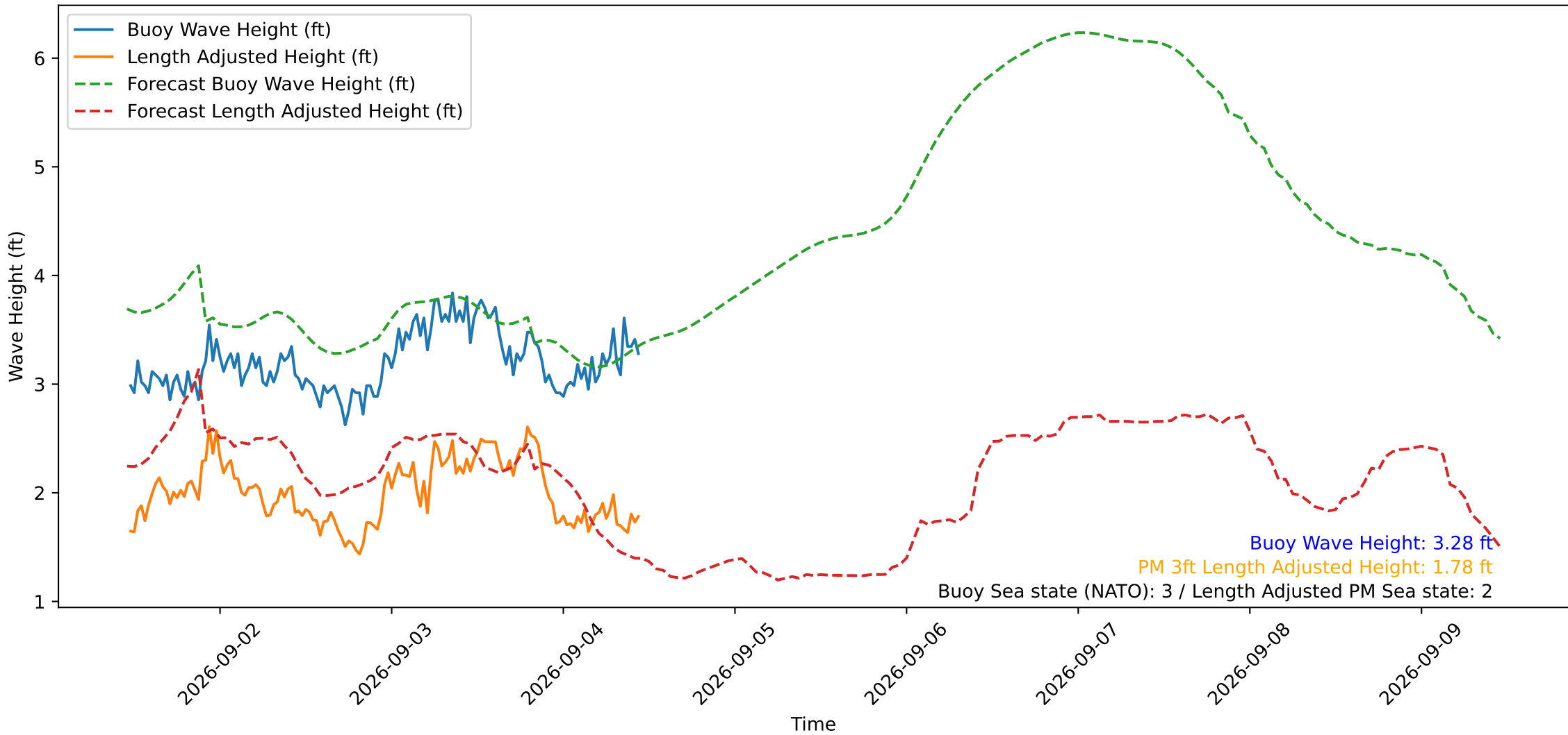
Wave Heights over Time for Oceanside Harbor at 2026-09-04 11:20:30
