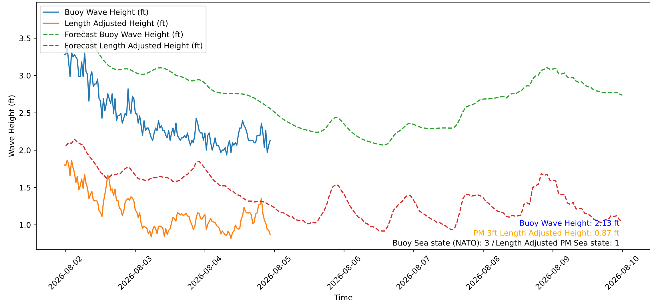
Wave Heights over Time for Green Beach at 2026-08-04 23:31:08
