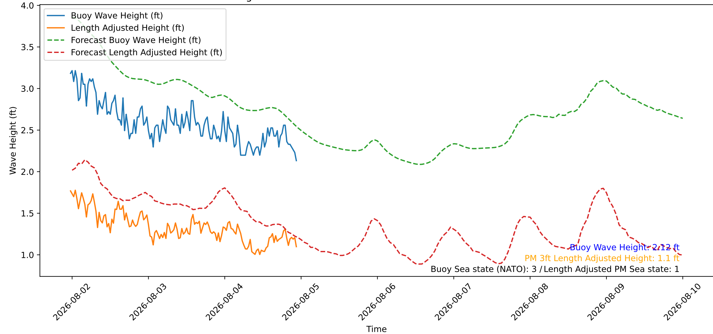
Wave Heights over Time for Oceanside Harbor at 2026-08-04 23:30:26
