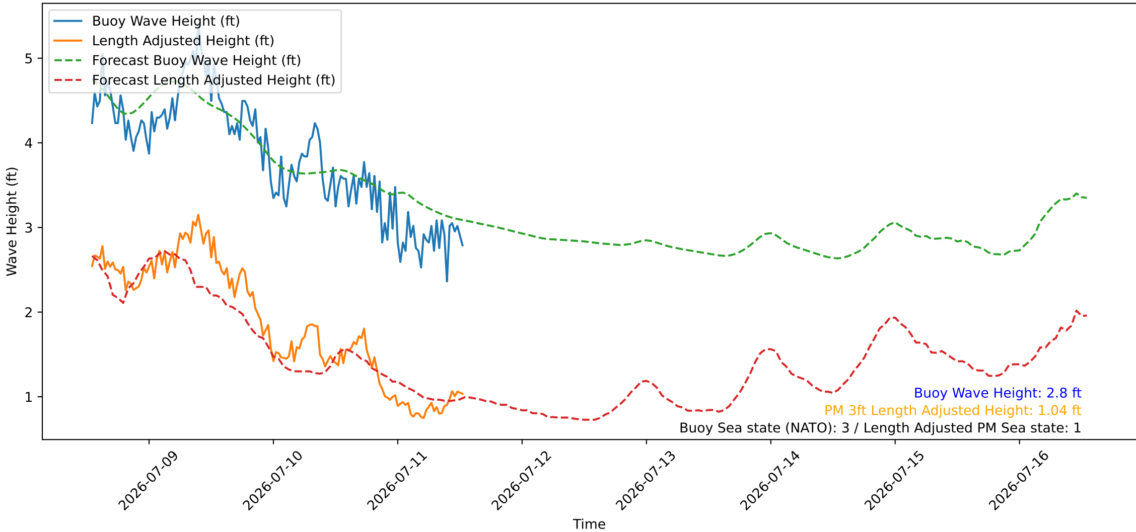
Wave Heights over Time for Oceanside Harbor at 2026-07-11 13:10:26
