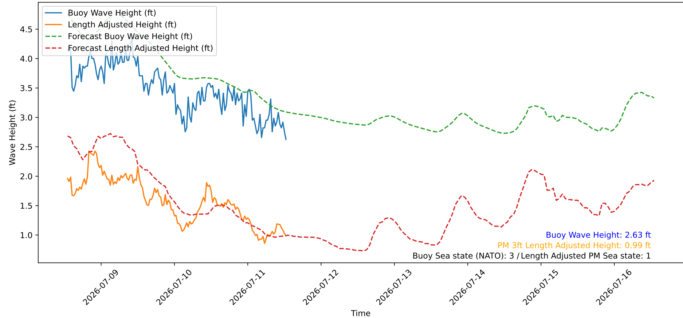
Wave Heights over Time for Green Beach at 2026-07-11 13:11:07
