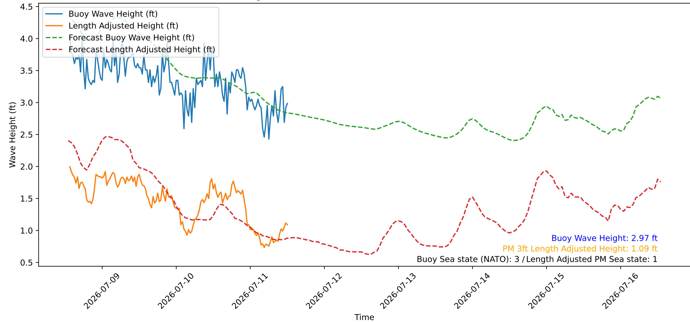
Wave Heights over Time for Red Beach at 2026-07-11 13:10:45
