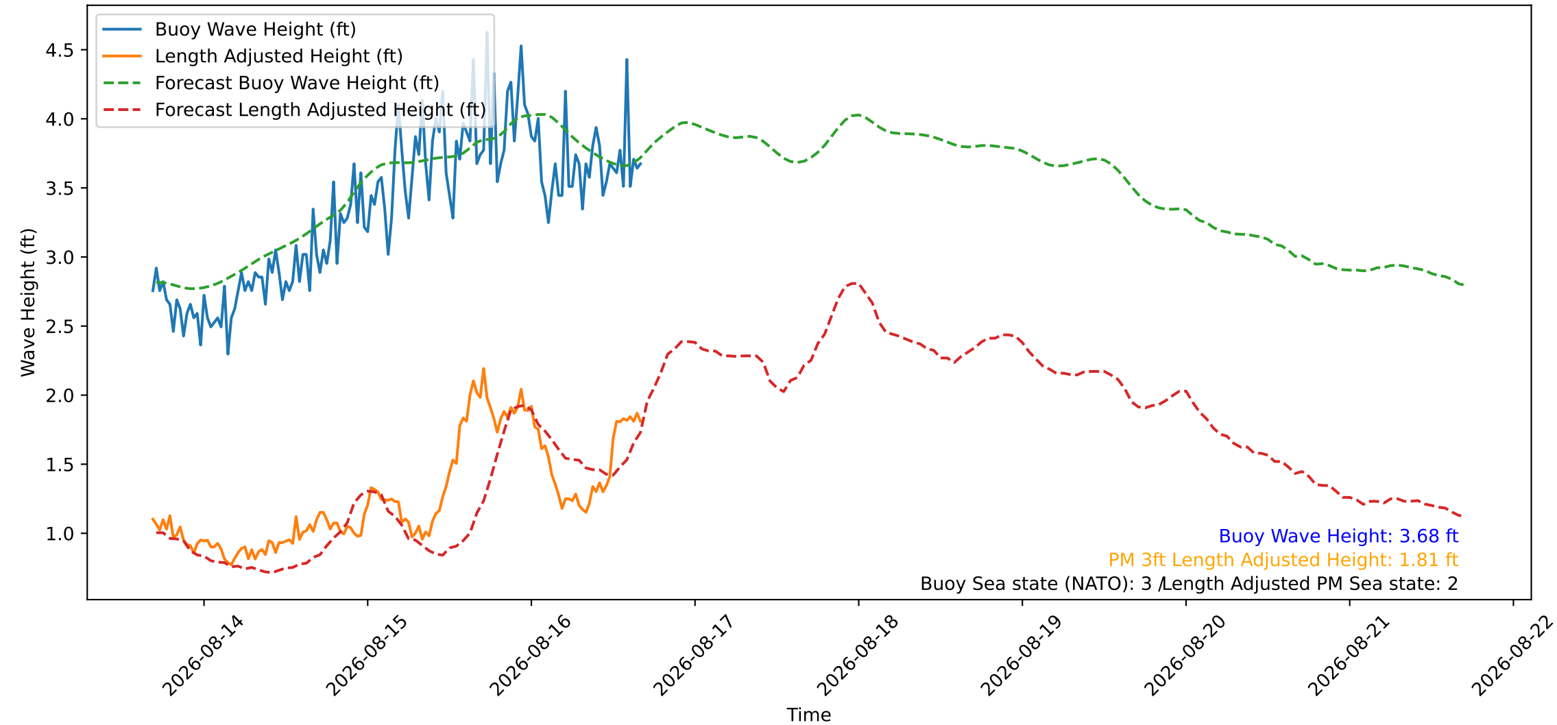
Wave Heights over Time for Oceanside Harbor at 2026-08-16 16:40:26
