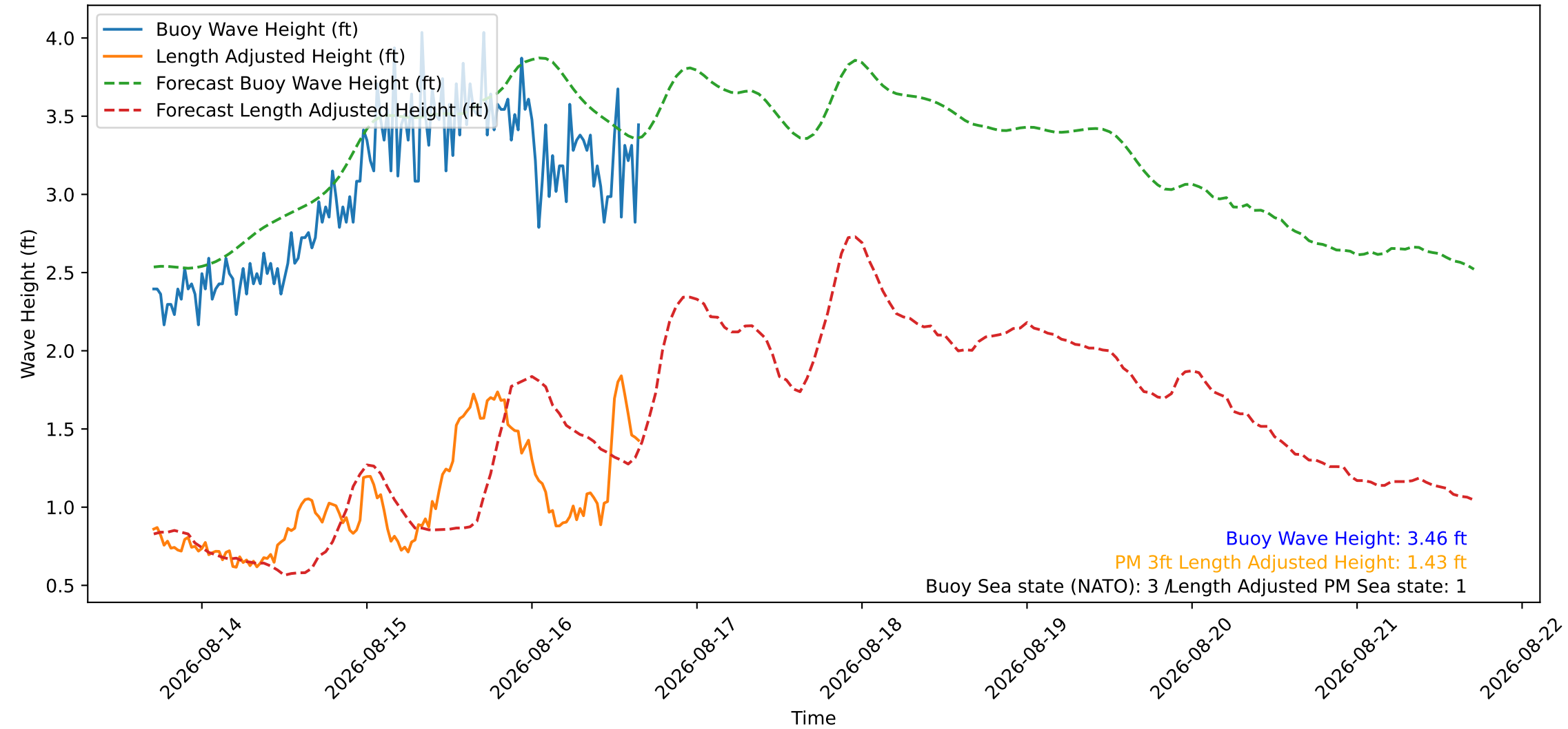
Wave Heights over Time for Red Beach at 2026-08-16 16:40:45
