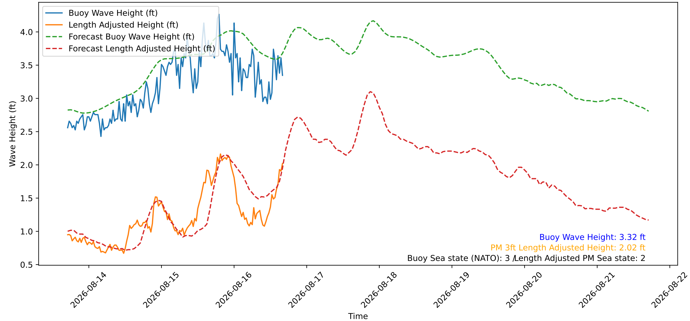
Wave Heights over Time for Green Beach at 2026-08-16 16:41:08
