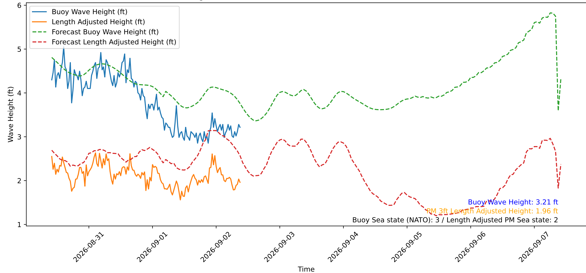
Wave Heights over Time for Oceanside Harbor at 2026-09-02 10:00:30
