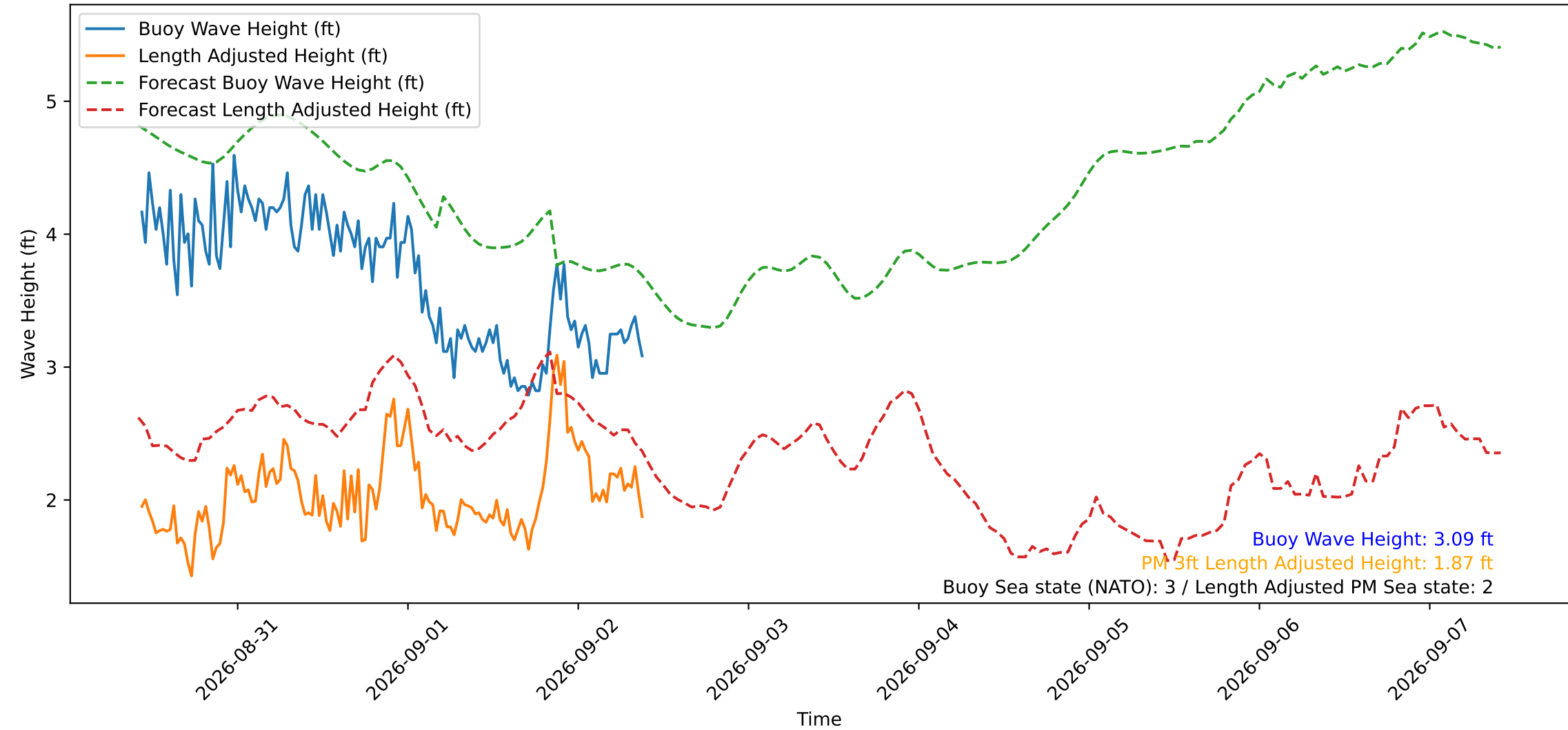
Wave Heights over Time for Green Beach at 2026-09-02 10:01:12
