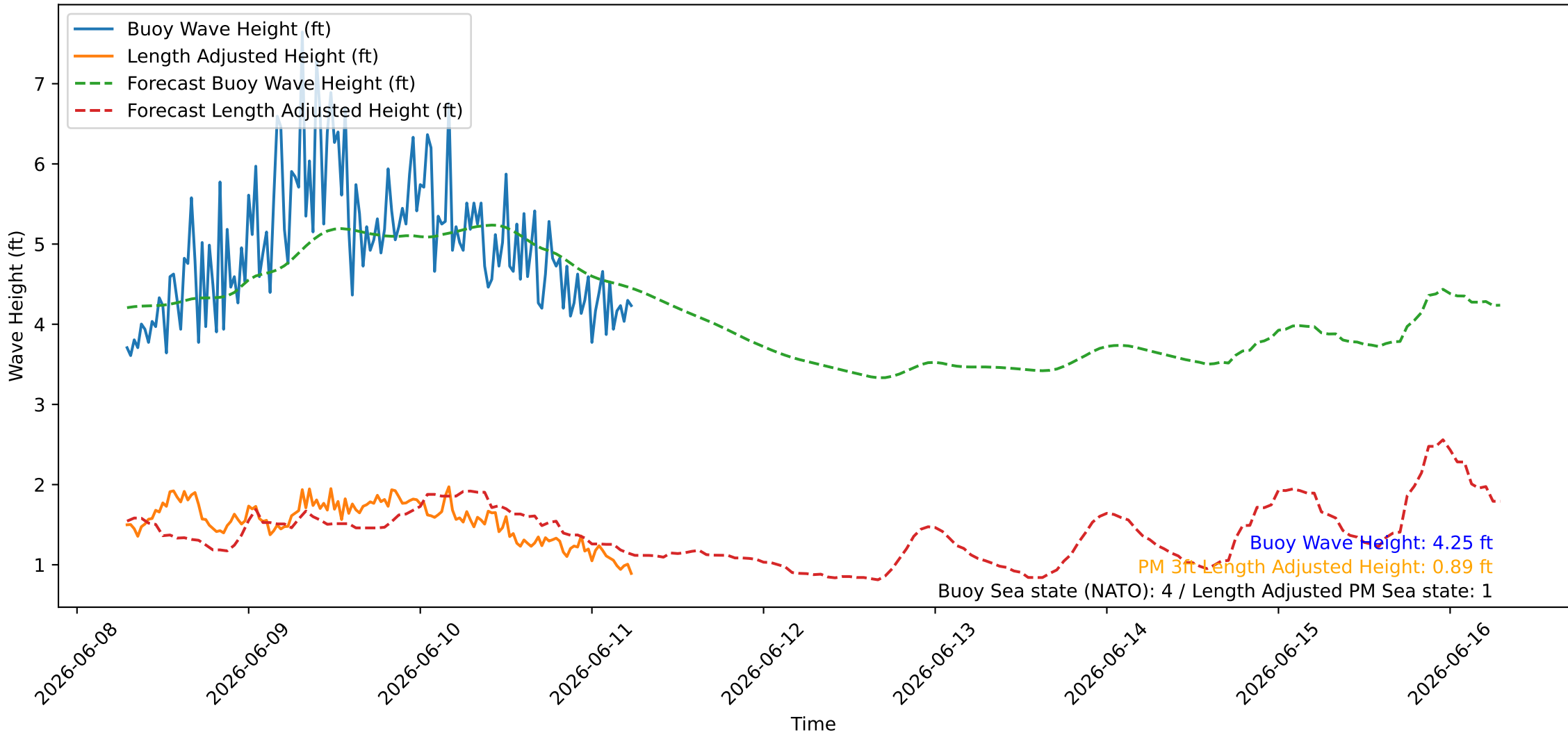
Wave Heights over Time for Red Beach at 2026-06-11 06:30:48
