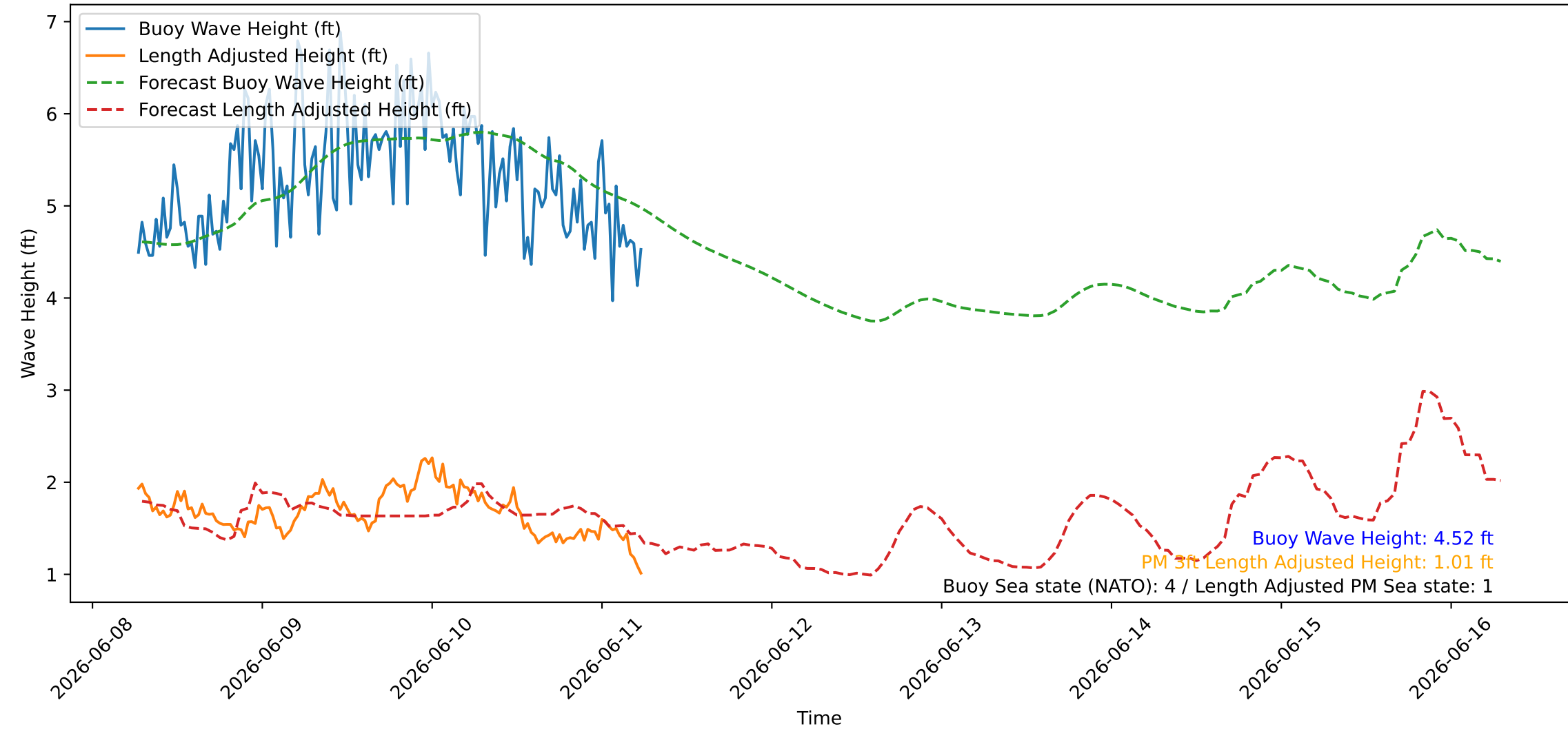
Wave Heights over Time for Green Beach at 2026-06-11 06:31:11
