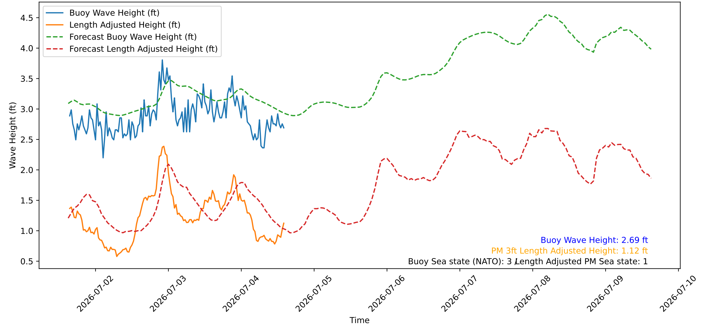
Wave Heights over Time for Red Beach at 2026-07-04 15:00:44
