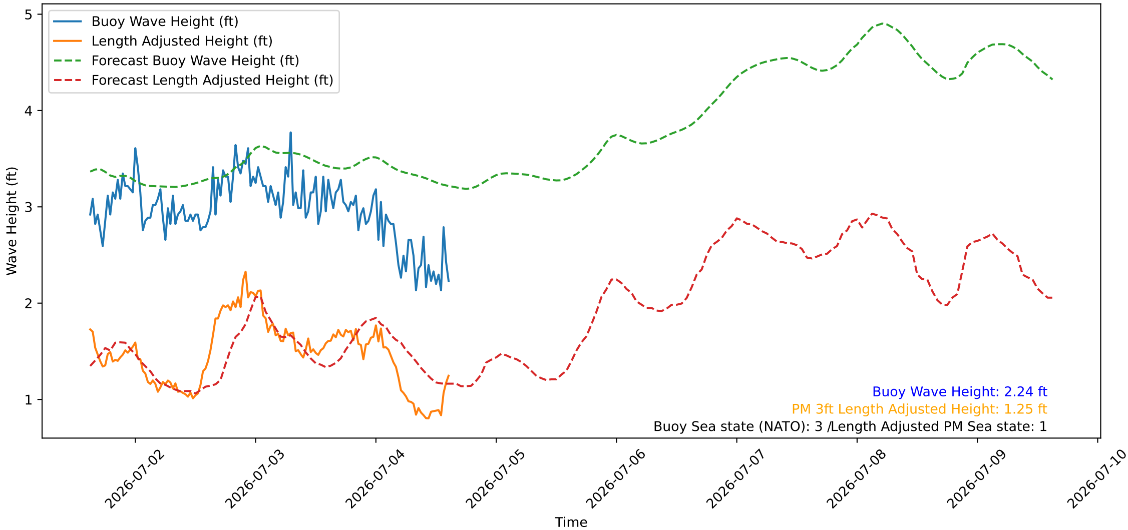
Wave Heights over Time for Oceanside Harbor at 2026-07-04 15:00:25
