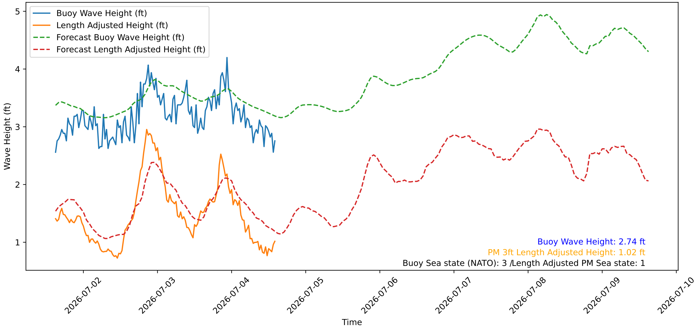
Wave Heights over Time for Green Beach at 2026-07-04 15:01:07
