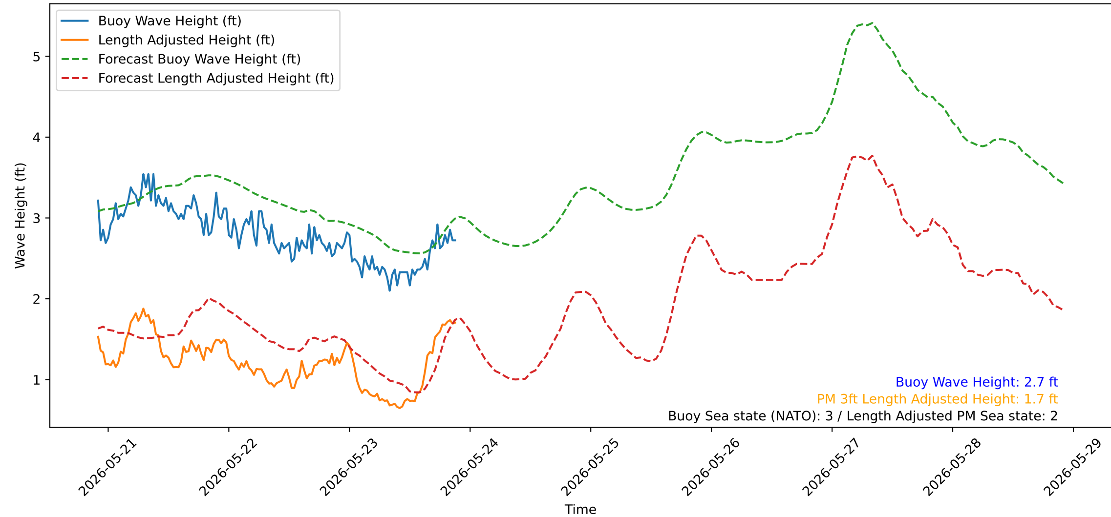
Wave Heights over Time for Green Beach at 2026-05-23 22:01:13
