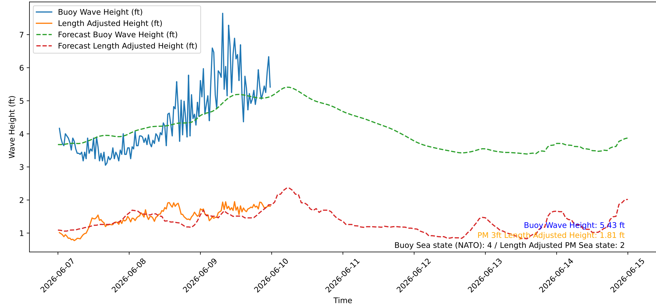
Wave Heights over Time for Red Beach at 2026-06-10 00:20:48
