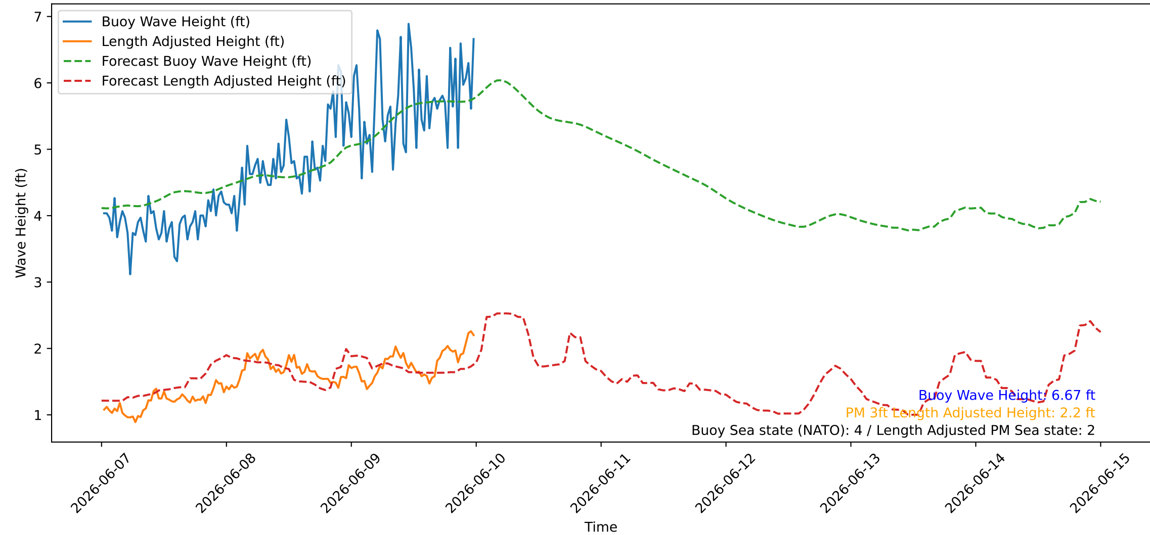
Wave Heights over Time for Green Beach at 2026-06-10 00:21:11
