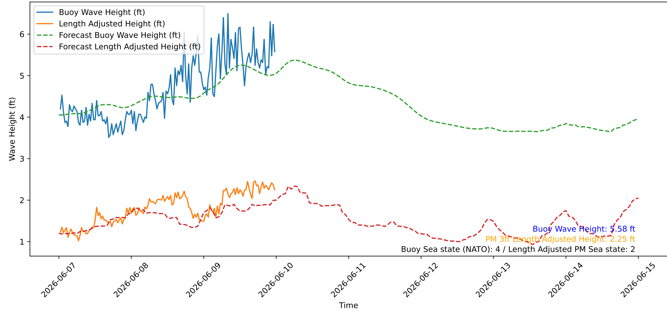
Wave Heights over Time for Oceanside Harbor at 2026-06-10 00:20:26
