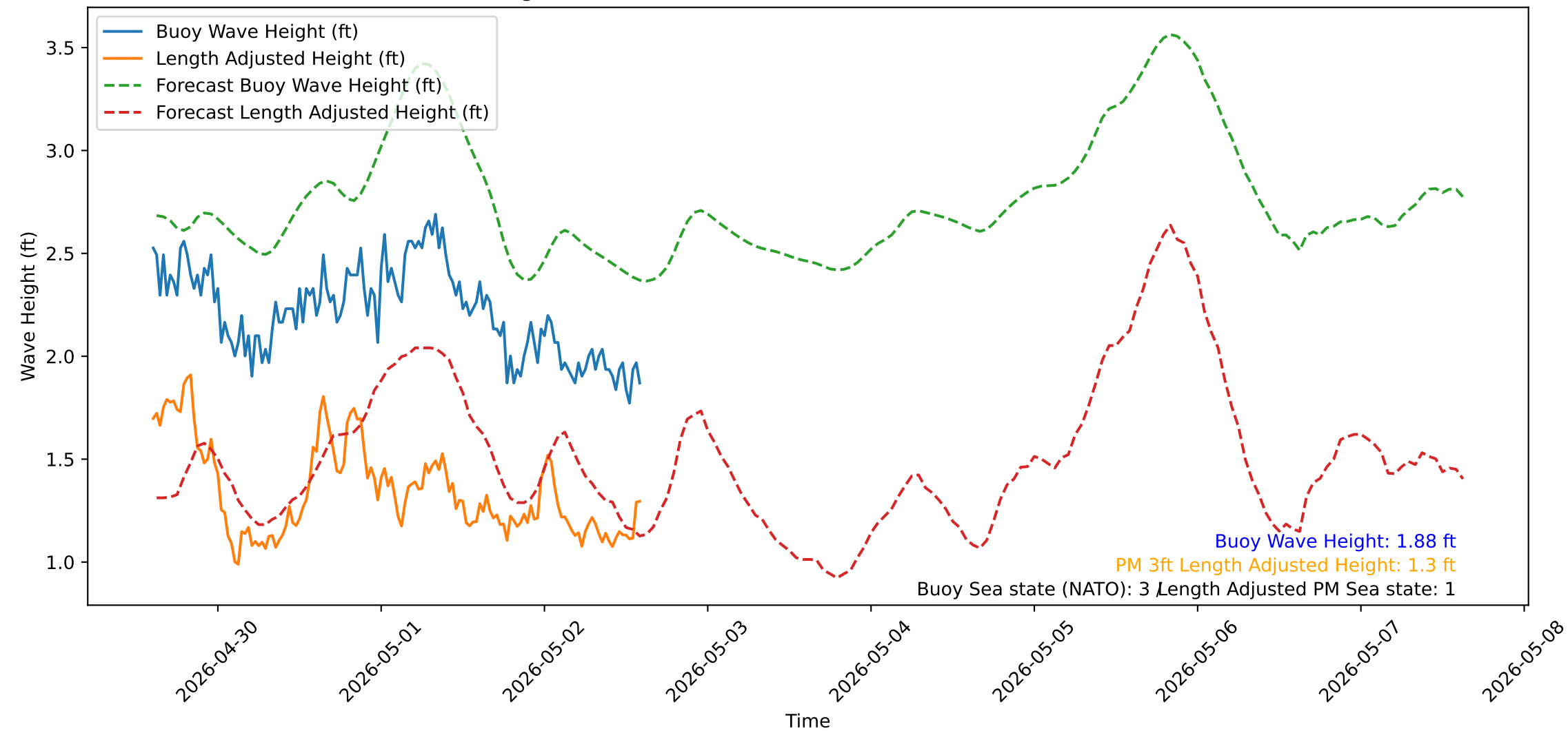
Wave Heights over Time for Oceanside Harbor at 2026-05-02 14:30:31
