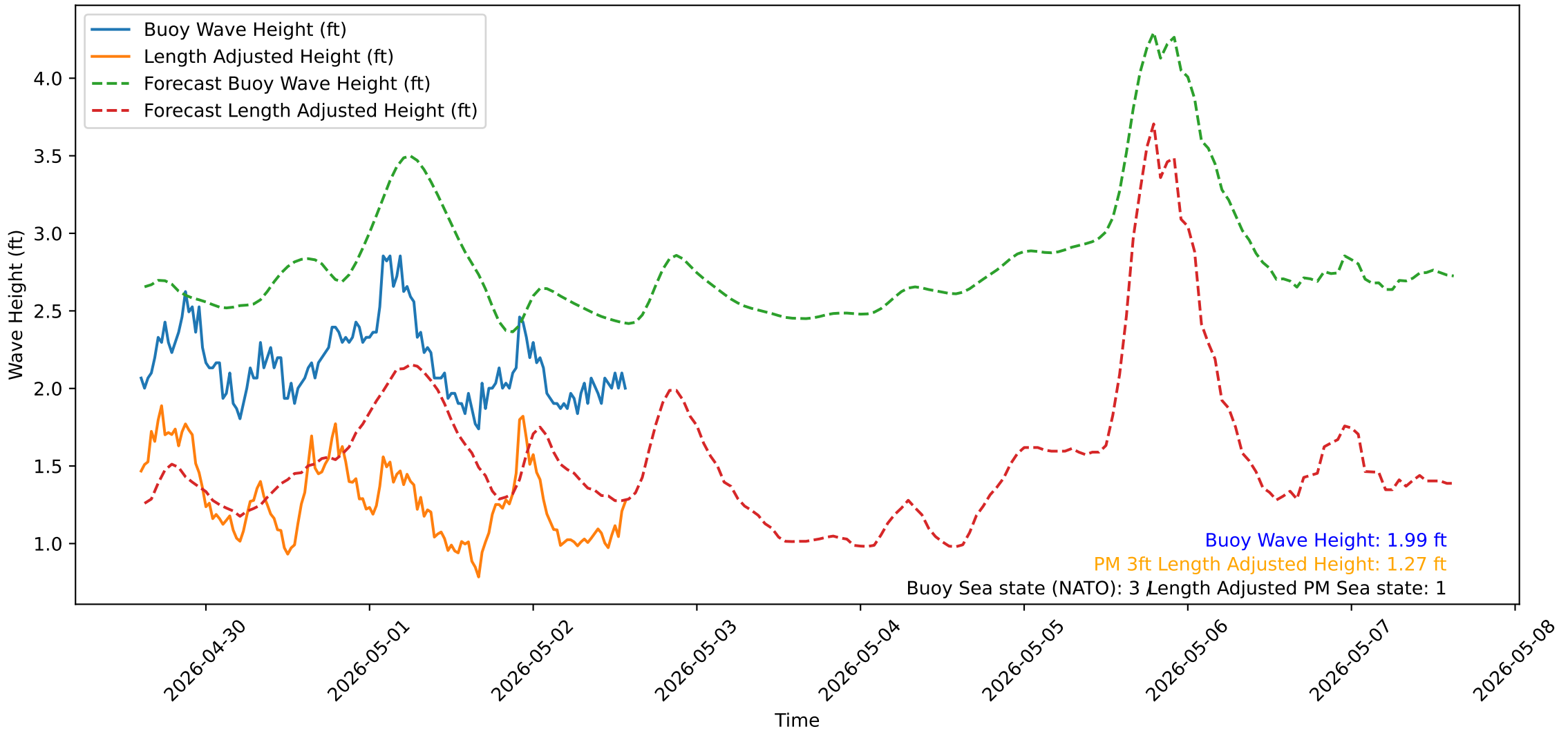
Wave Heights over Time for Green Beach at 2026-05-02 14:31:13
