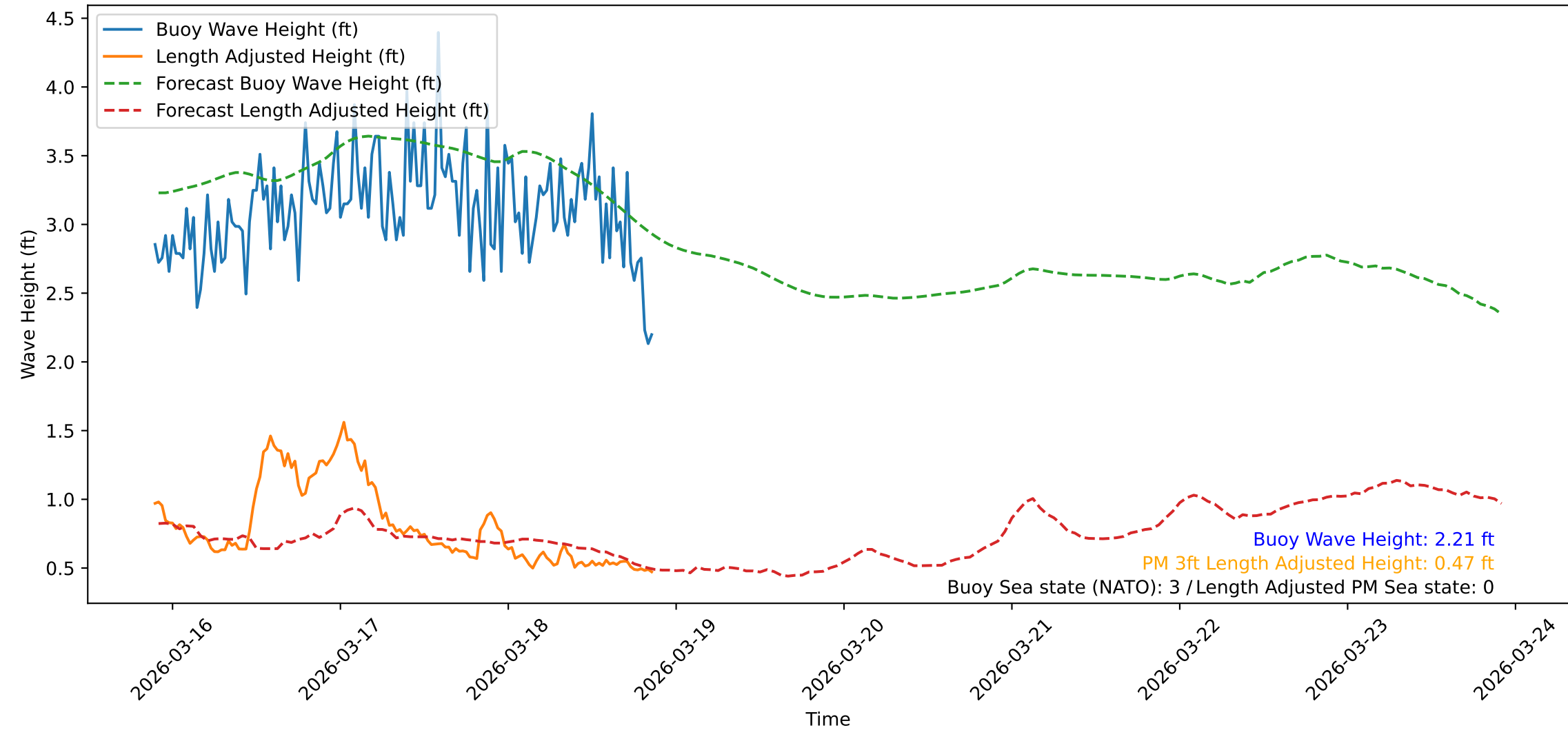
Wave Heights over Time for Oceanside Harbor at 2026-03-18 21:30:31
