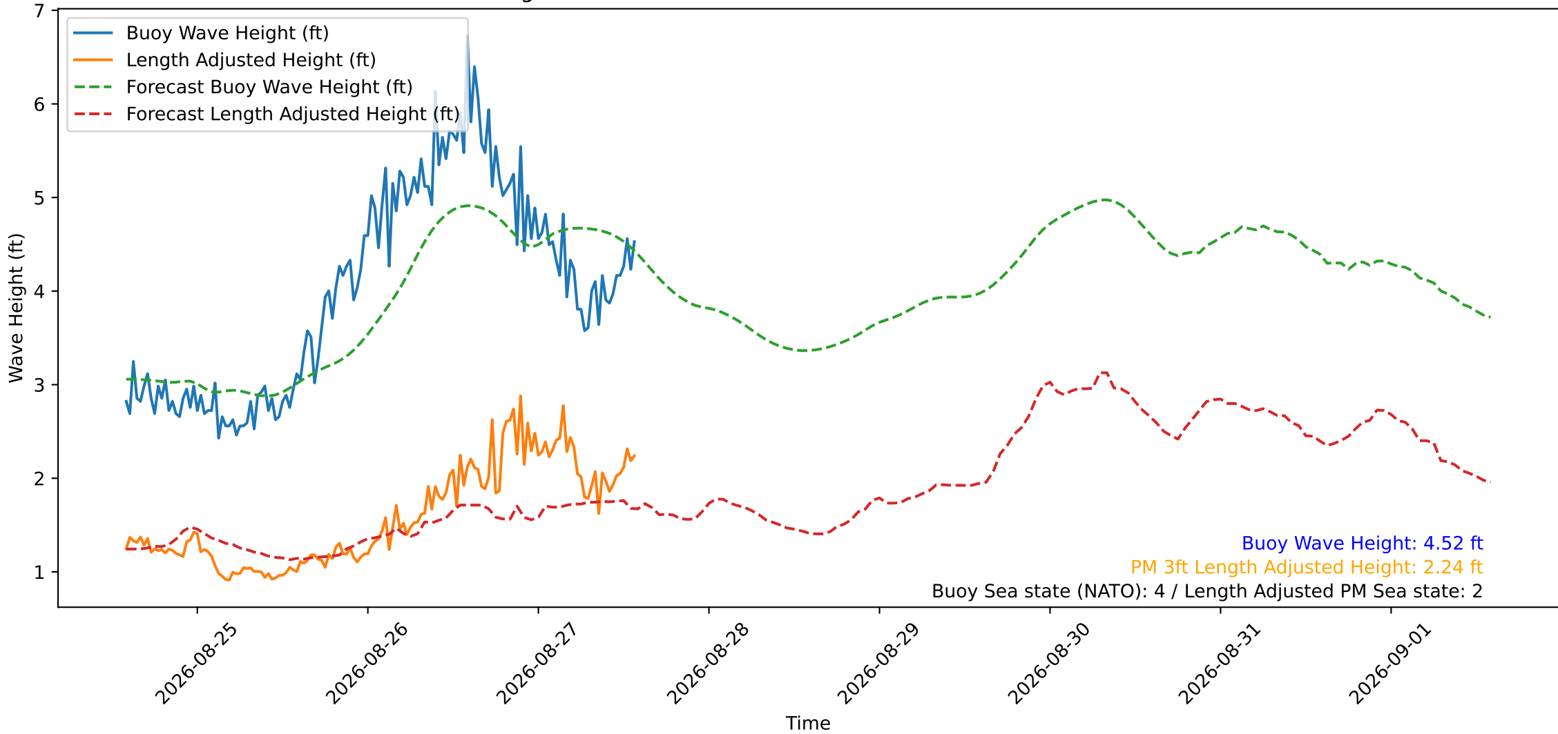
Wave Heights over Time for Oceanside Harbor at 2026-08-27 14:10:29
