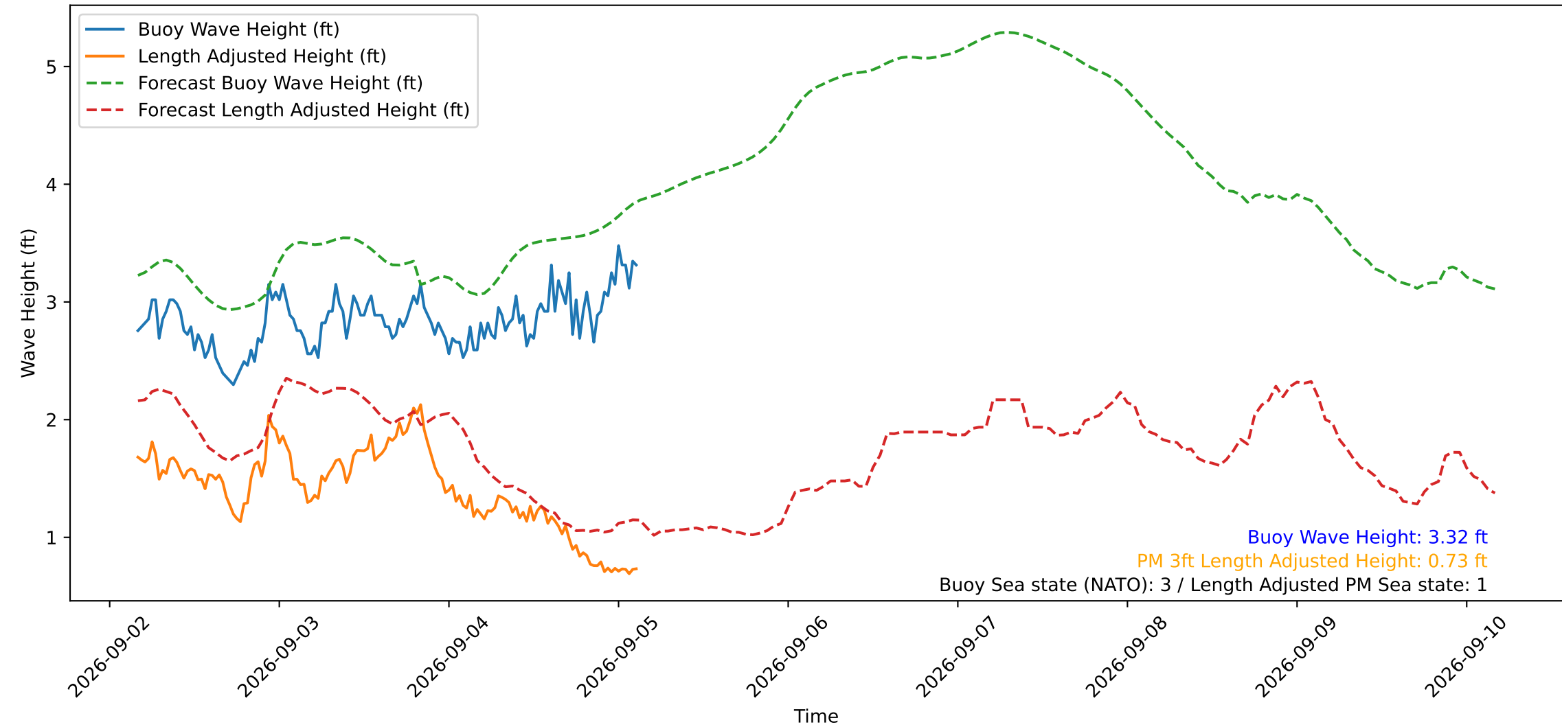
Wave Heights over Time for Red Beach at 2026-09-05 03:30:50
