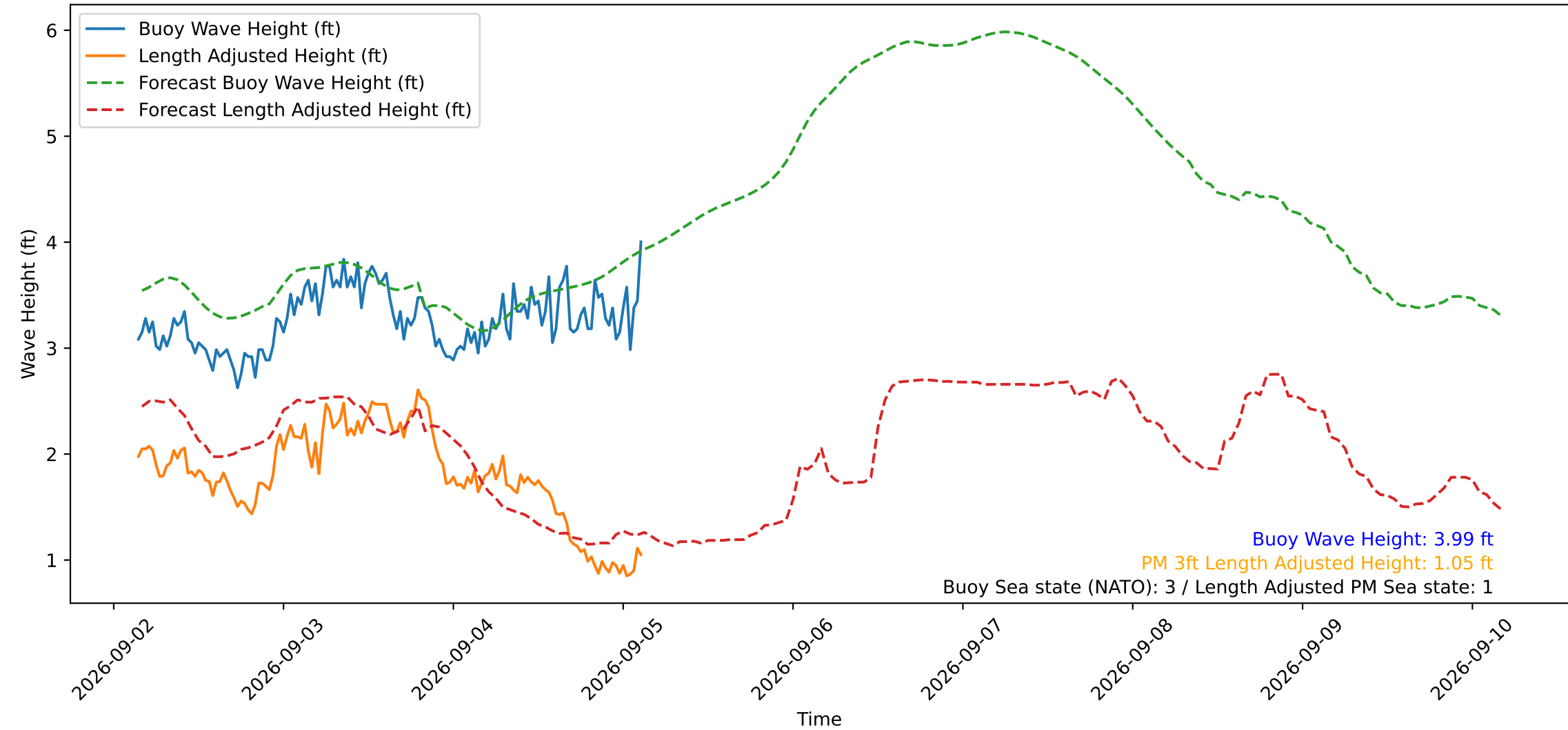
Wave Heights over Time for Oceanside Harbor at 2026-09-05 03:30:29
