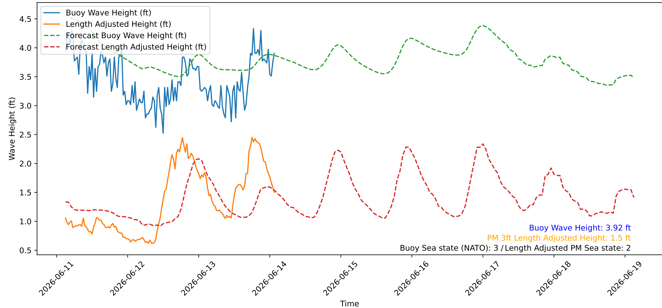
Wave Heights over Time for Red Beach at 2026-06-14 02:30:46
