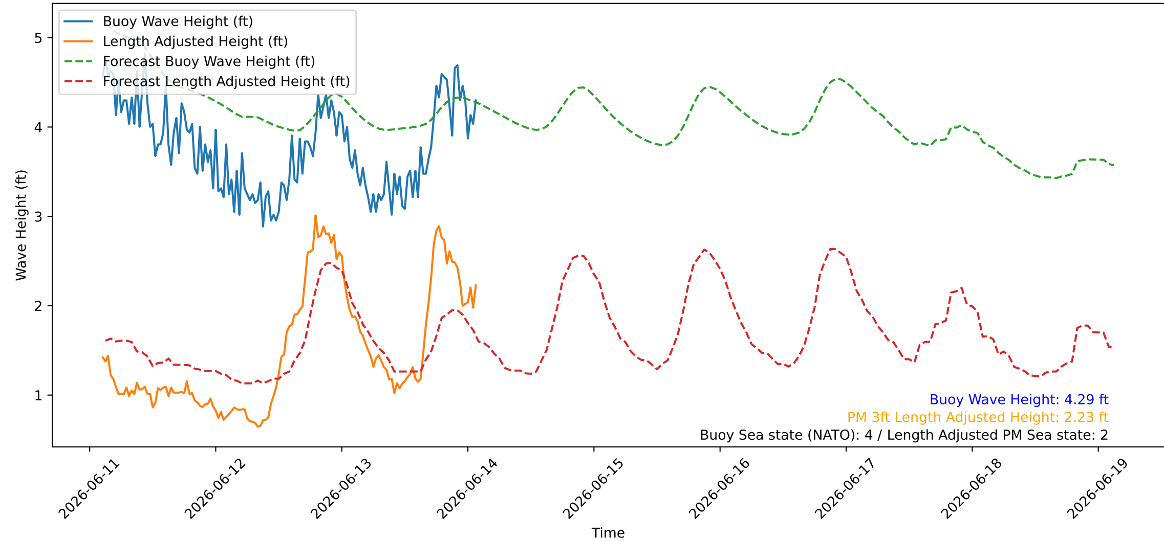
Wave Heights over Time for Green Beach at 2026-06-14 02:31:09
