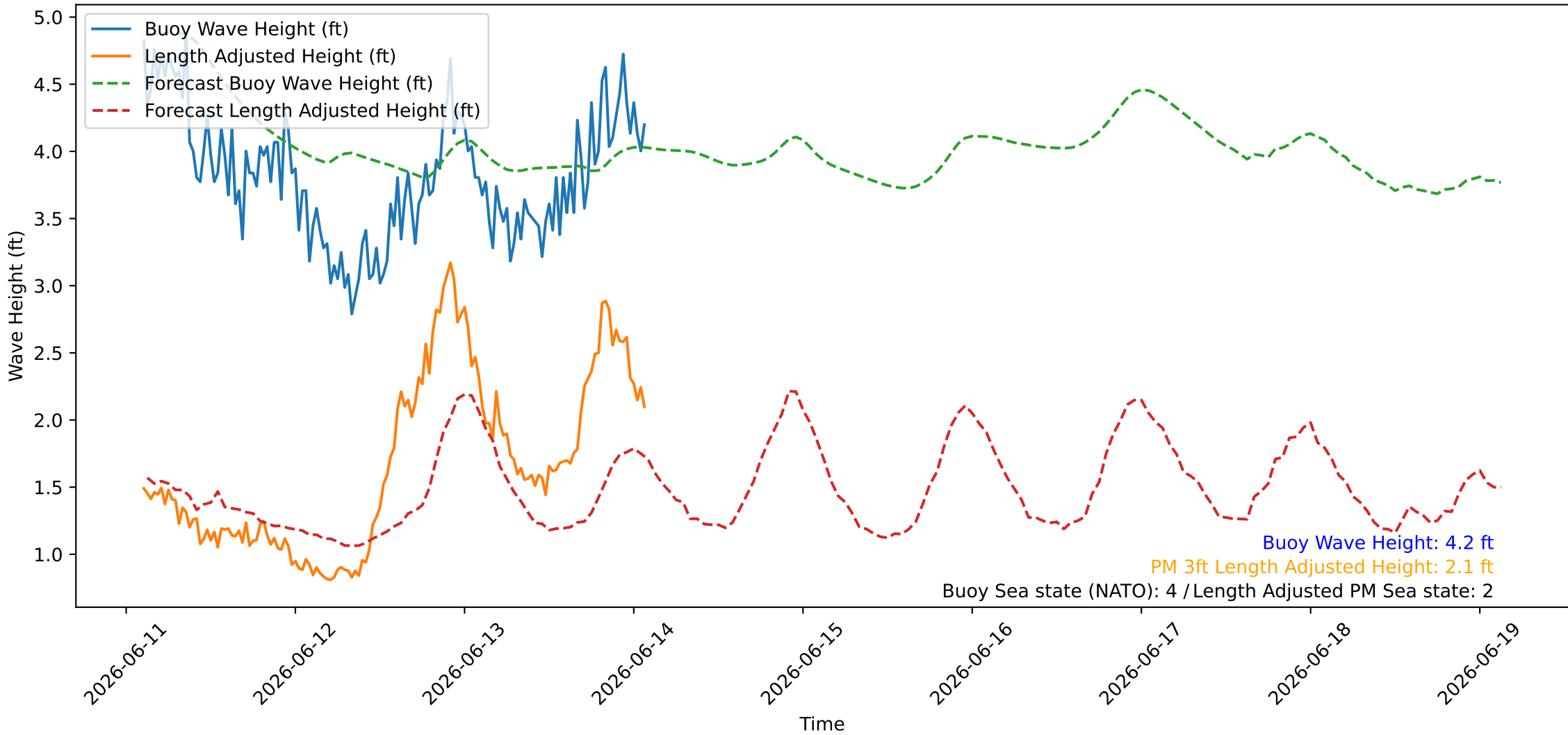
Wave Heights over Time for Oceanside Harbor at 2026-06-14 02:30:27
