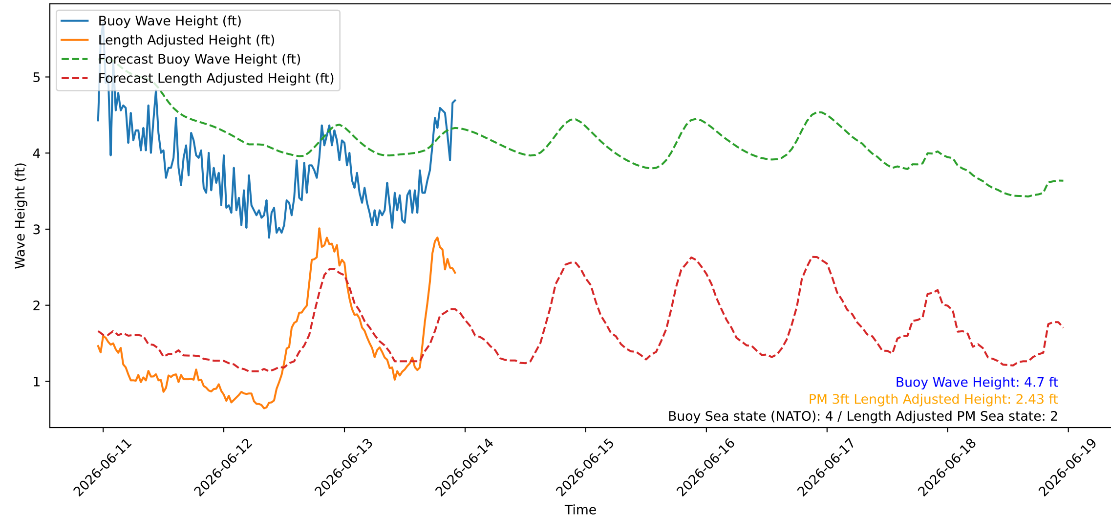
Wave Heights over Time for Green Beach at 2026-06-13 23:01:08
