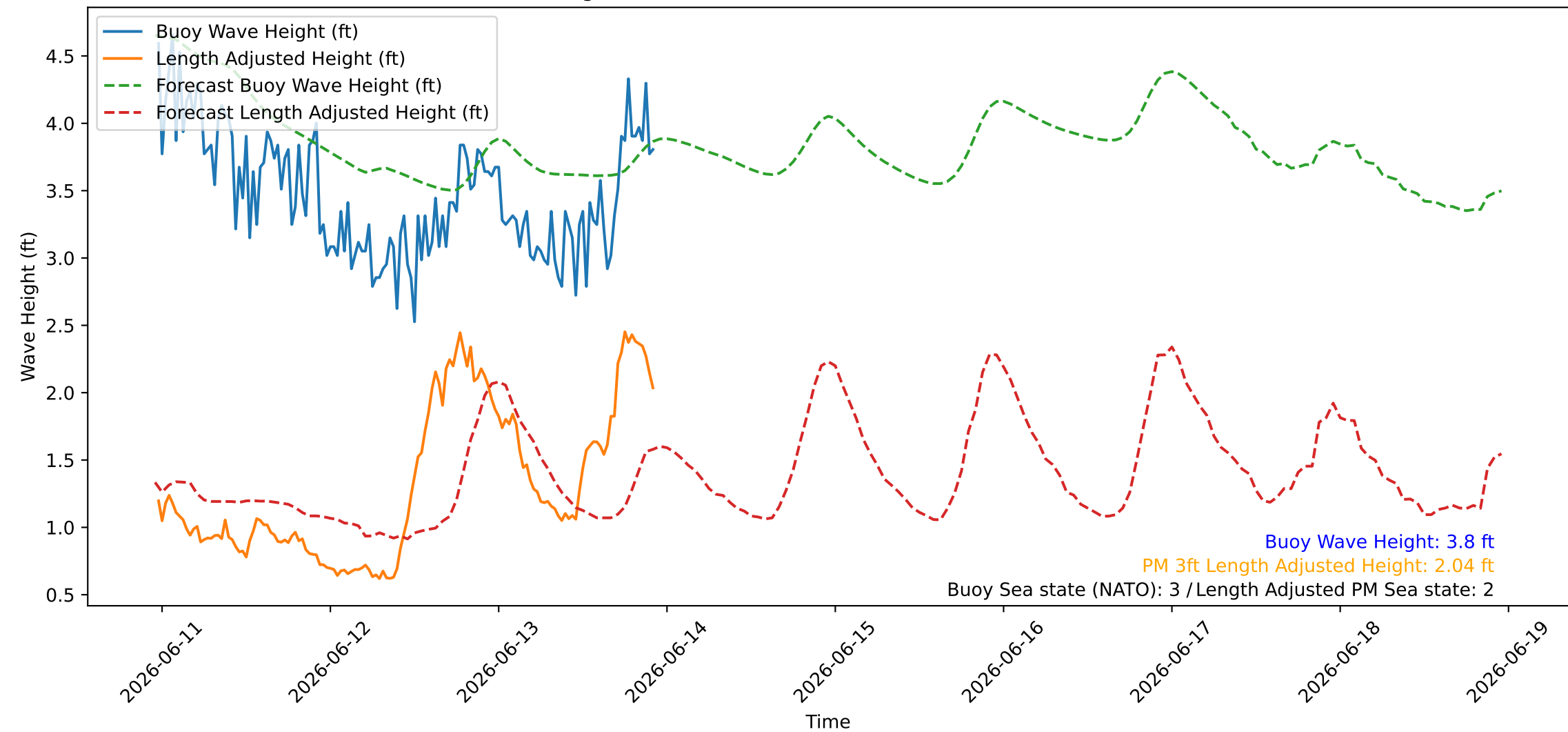
Wave Heights over Time for Red Beach at 2026-06-13 23:00:45
