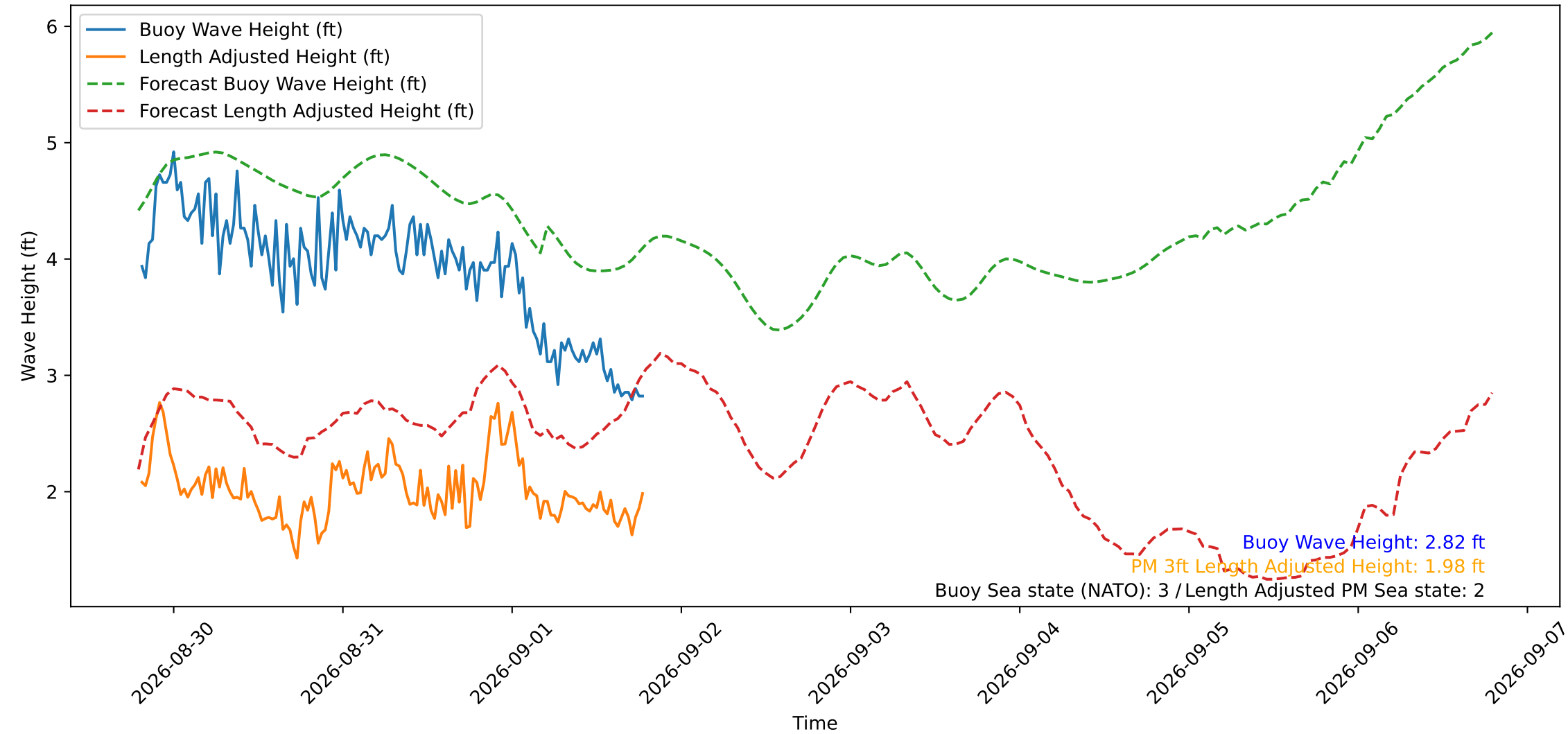
Wave Heights over Time for Green Beach at 2026-09-01 19:11:13
