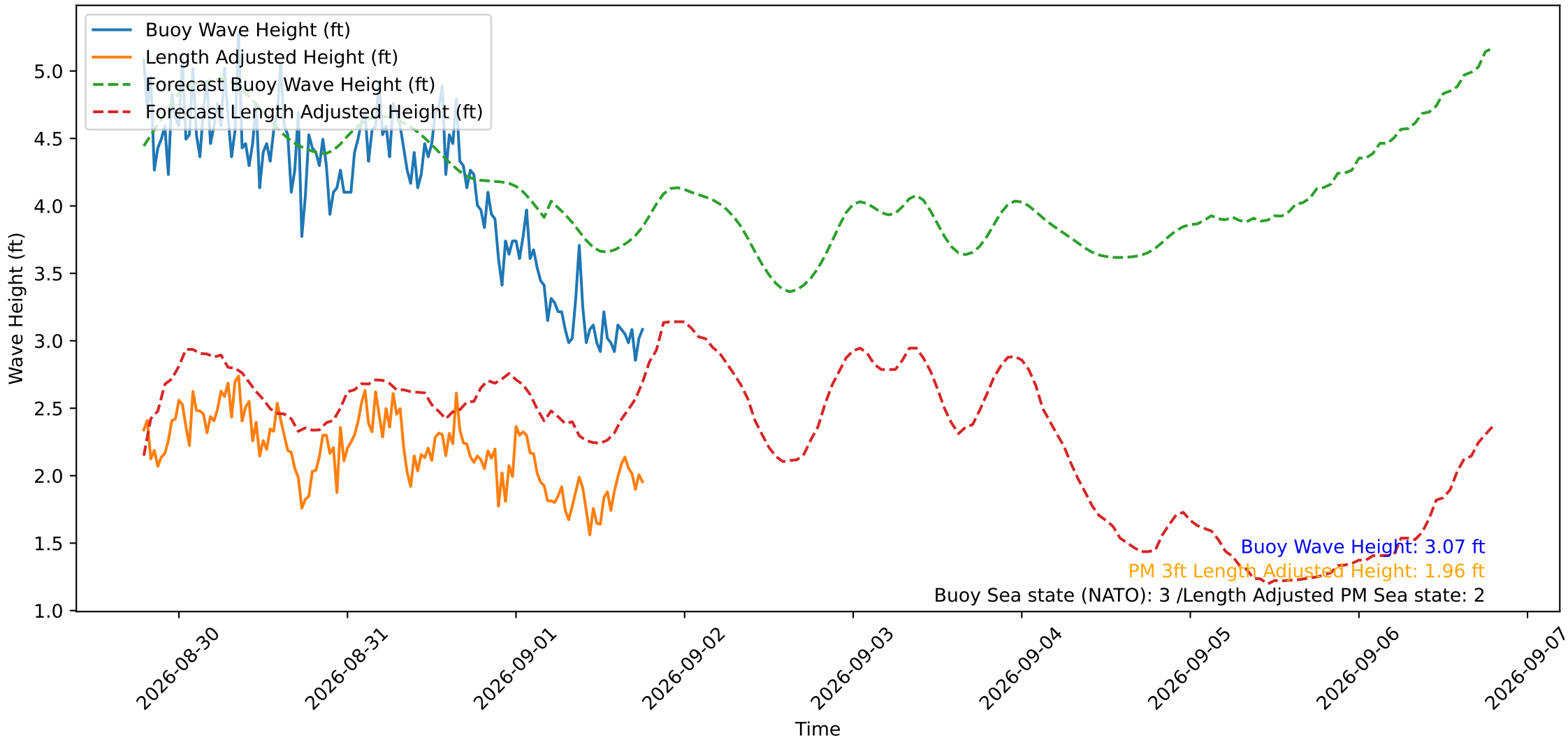
Wave Heights over Time for Oceanside Harbor at 2026-09-01 19:10:30
