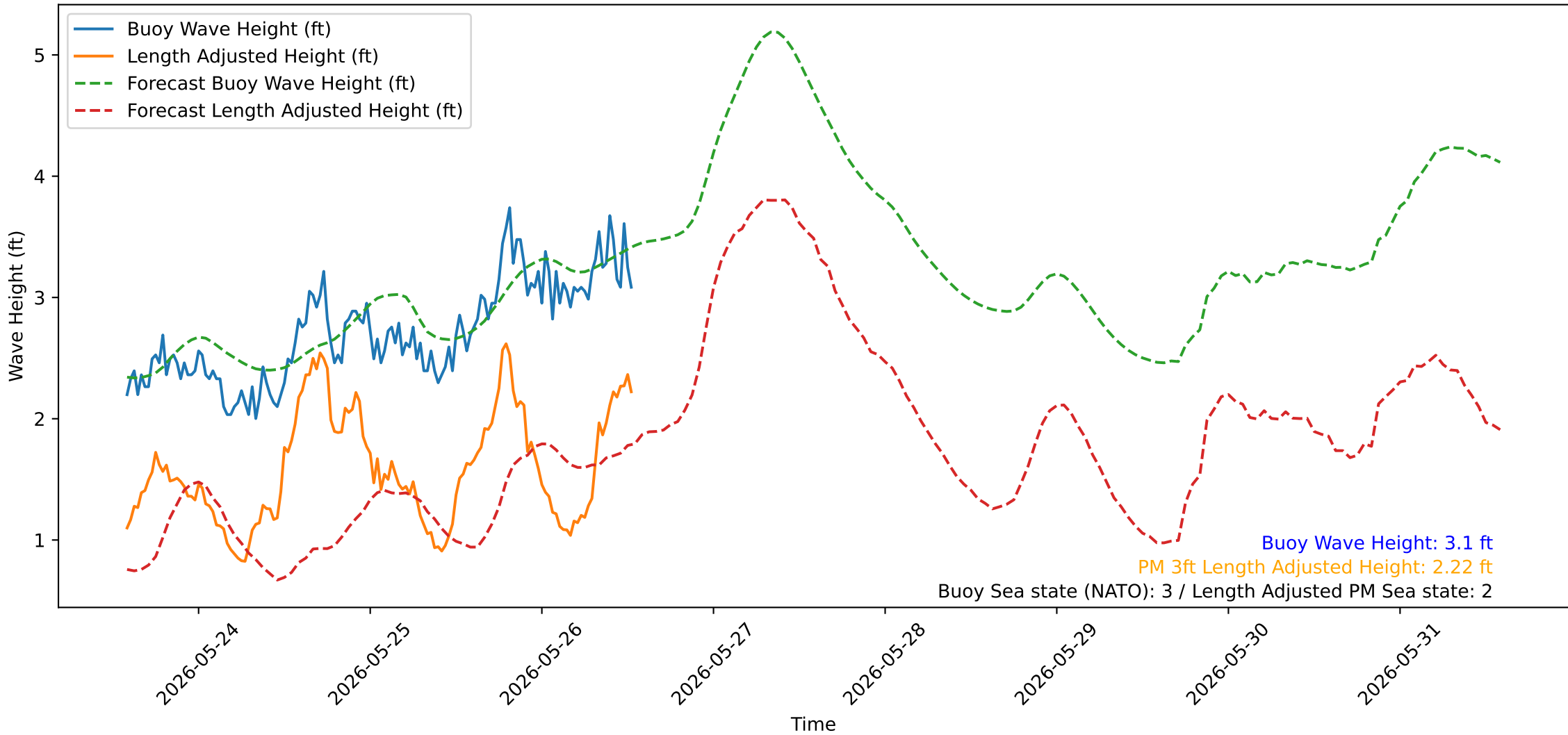
Wave Heights over Time for Red Beach at 2026-05-26 13:30:48
