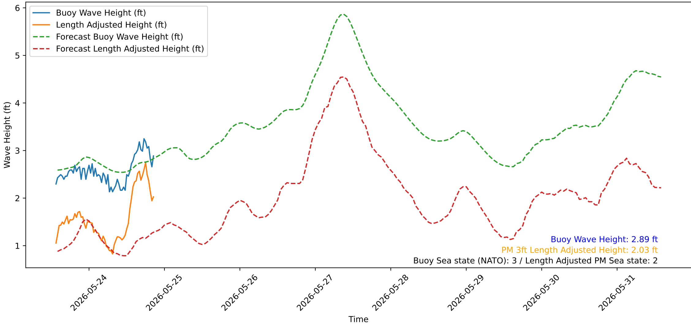
Wave Heights over Time for Oceanside Harbor at 2026-05-26 13:30:29
