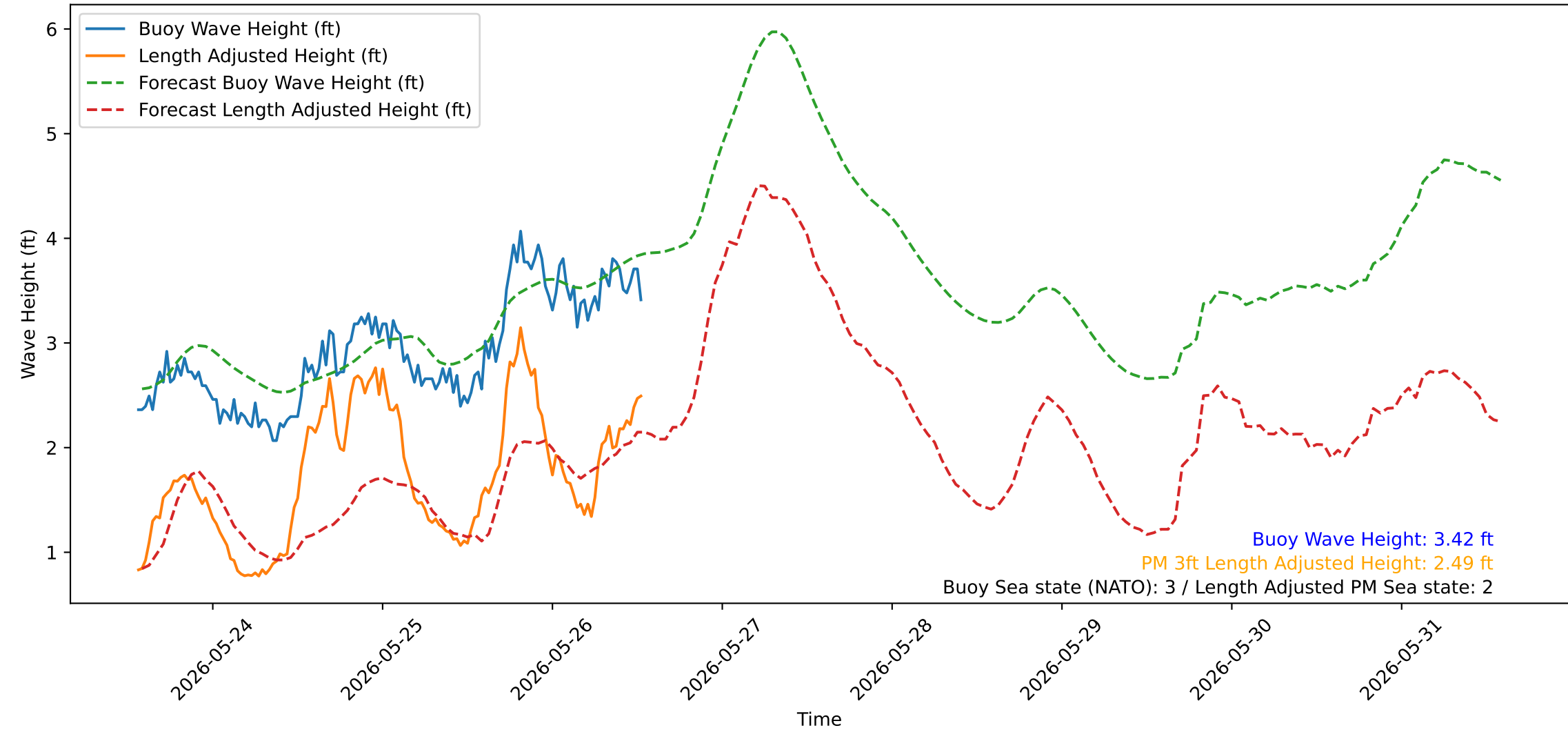
Wave Heights over Time for Green Beach at 2026-05-26 13:31:10
