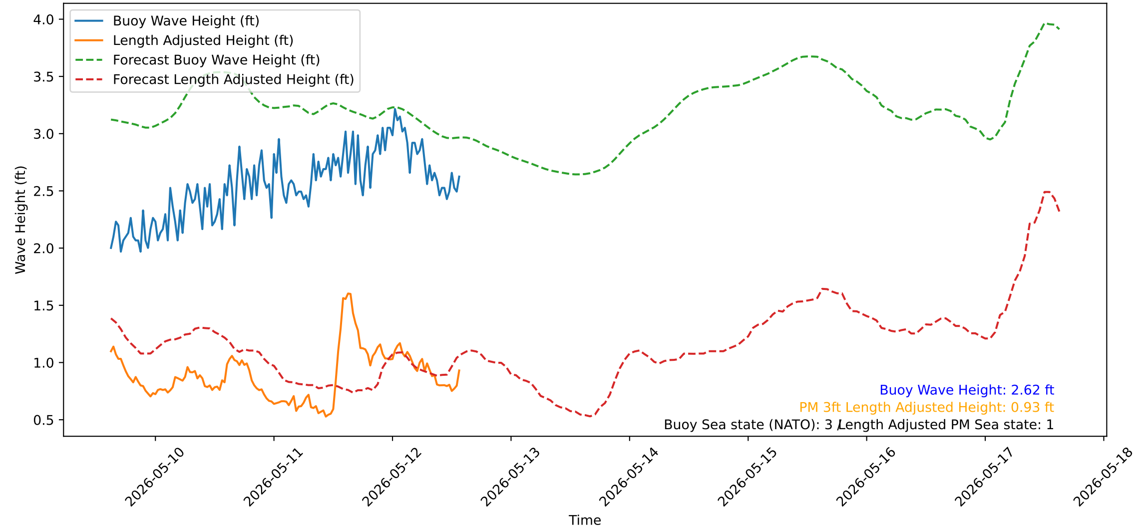
Wave Heights over Time for Red Beach at 2026-05-12 14:30:51
