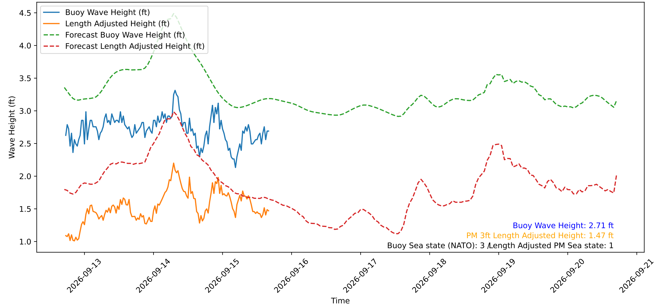
Wave Heights over Time for Green Beach at 2026-09-15 17:01:11
