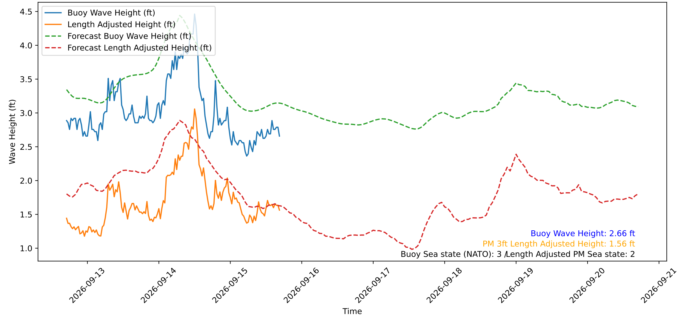
Wave Heights over Time for Oceanside Harbor at 2026-09-15 17:00:30
