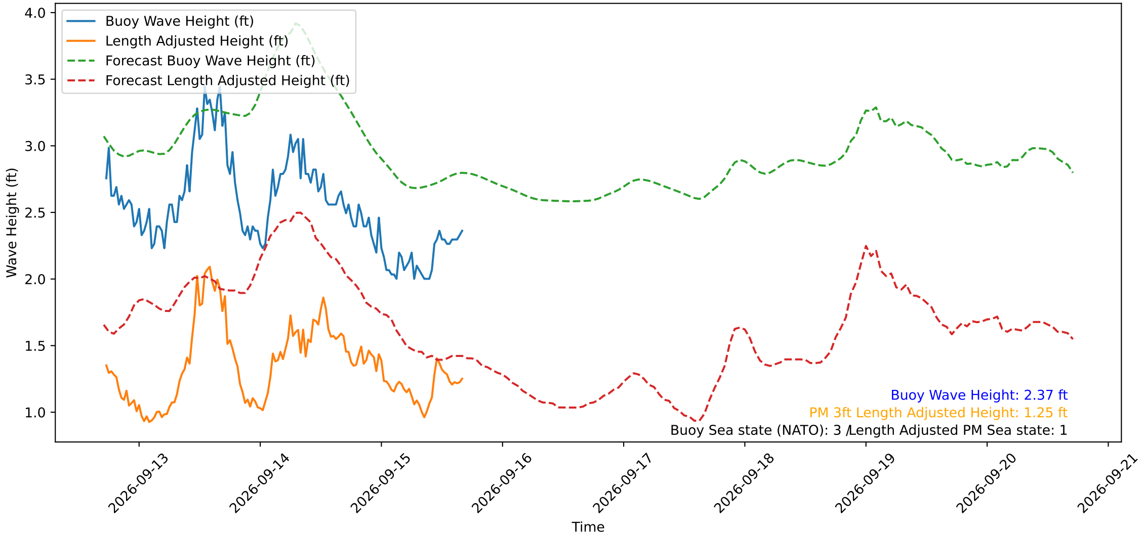
Wave Heights over Time for Red Beach at 2026-09-15 17:00:49
