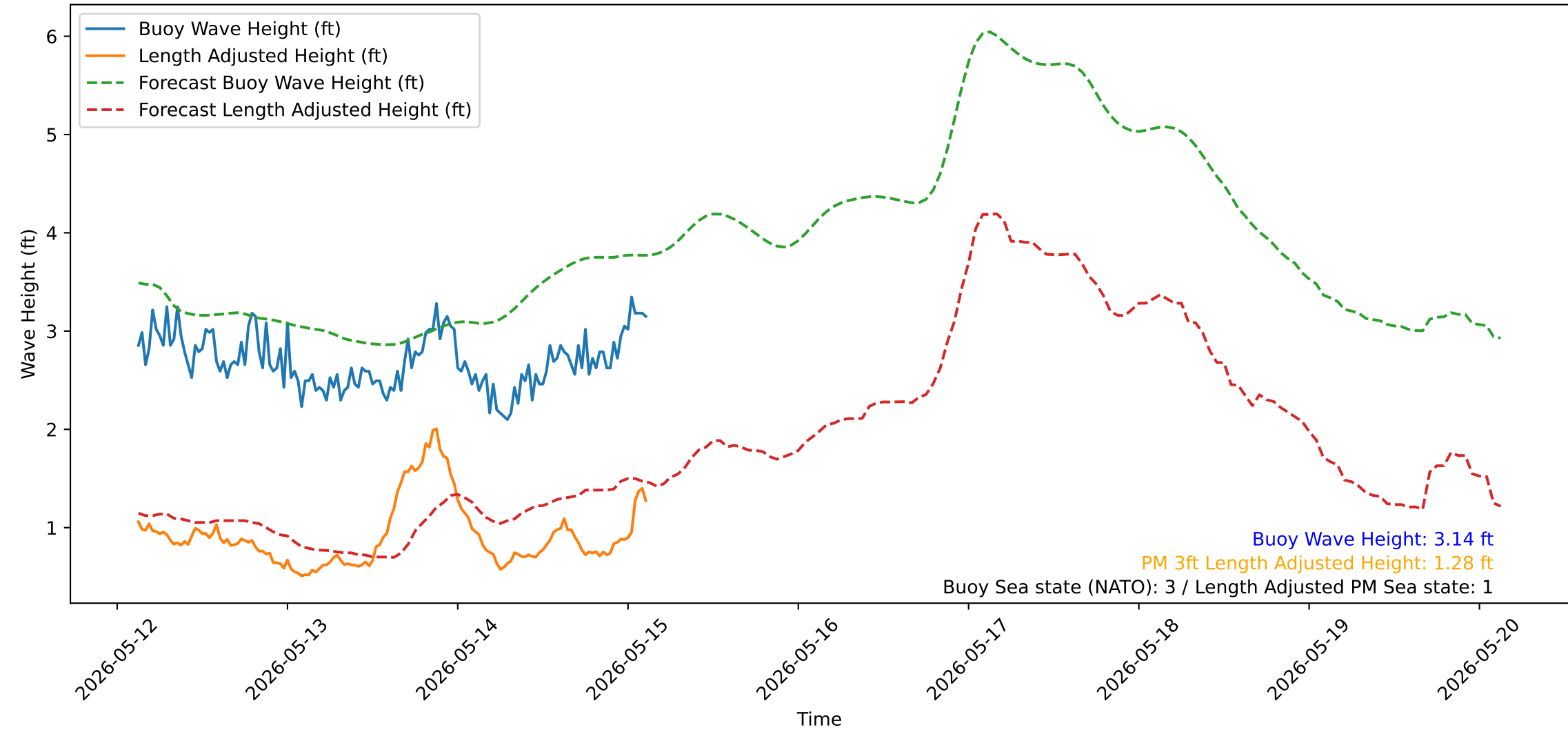
Wave Heights over Time for Green Beach at 2026-05-15 03:11:14
