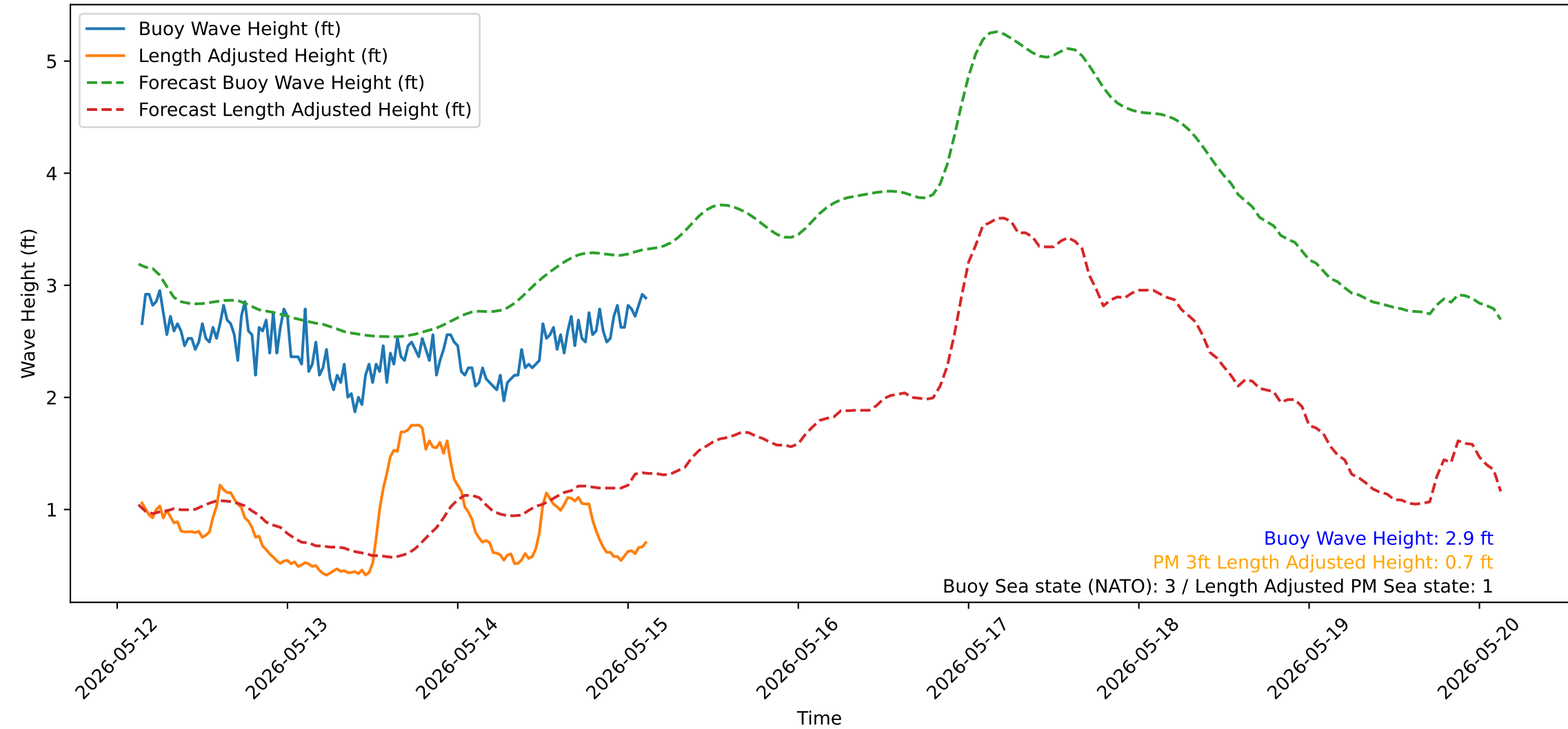
Wave Heights over Time for Red Beach at 2026-05-15 03:10:51
