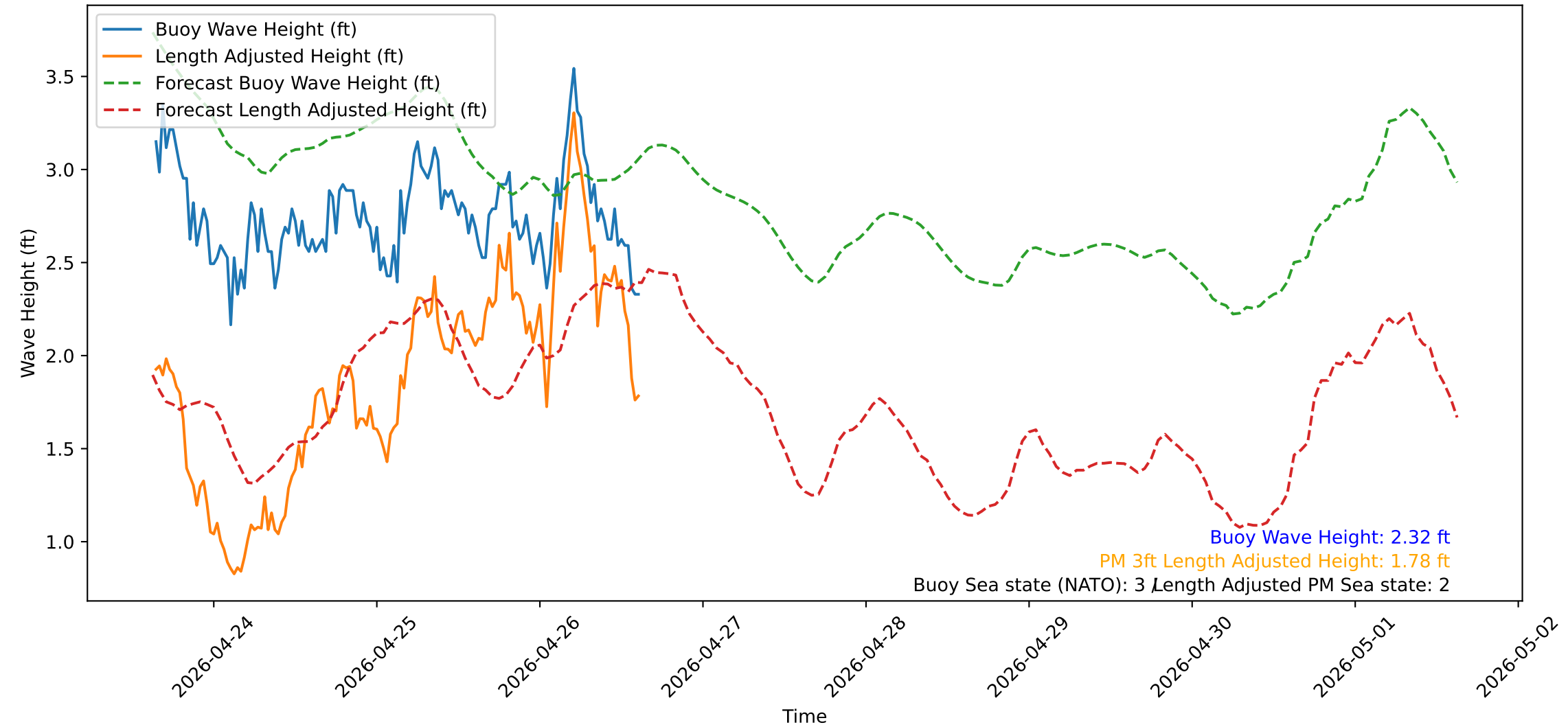
Wave Heights over Time for Red Beach at 2026-04-26 15:10:51
