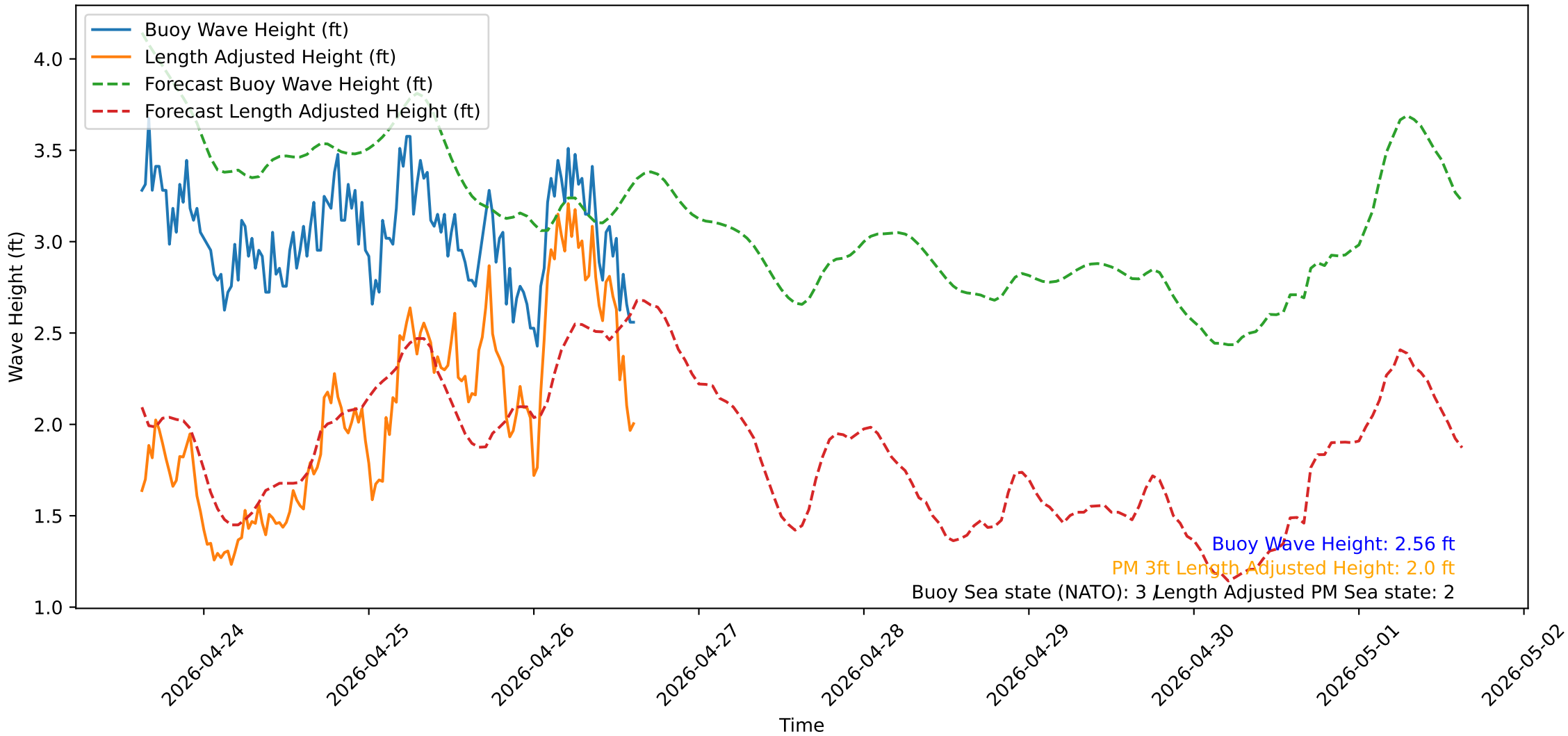
Wave Heights over Time for Green Beach at 2026-04-26 15:11:13
