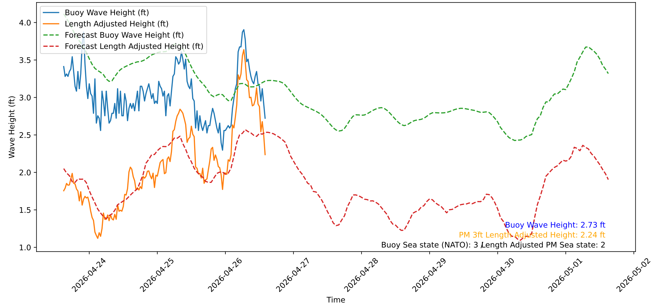
Wave Heights over Time for Oceanside Harbor at 2026-04-26 15:10:31
