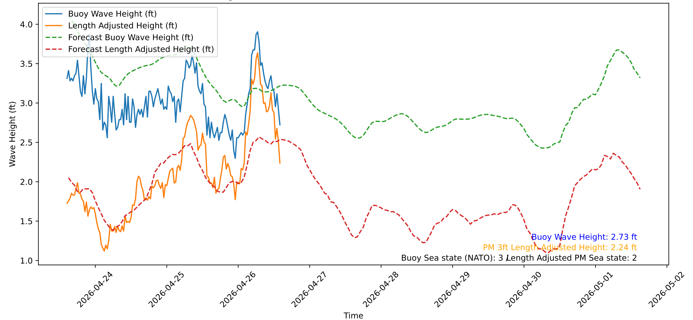
Wave Heights over Time for Oceanside Harbor at 2026-04-26 14:40:31
