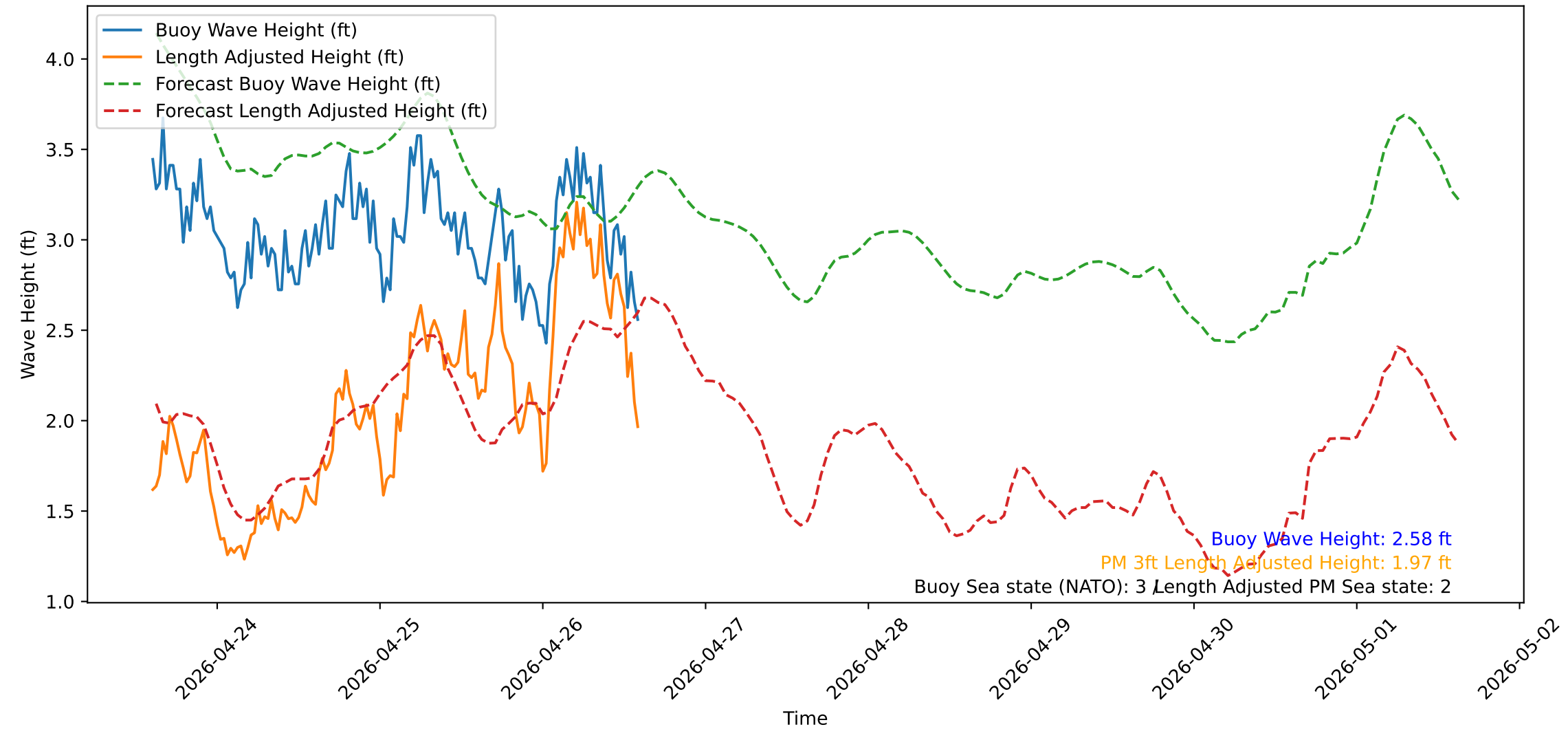
Wave Heights over Time for Green Beach at 2026-04-26 14:41:14
