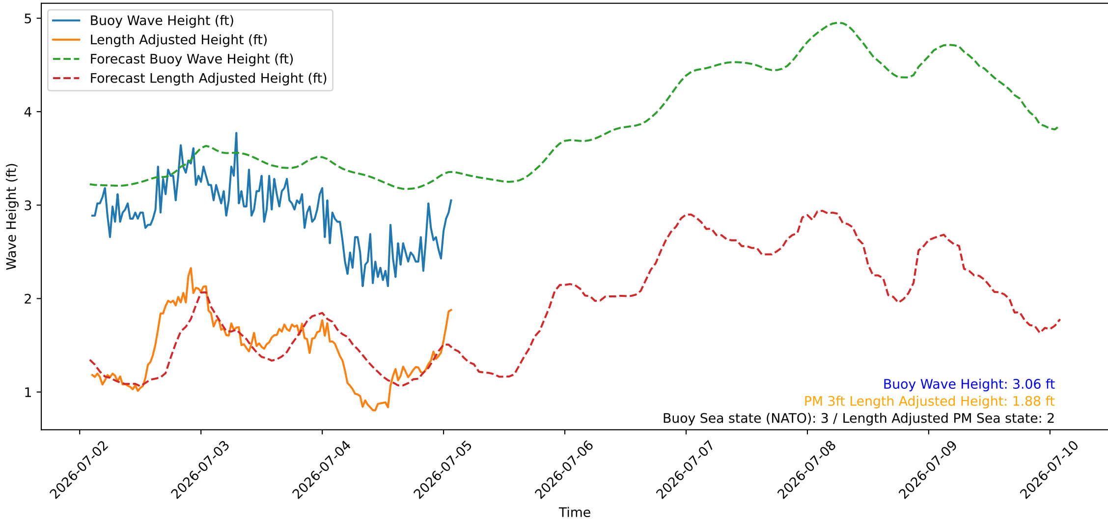
Wave Heights over Time for Oceanside Harbor at 2026-07-05 02:20:27
