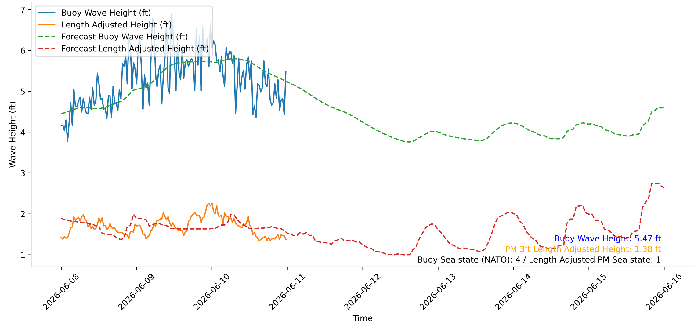
Wave Heights over Time for Green Beach at 2026-06-11 00:11:10
