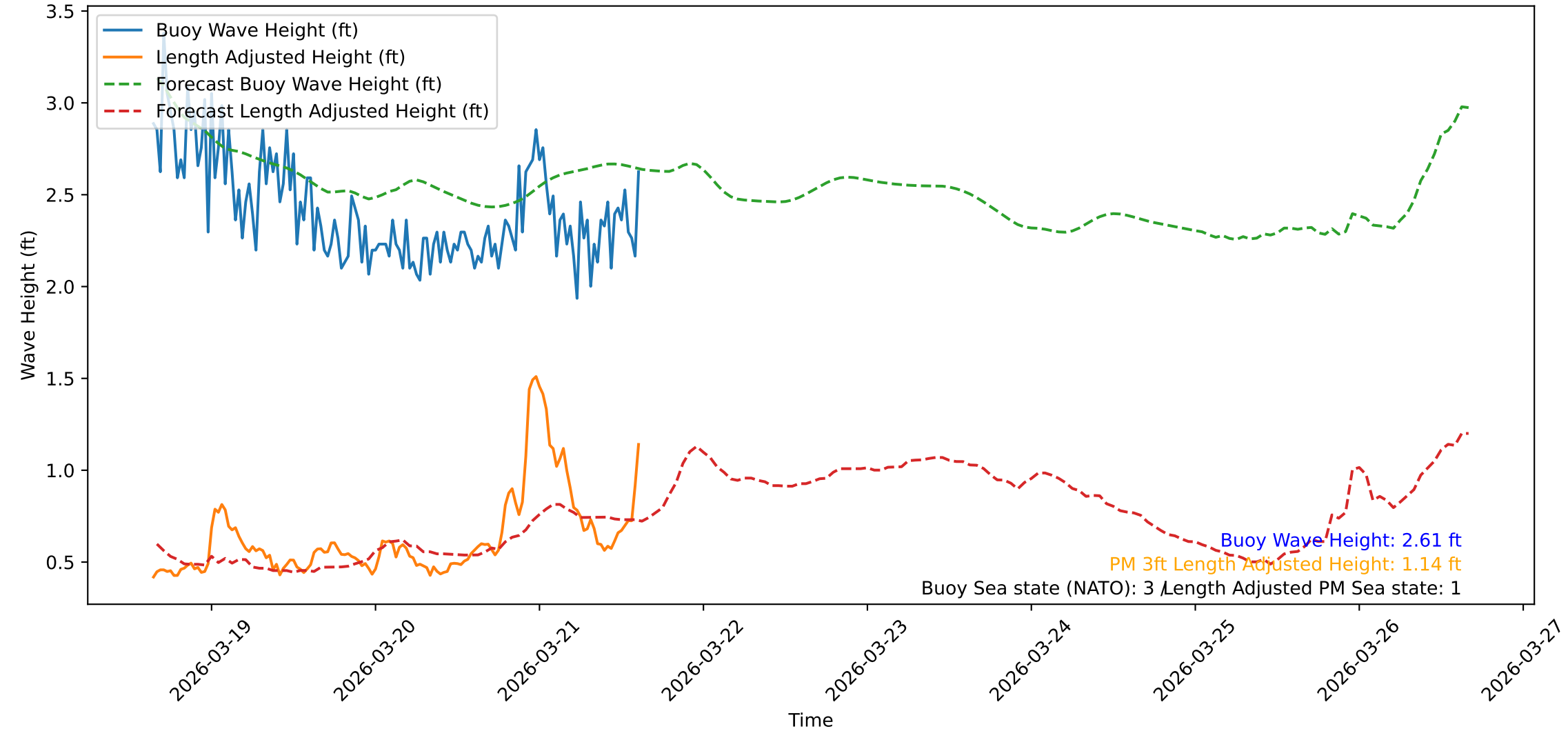
Wave Heights over Time for Green Beach at 2026-03-21 15:31:09
