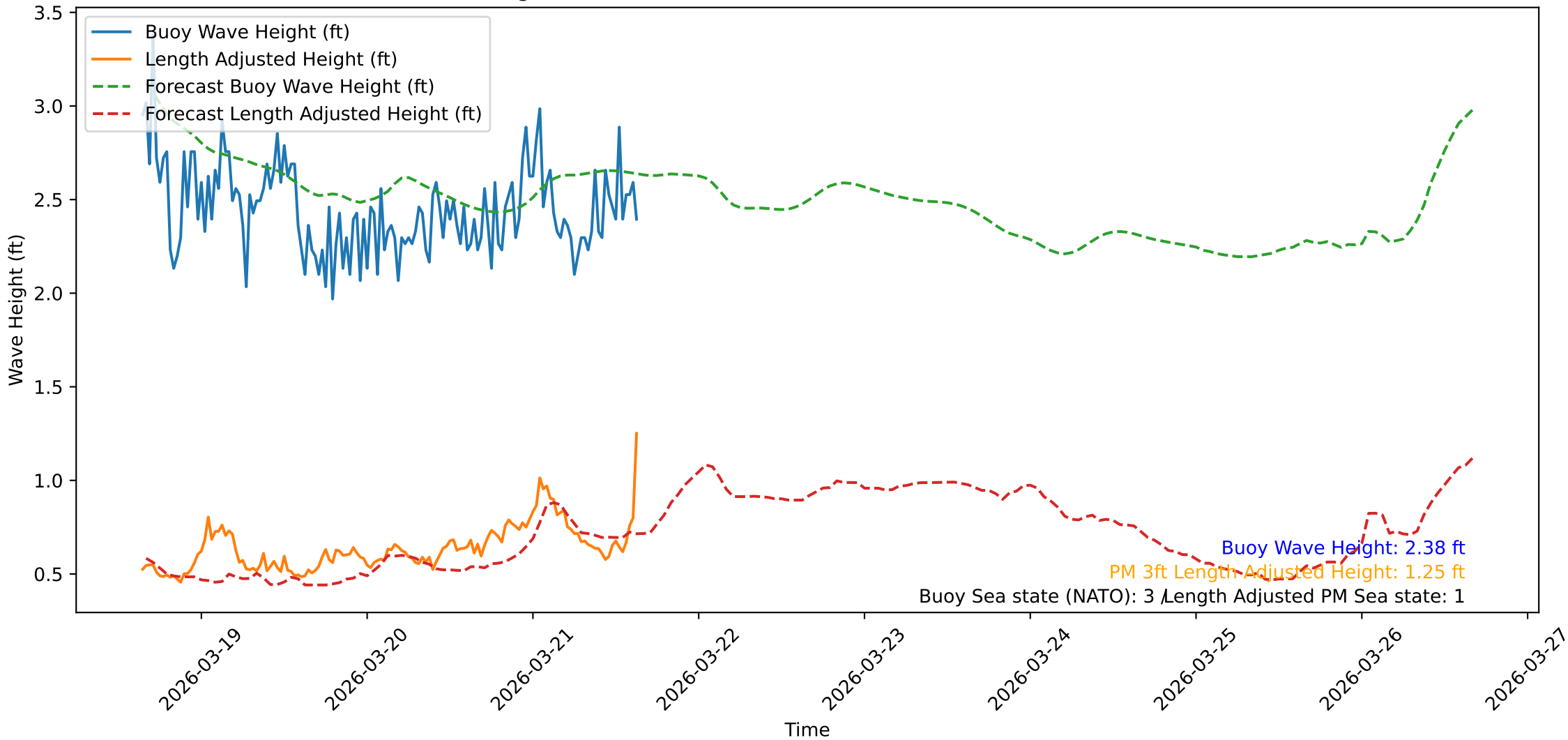
Wave Heights over Time for Oceanside Harbor at 2026-03-21 15:30:31
