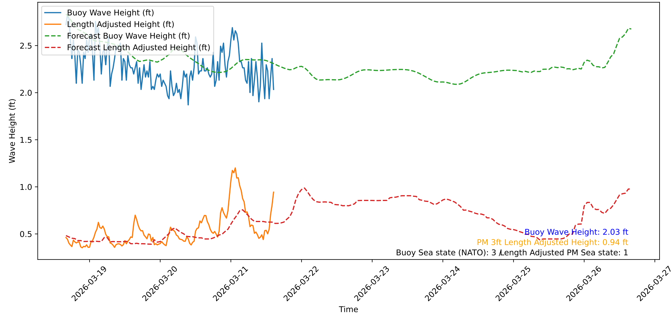
Wave Heights over Time for Red Beach at 2026-03-21 15:30:47
