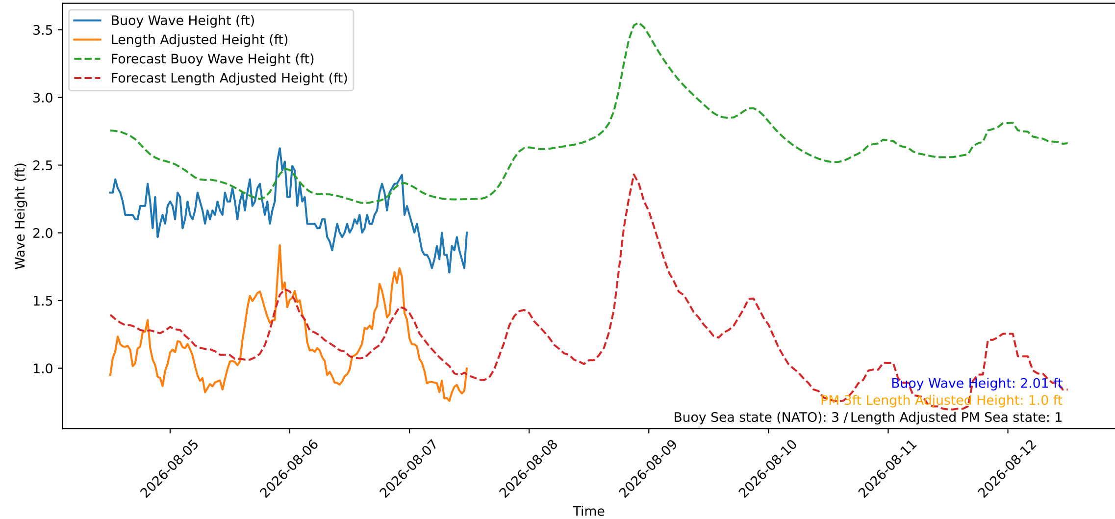
Wave Heights over Time for Green Beach at 2026-08-07 12:11:08
