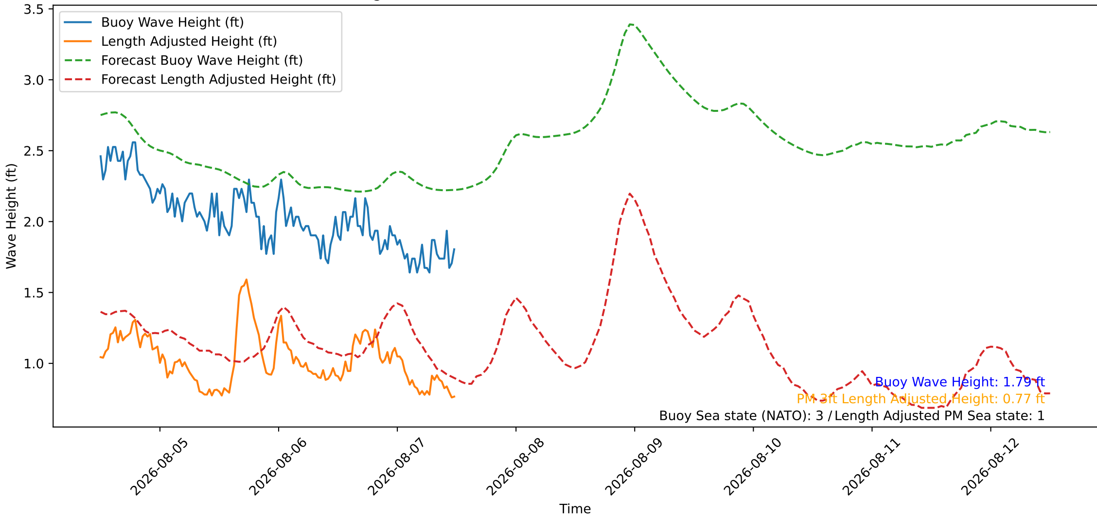
Wave Heights over Time for Oceanside Harbor at 2026-08-07 12:10:26
