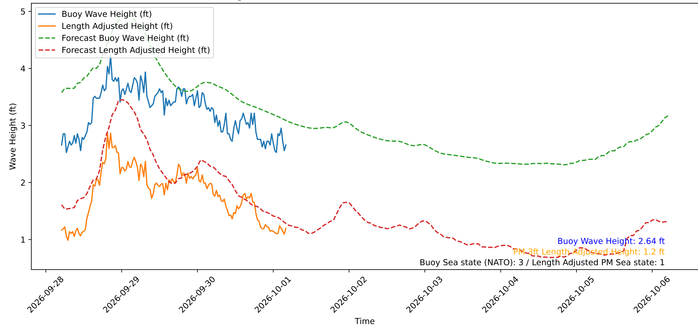
Wave Heights over Time for Oceanside Harbor at 2026-10-01 04:50:29
