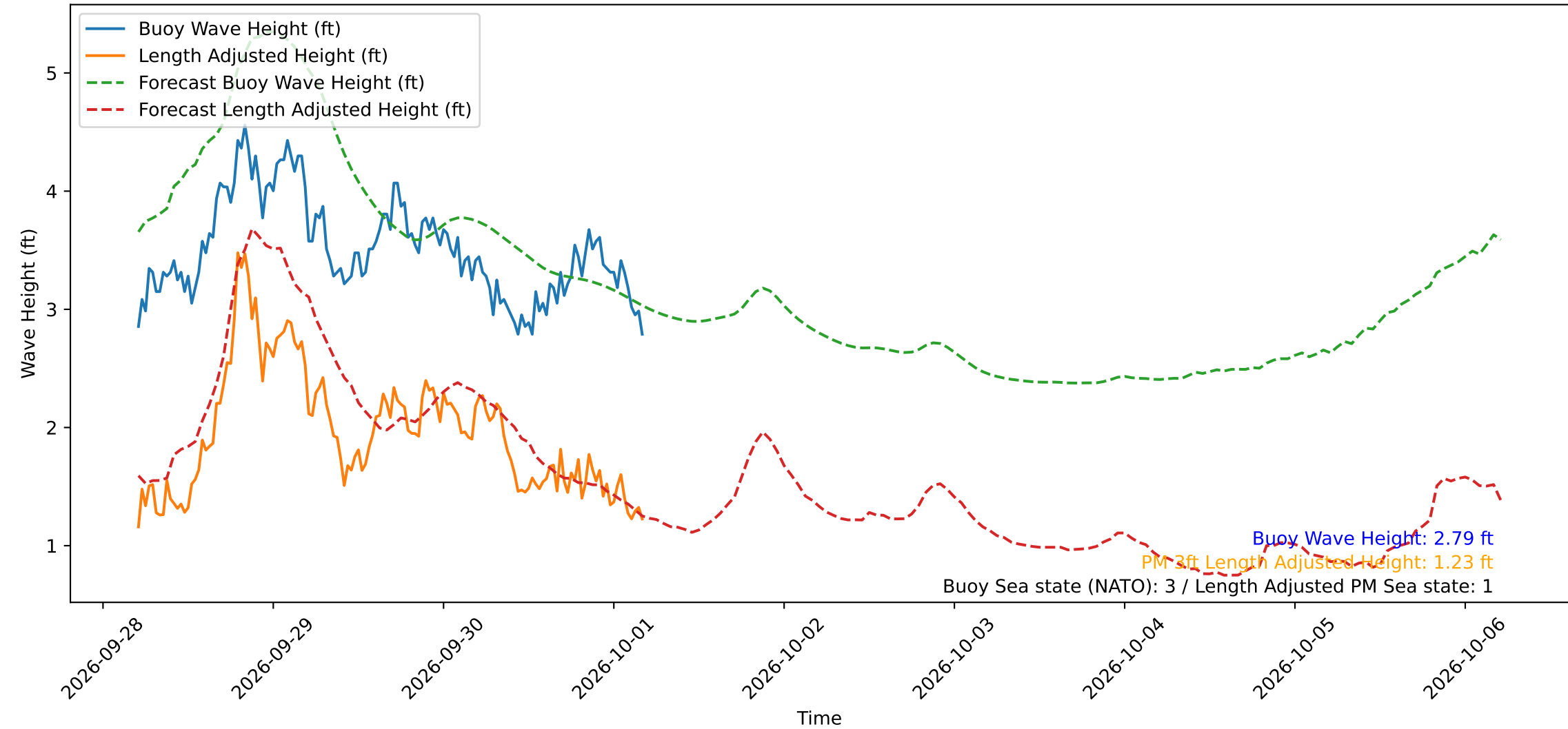
Wave Heights over Time for Green Beach at 2026-10-01 04:51:14
