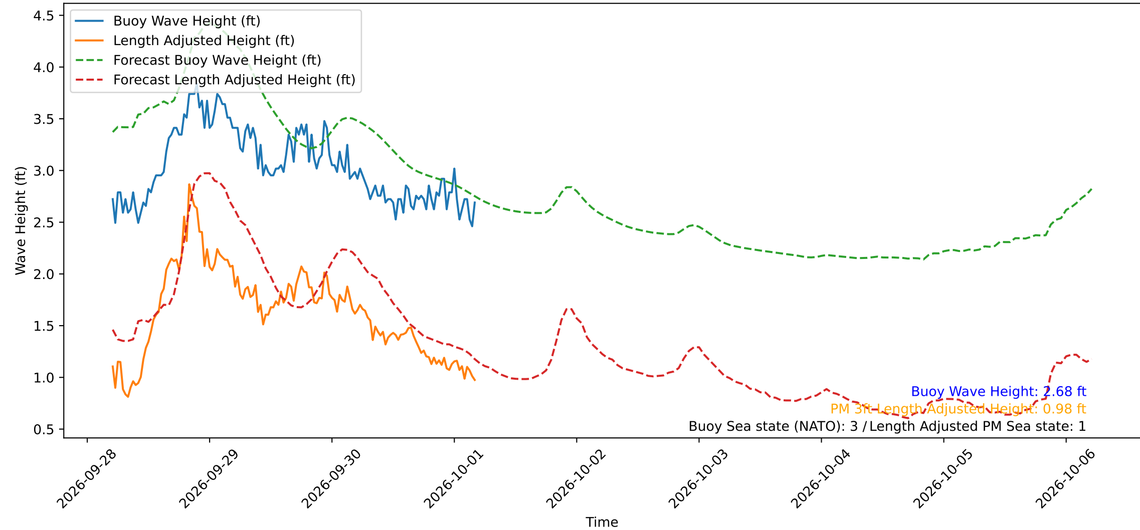
Wave Heights over Time for Red Beach at 2026-10-01 04:50:50
