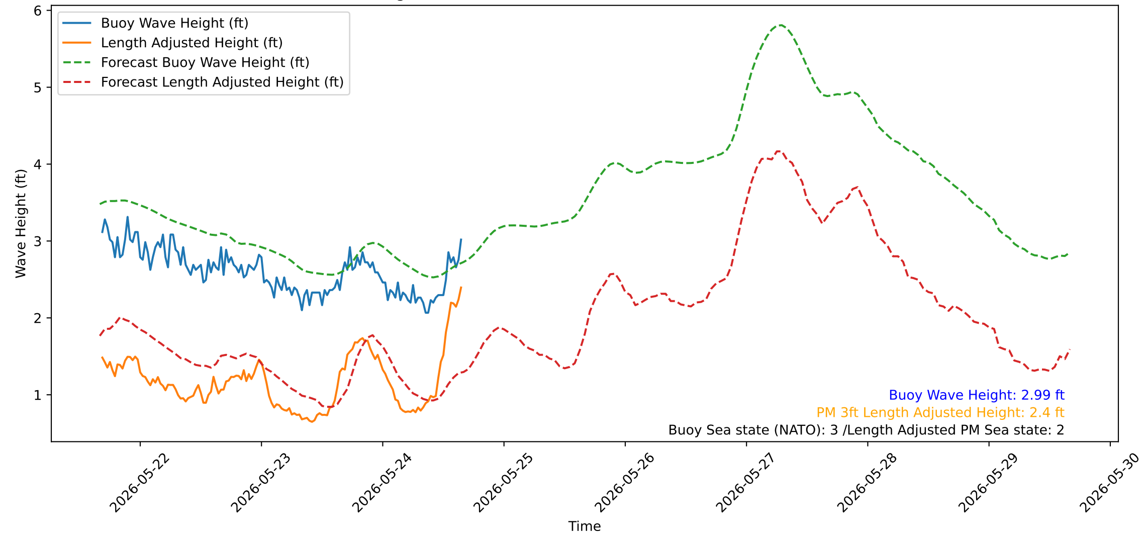
Wave Heights over Time for Green Beach at 2026-05-24 16:21:16
