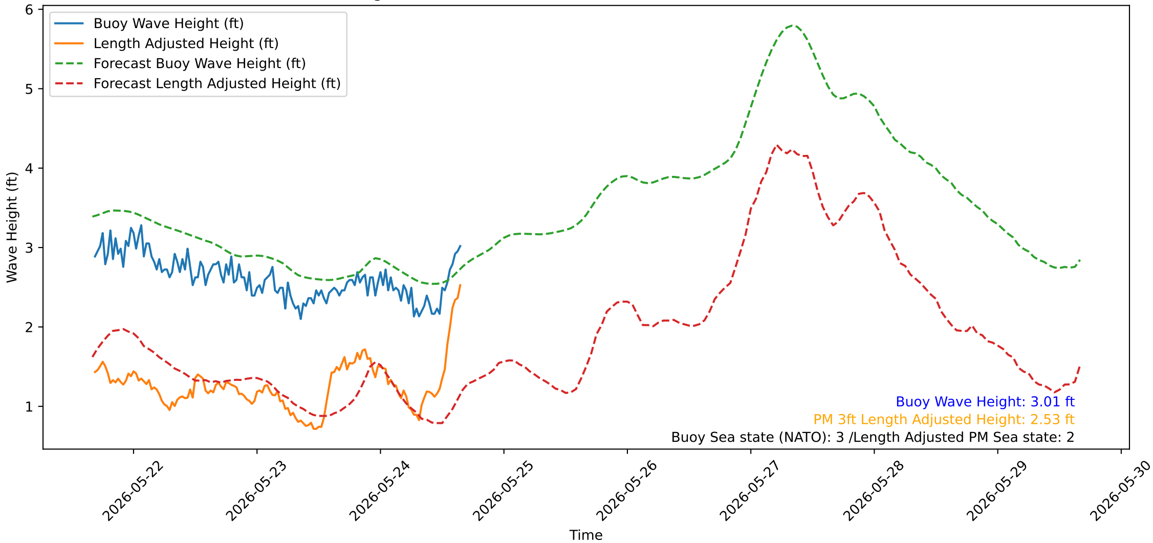
Wave Heights over Time for Oceanside Harbor at 2026-05-24 16:20:32
