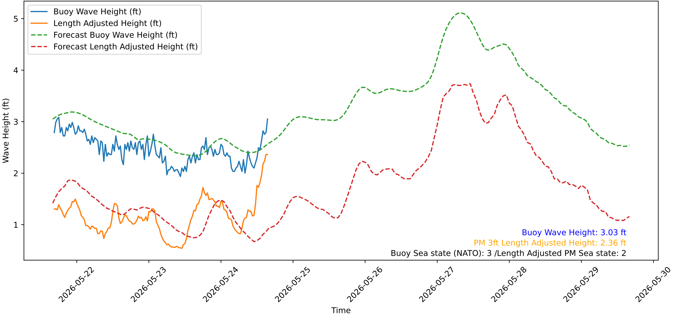
Wave Heights over Time for Red Beach at 2026-05-24 16:20:53
