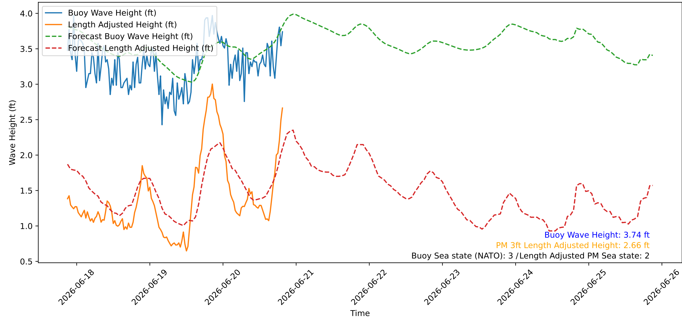
Wave Heights over Time for Green Beach at 2026-06-20 21:01:07
