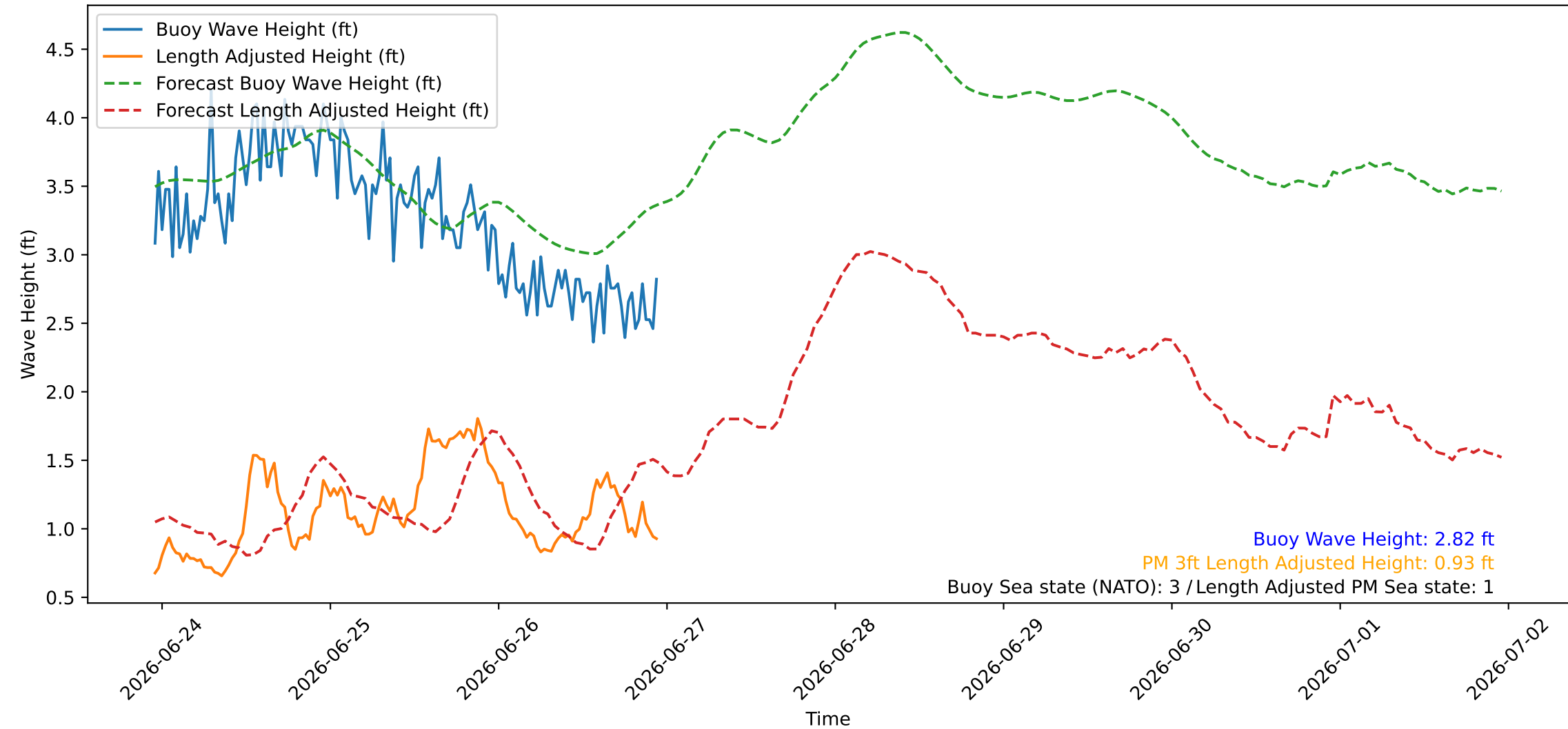
Wave Heights over Time for Green Beach at 2026-06-26 23:11:08
