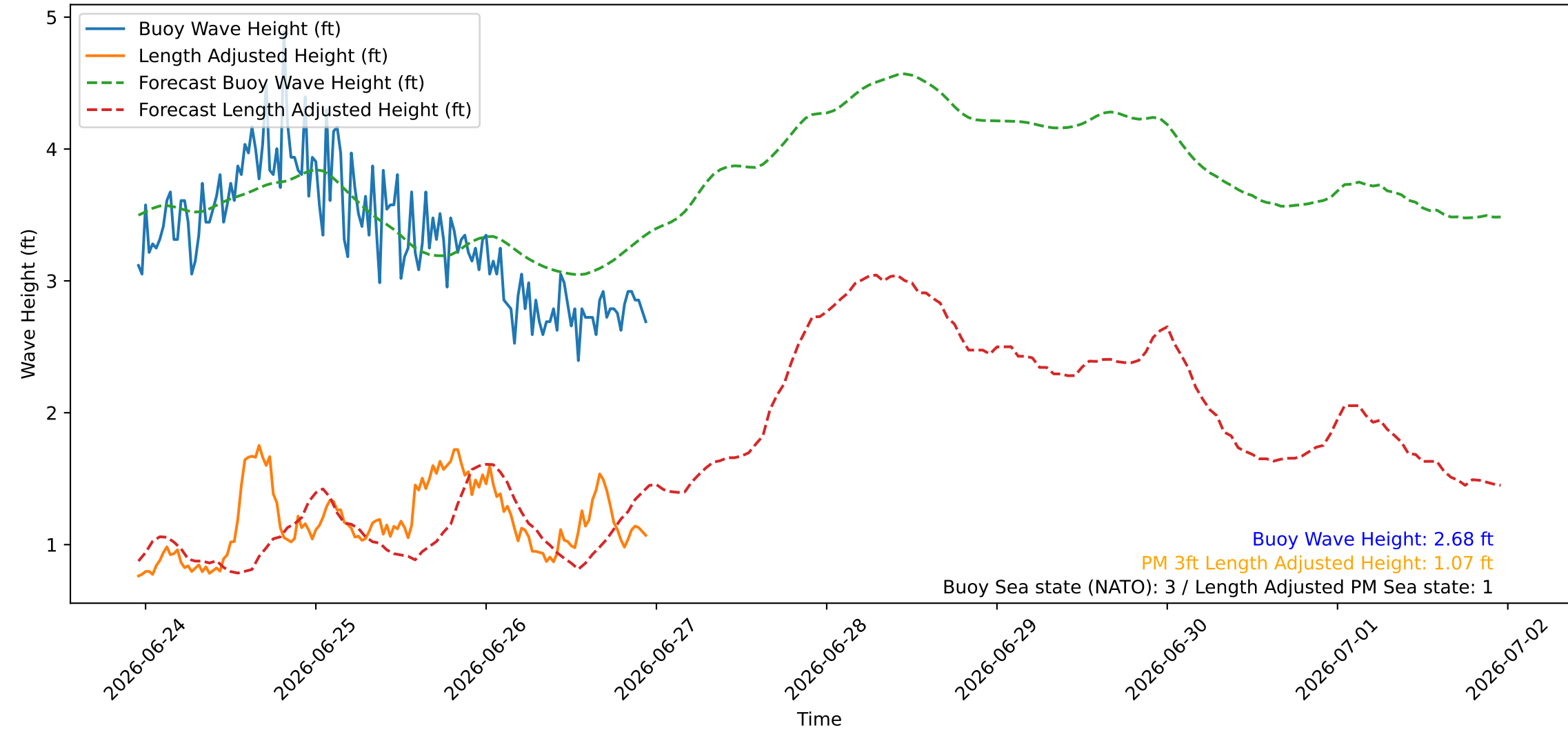
Wave Heights over Time for Oceanside Harbor at 2026-06-26 23:10:26
