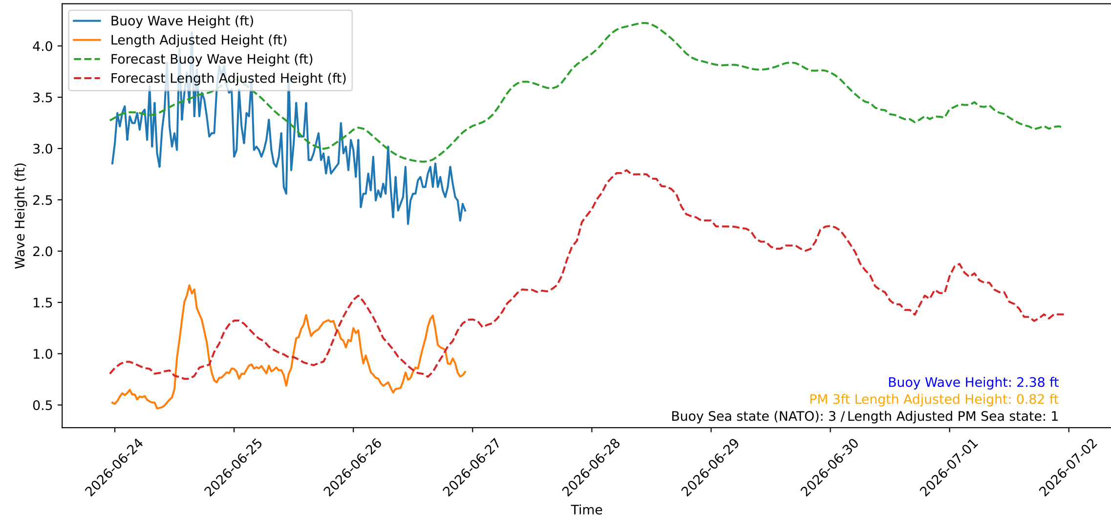
Wave Heights over Time for Red Beach at 2026-06-26 23:10:45
