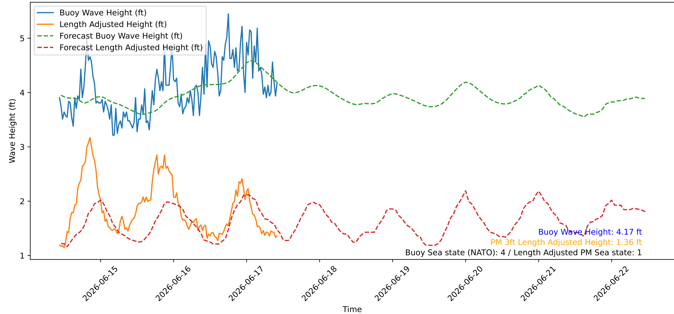
Wave Heights over Time for Oceanside Harbor at 2026-06-17 10:40:27
