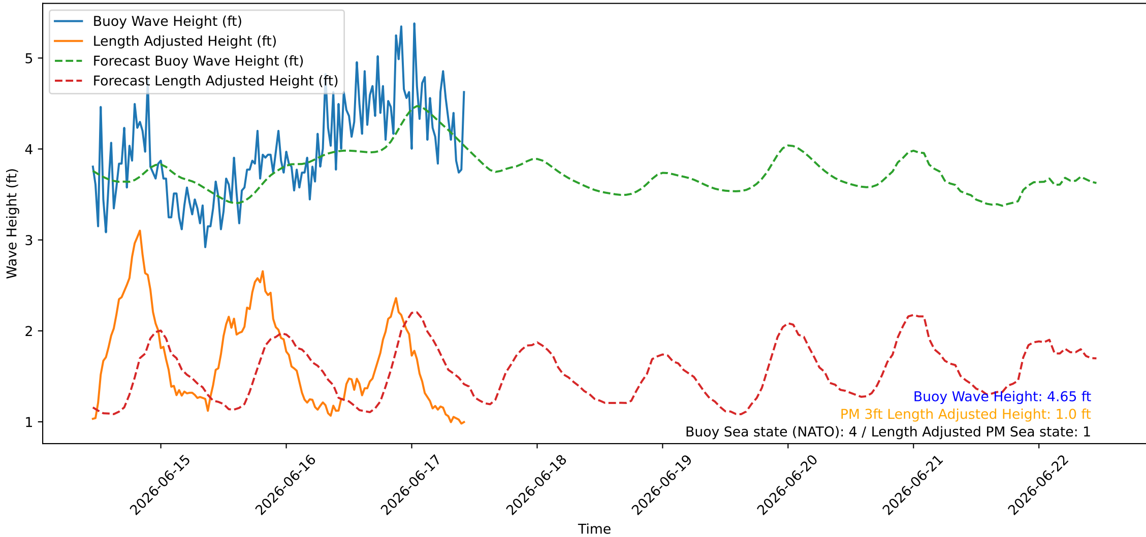
Wave Heights over Time for Red Beach at 2026-06-17 10:40:46
