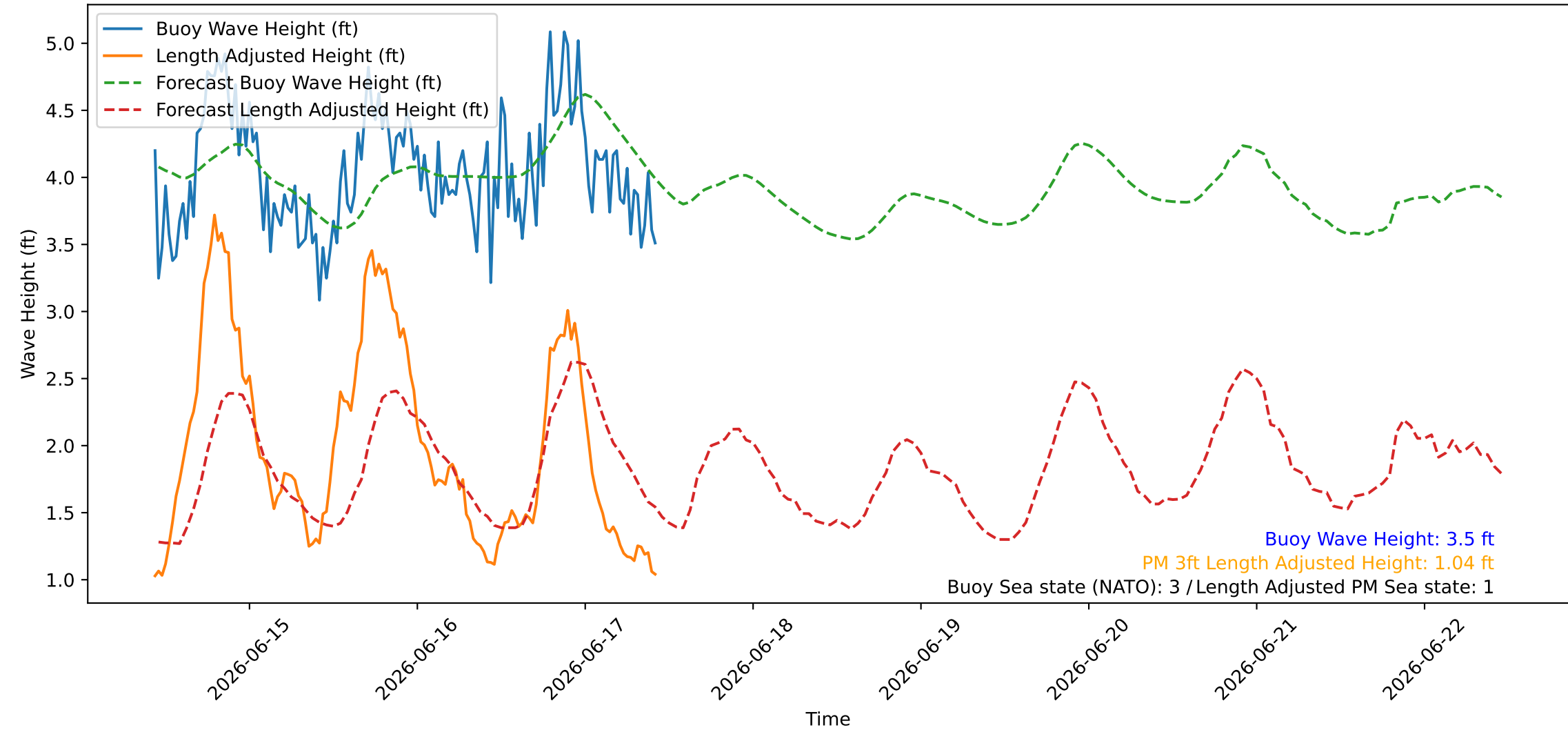
Wave Heights over Time for Green Beach at 2026-06-17 10:41:09
