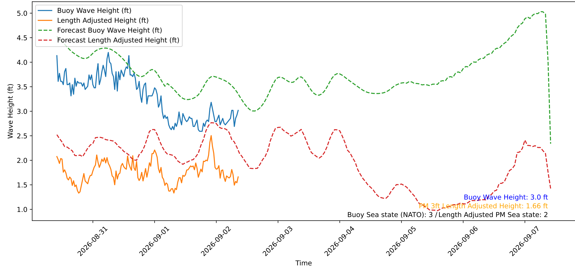
Wave Heights over Time for Red Beach at 2026-09-02 09:30:49
