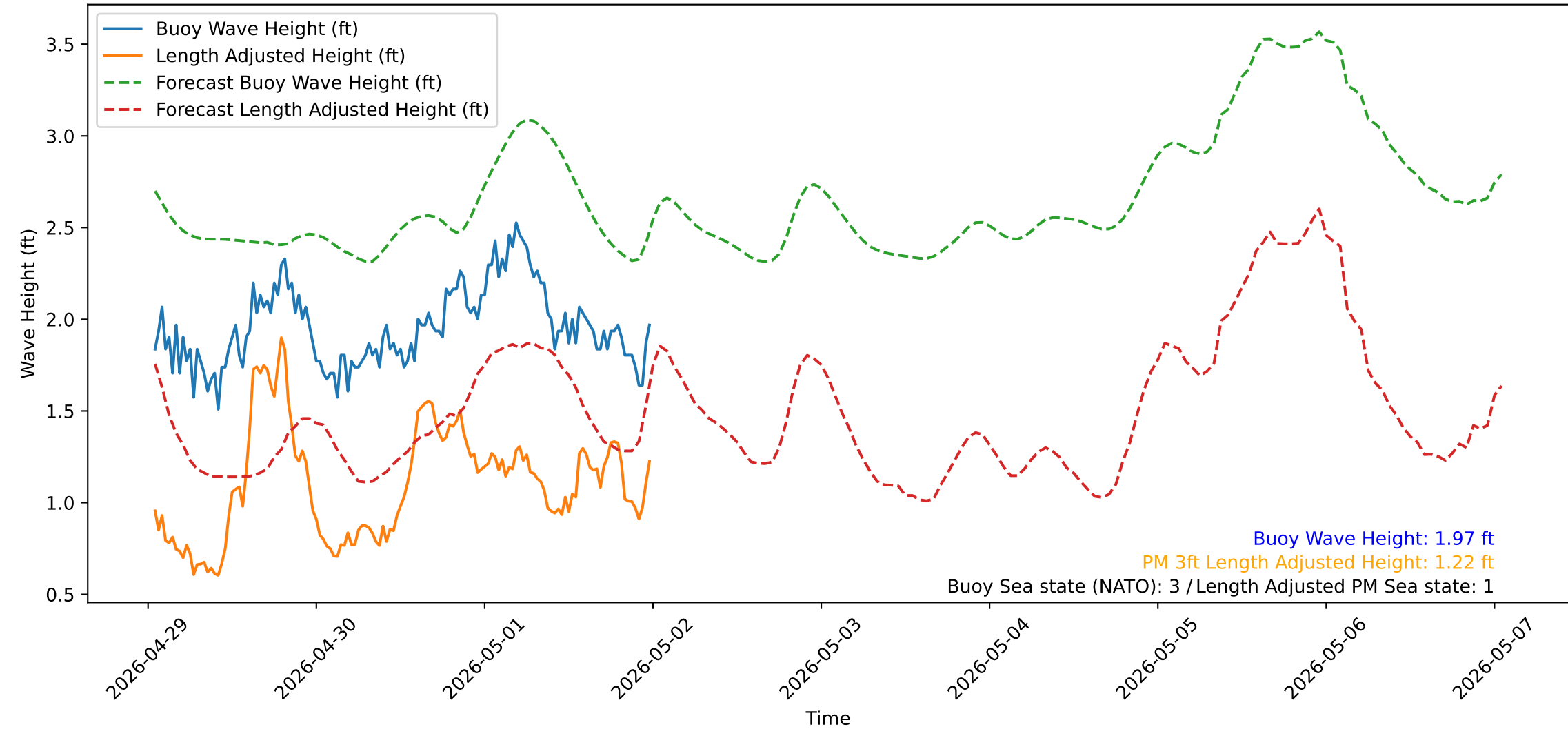
Wave Heights over Time for Red Beach at 2026-05-02 00:30:51
