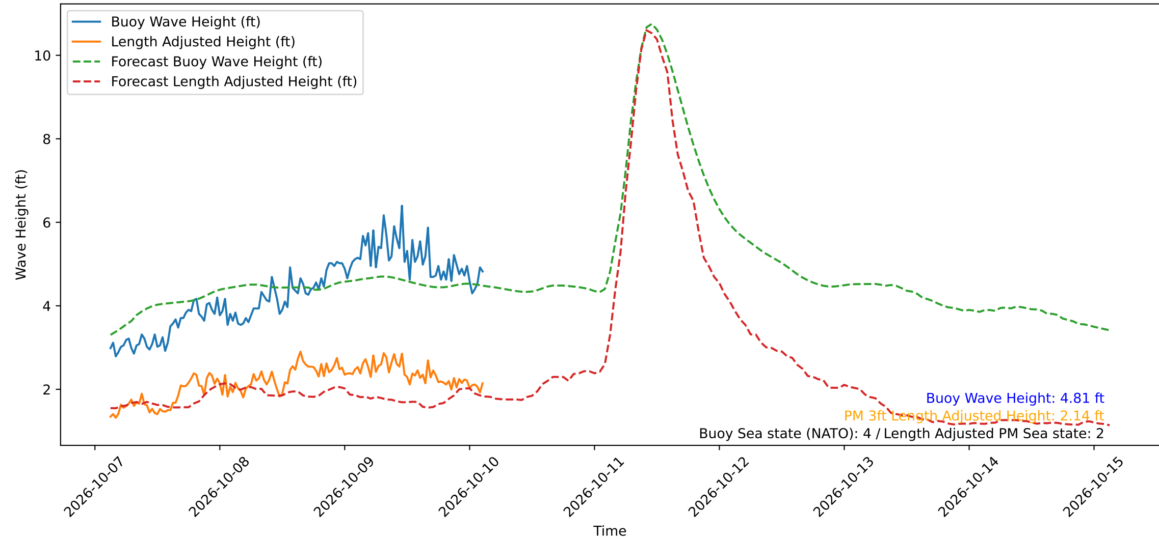
Wave Heights over Time for Oceanside Harbor at 2026-10-10 03:10:29
