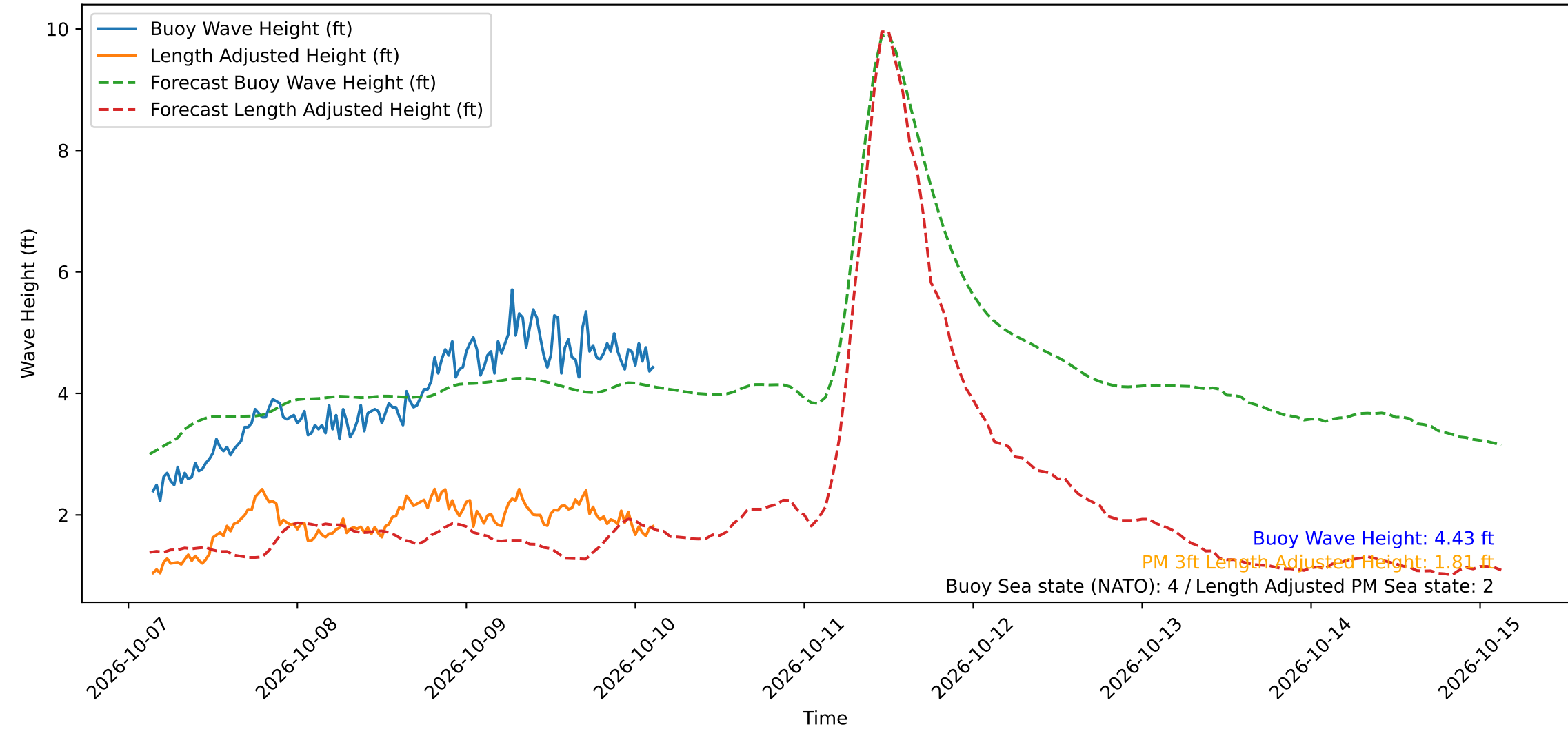
Wave Heights over Time for Red Beach at 2026-10-10 03:10:49
