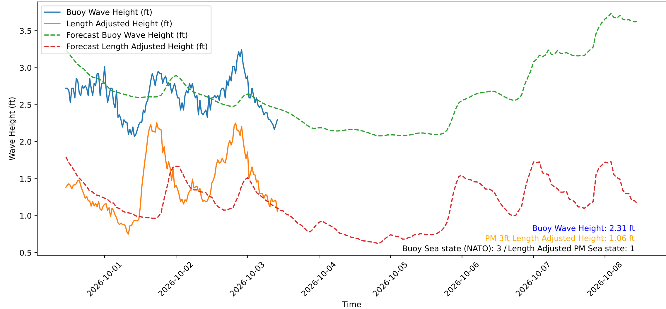
Wave Heights over Time for Red Beach at 2026-10-03 10:50:52
