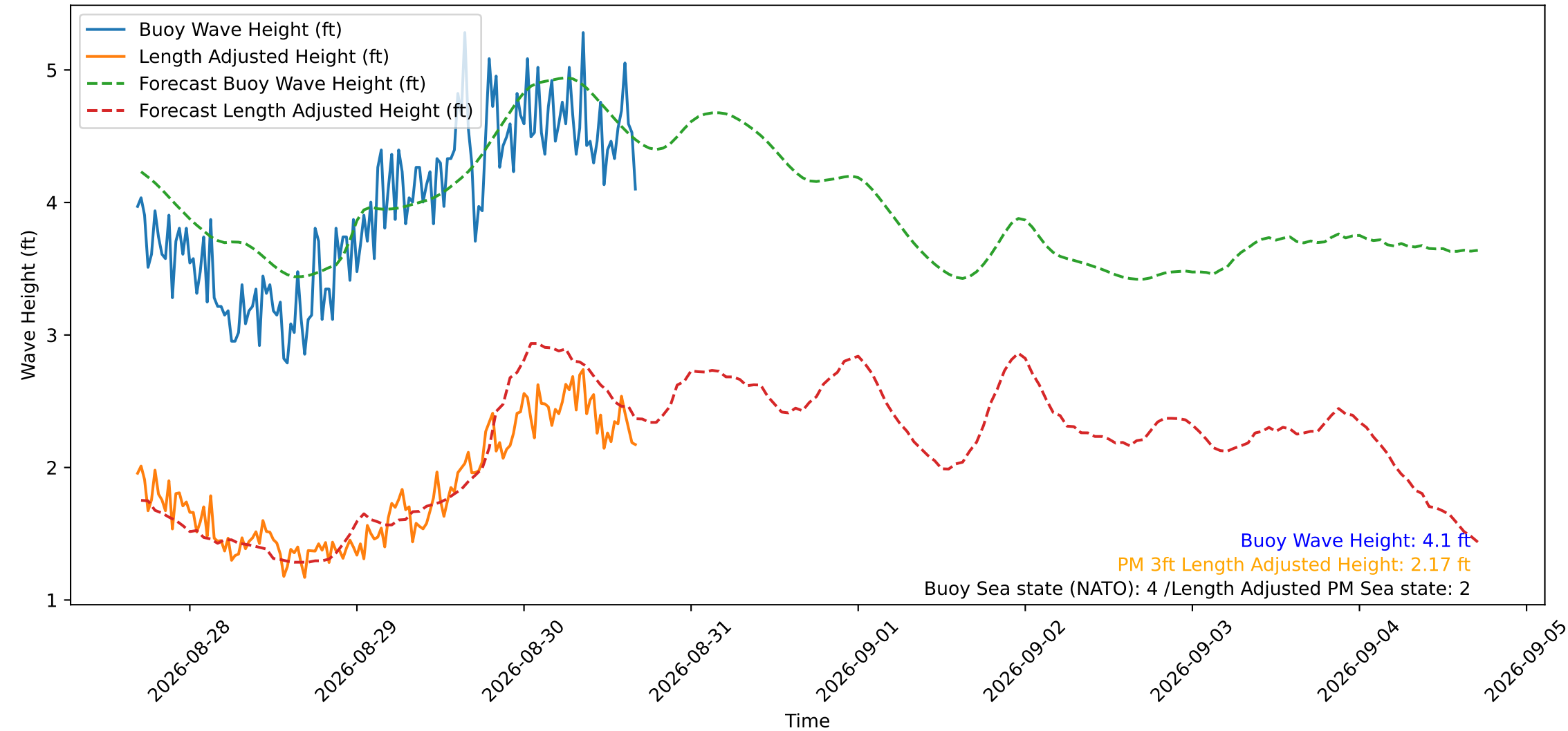
Wave Heights over Time for Oceanside Harbor at 2026-08-30 16:30:29
