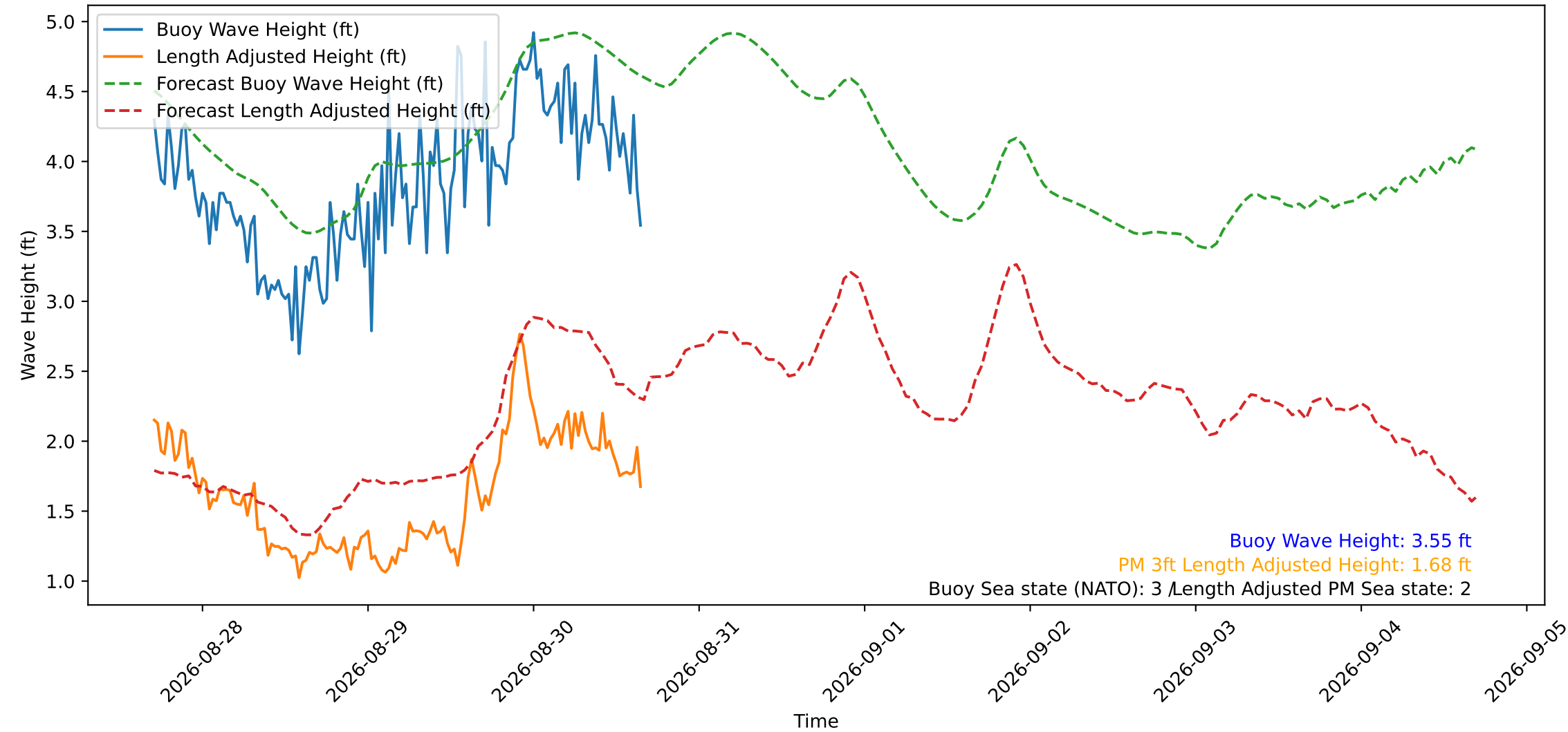
Wave Heights over Time for Green Beach at 2026-08-30 16:31:12
