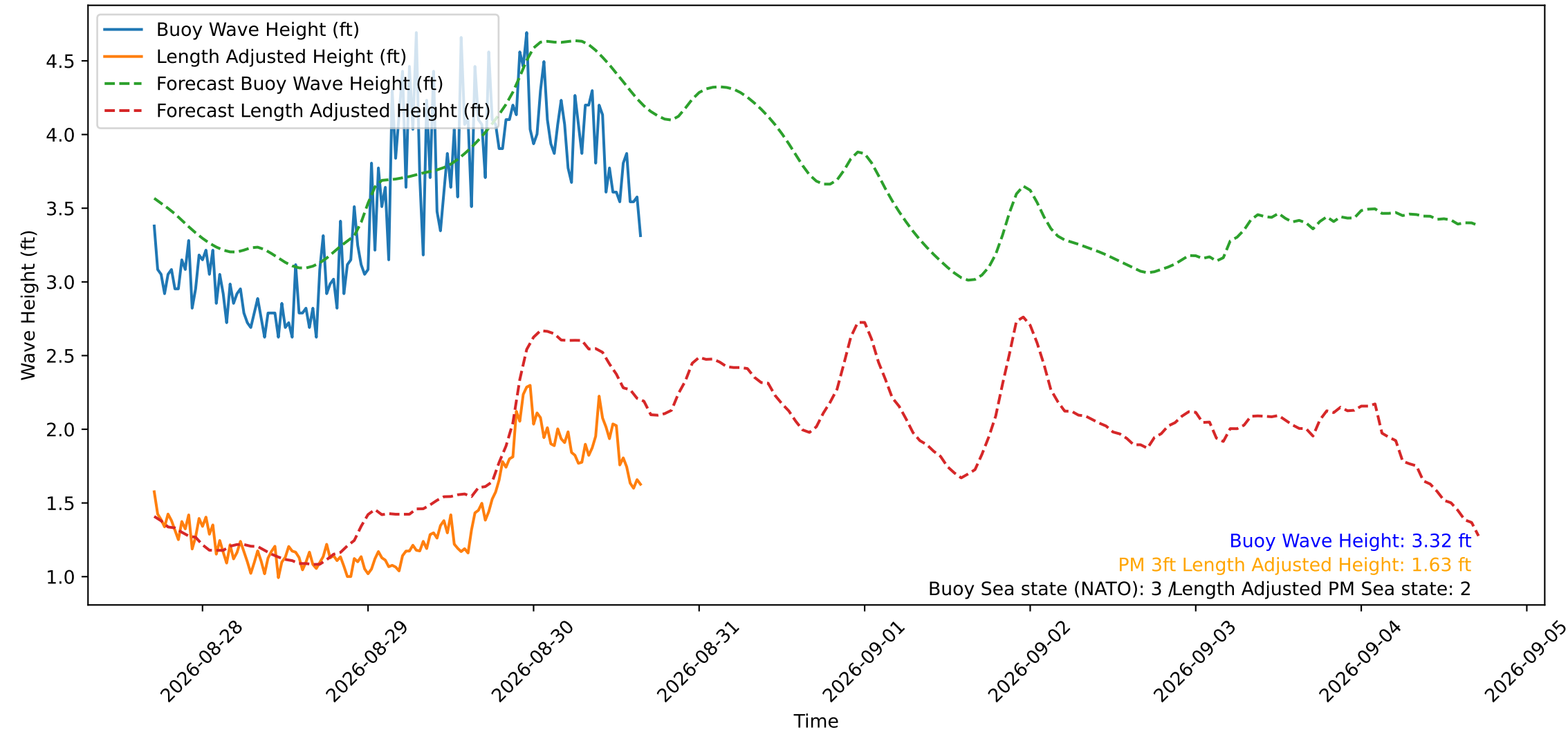
Wave Heights over Time for Red Beach at 2026-08-30 16:30:50
