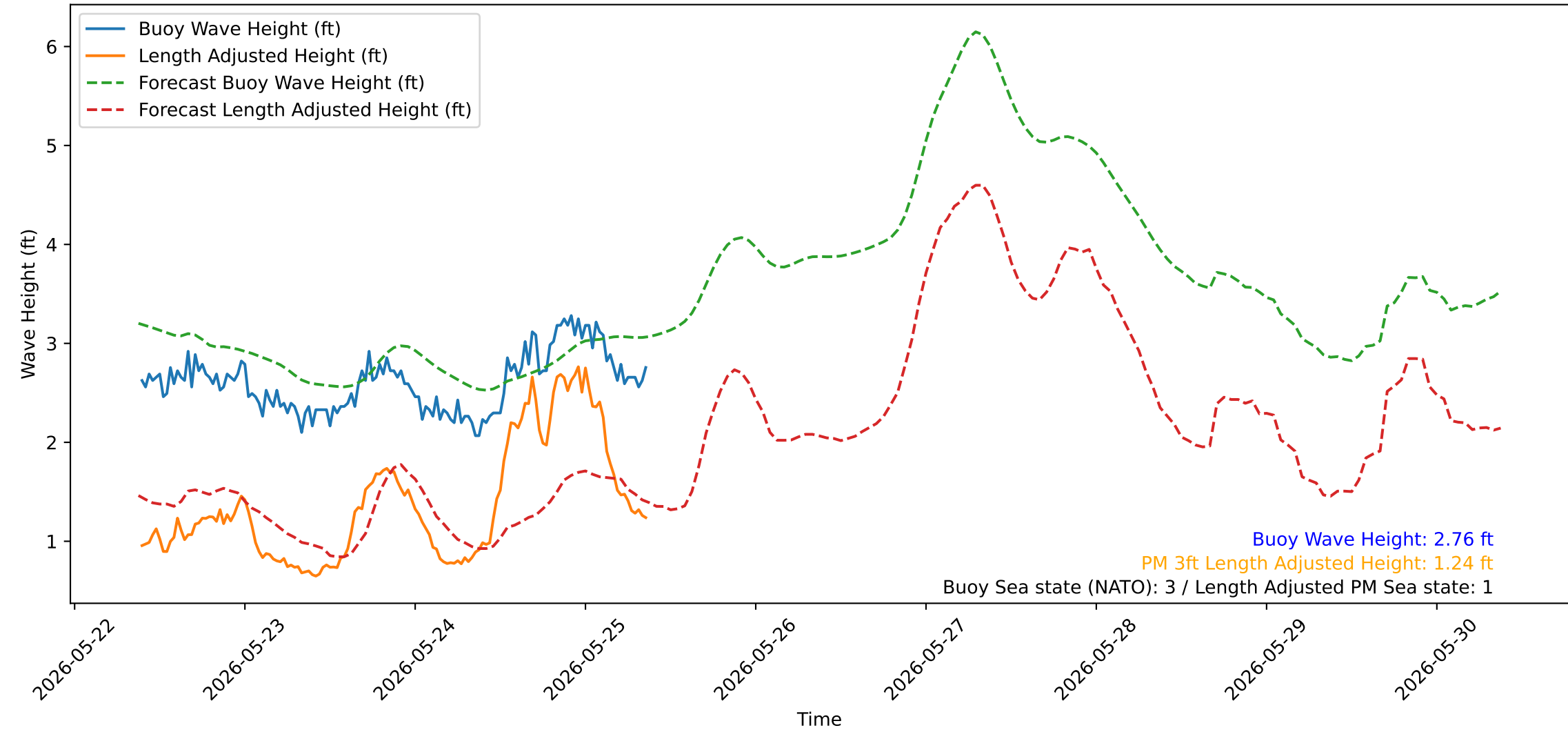
Wave Heights over Time for Green Beach at 2026-05-25 09:21:13
