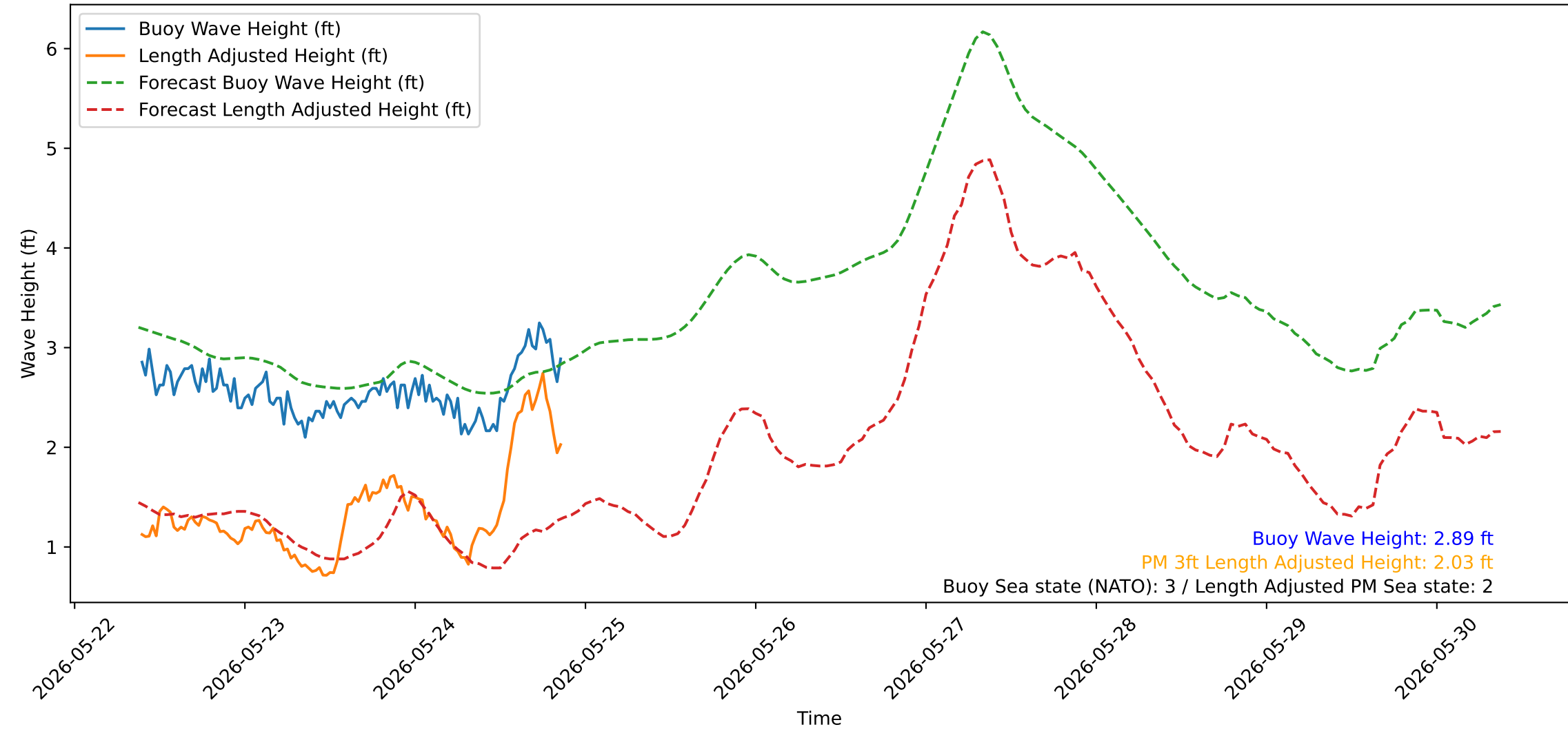
Wave Heights over Time for Oceanside Harbor at 2026-05-25 09:20:30
