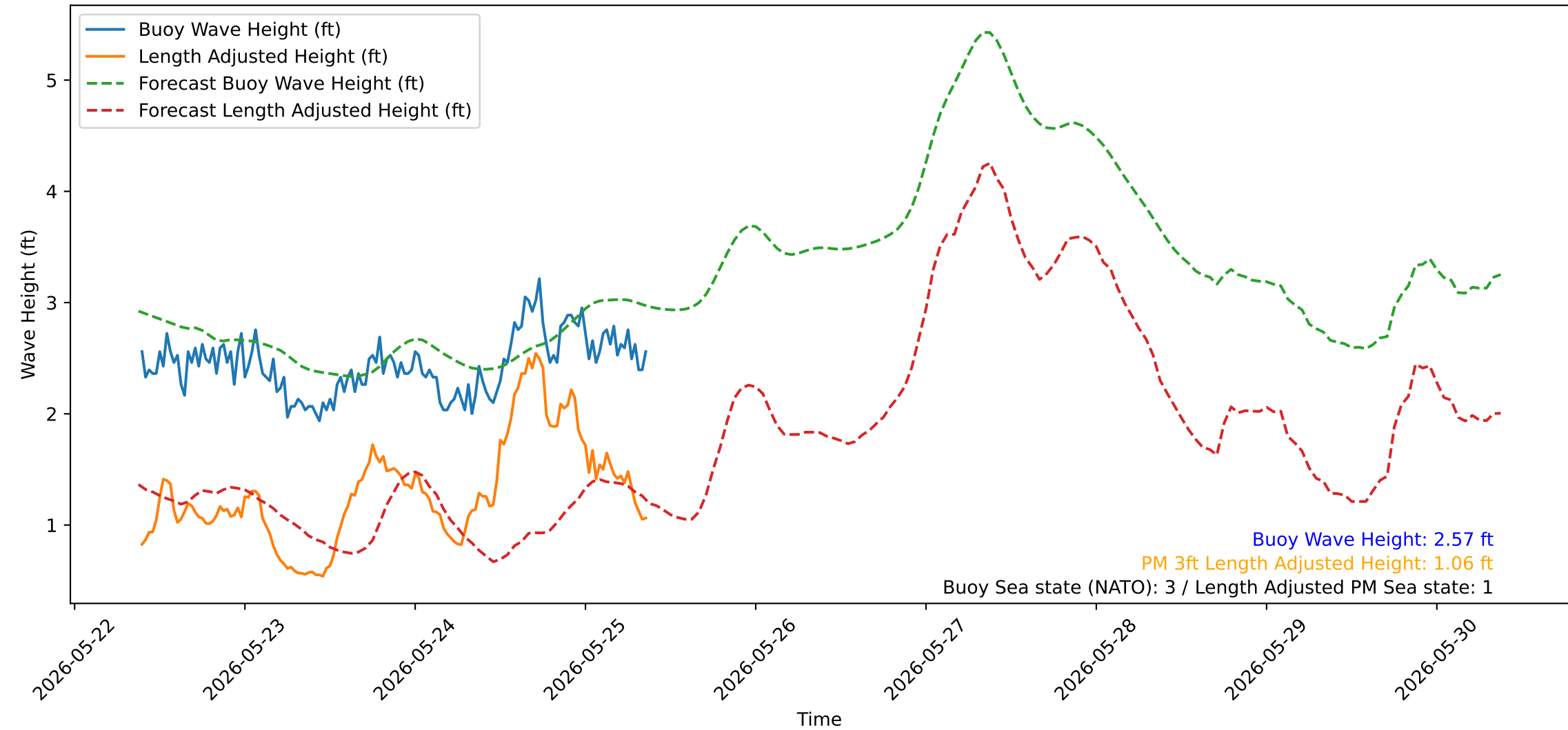
Wave Heights over Time for Red Beach at 2026-05-25 09:20:50
