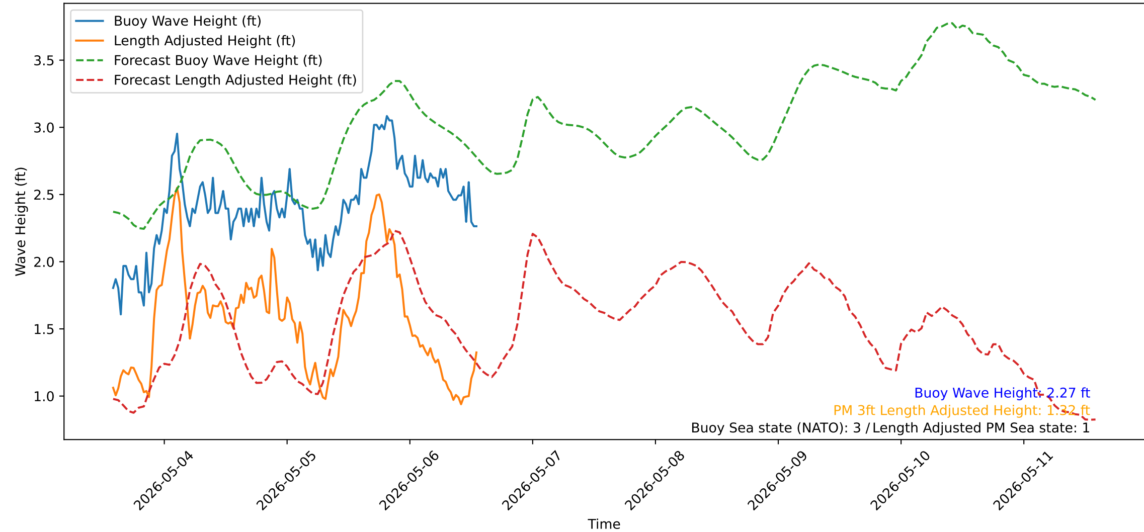
Wave Heights over Time for Red Beach at 2026-05-06 13:40:50
