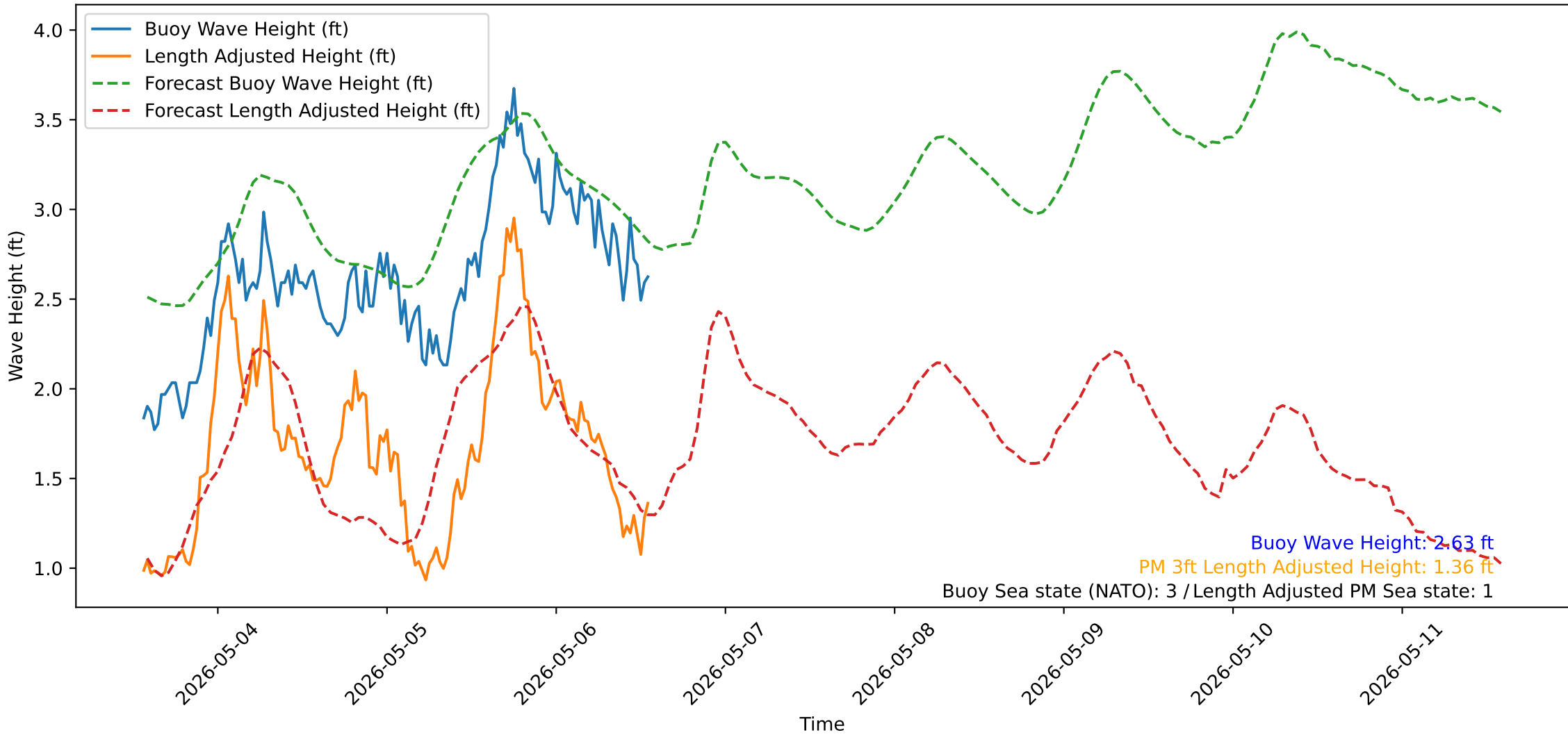
Wave Heights over Time for Green Beach at 2026-05-06 13:41:12
